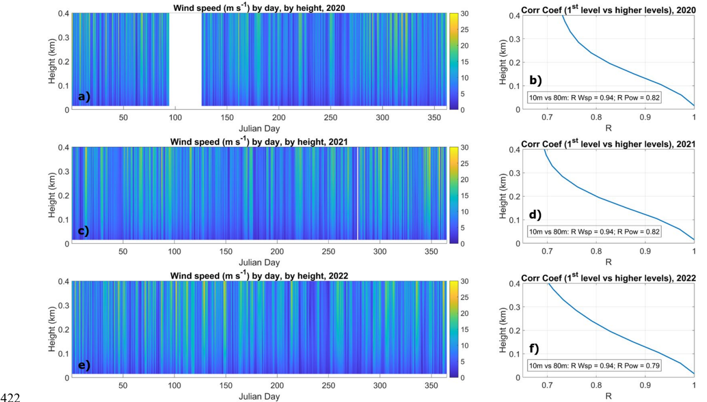
422 Figure A3: Time-height cross section of wind speeds by year (2020 in panel a, 2021 in panel c, and 2022 in panel e) at the SGP site. 423 Corresponding profiles of correlation coefficient values for wind speed between 10 m and the levels above are on the right panels 424 (2020 in panel b, 2021 in panel d, and 2022 in panel f). Note that during the 3 April–5 May 2020 period, the SGP site was shut down 425 due to the COVID-19 pandemic. 426
