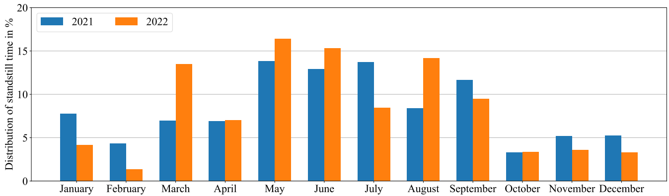
Figure 1. Distribution of calm wind periods in 2021 and 2022
