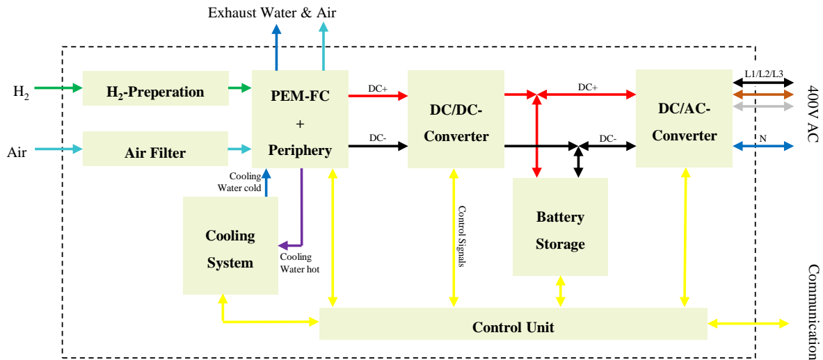
Figure 6. Structure of the fuel cell system
