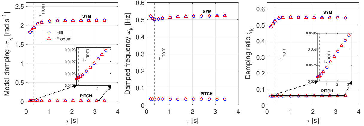
Figure 9. Modal damping, damped frequency and damping ratio for an eigenvalue analysis in the rotational frame with a time constant \tau variation.
