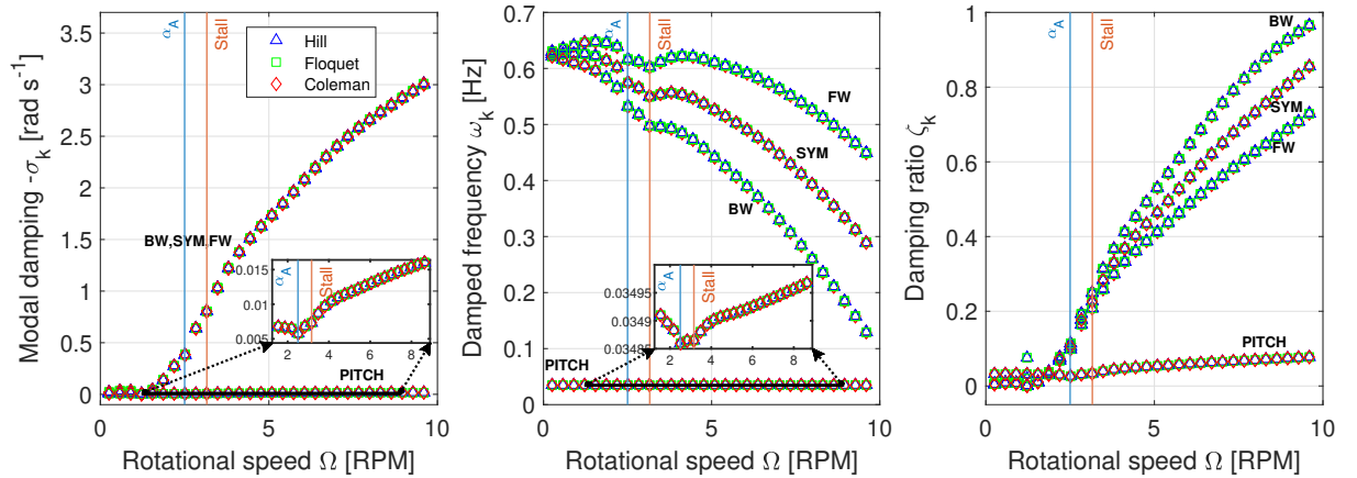
Figure 12. Modal damping, damped frequency and damping ratio for a Campbell diagram eigenvalue analysis in the NR frame with a rotational speed variation. The operational point is of V_0 = 8 \text{ m s}^{-1} .
