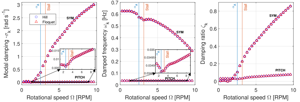
Figure 11. Modal damping, damped frequency and damping ratio for a Campbell diagram eigenvalue analysis in the rotational frame with a rotational speed variation. The operational point is of V_0 = 8 \text{ m s}^{-1} .
