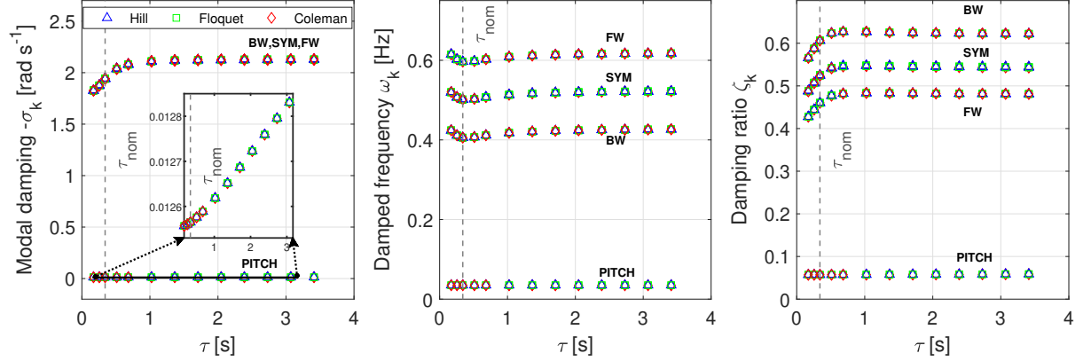
Figure 10. Modal damping, damped frequency and damping ratio for an eigenvalue analysis in the NR frame with a time constant \tau variation.
