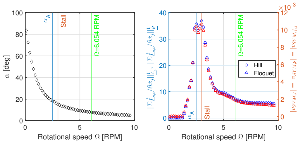
Figure 17. Angle of attack \alpha , 1-norm of the gradient \partial \underline{f}_{-s,i} / \partial \underline{\dot{x}}_j components, and dynamic stall component of the symmetric blade mode ( |v_{SYM,7}| ) for the LTI system matrix using Hill's and Floquet's method. The rotational speed \Omega is varied for the operational point of V_0 = 8 \text{ ms}^{-1} .
