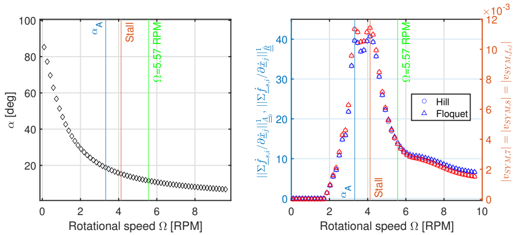
Figure 18. Angle of attack \alpha , 1-norm of the gradient \partial \dot{f}_{-s,i} / \partial \dot{x}_j components, and dynamic stall component of the symmetric blade mode ( |v_{SYM, f_s, l}| ) for the LTI system matrix using Hill's and Floquet's method. The rotational speed \Omega is varied for the operational point of V_0 = 10 \text{ m s}^{-1} .
