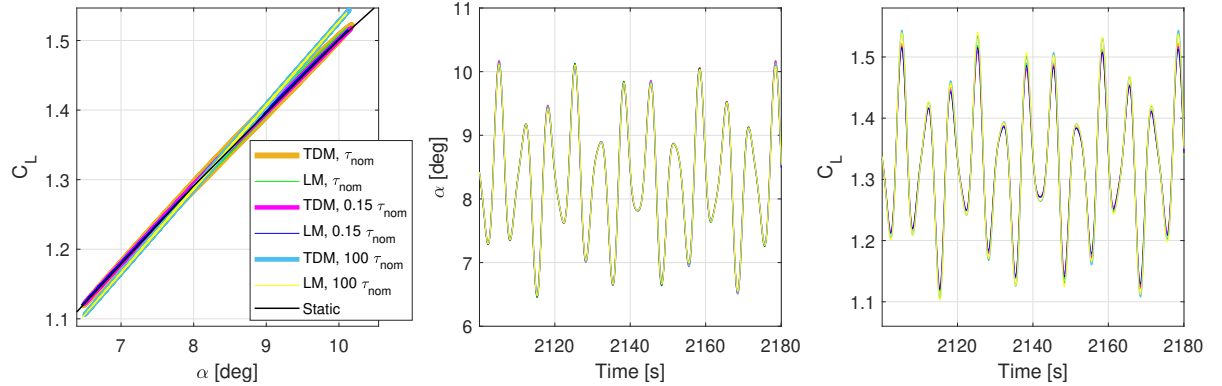
Figure 7. Hysteresis results for simulations with the operational point of V_0 = 8 \text{ m s}^{-1} and \Omega = 0.6 \text{ rad s}^{-1} , with a forcing moment applied on the floater pitch DOF, and where time domain model (TDM) and linear model (LM) results are compared.
