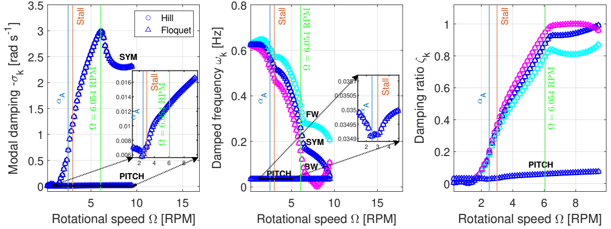
Figure 15. Modal damping, natural-damped frequency and damping ratio for a Campbell diagram eigenvalue analysis in the NR frame with a rotational speed variation. The operational point is of V_0 = 8 \text{ ms}^{-1} .
