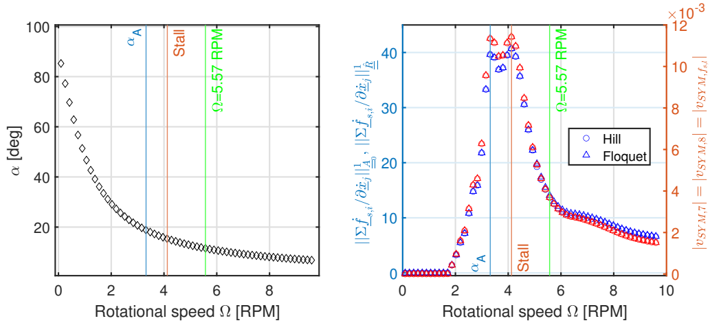
Figure 18. Angle of attack \alpha , 1-norm of the gradient \partial \dot{f}_{s,i} / \partial \dot{x}_j components, and dynamic stall component of the symmetric blade mode ( |v_{SYM, f_{s,i}}| ) for the LTI system matrix using Hill's and Floquet's method. The rotational speed \Omega is varied for the operational point of V_0 = 10 \text{ ms}^{-1} .
