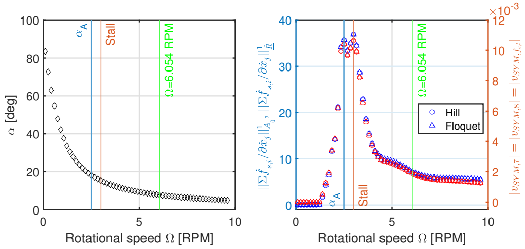
Figure 17. Angle of attack \alpha , 1-norm of the gradient \partial \dot{f}_{s,i} / \partial \dot{x}_j components, and dynamic stall component of the symmetric blade mode ( |v_{SYM, f_{s,i}}| ) for the LTI system matrix using Hill's and Floquet's method. The rotational speed \Omega is varied for the operational point of V_0 = 8 \text{ ms}^{-1} .
