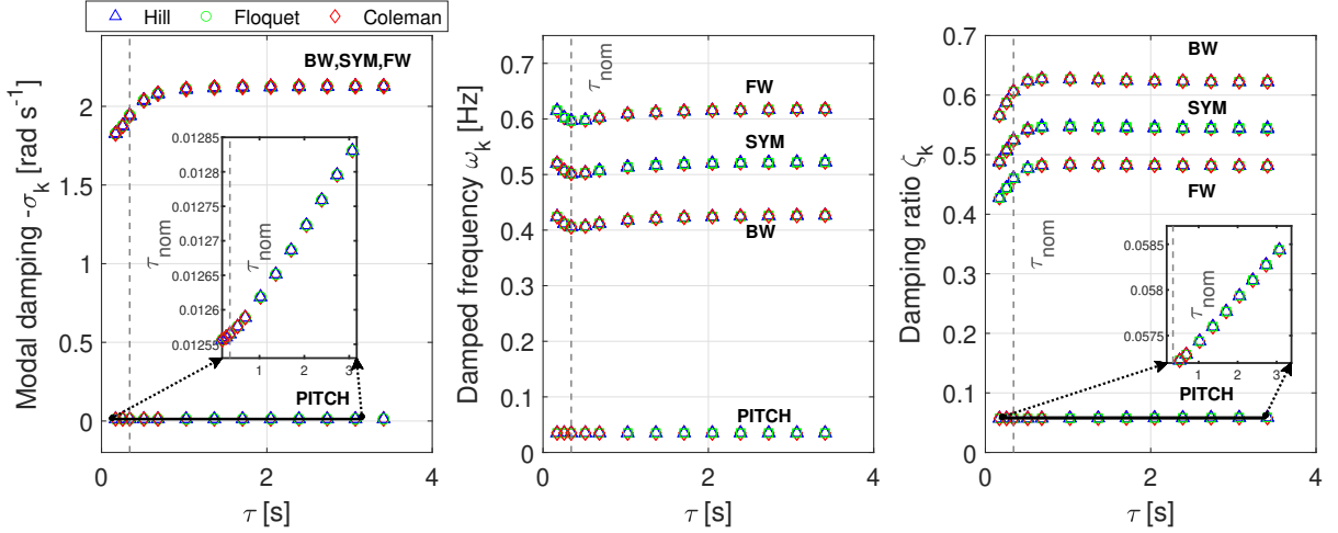
Figure 10. Modal damping, natural-damped frequency and damping ratio for an eigenvalue analysis in the NR frame with a time constant \tau variation.
