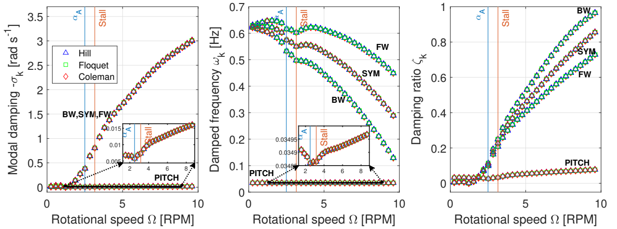
Figure 12. Modal damping, natural-damped frequency and damping ratio for a Campbell diagram eigenvalue analysis in the NR frame with a rotational speed variation. The operational point is of V_0 = 8 \text{ ms}^{-1} .
