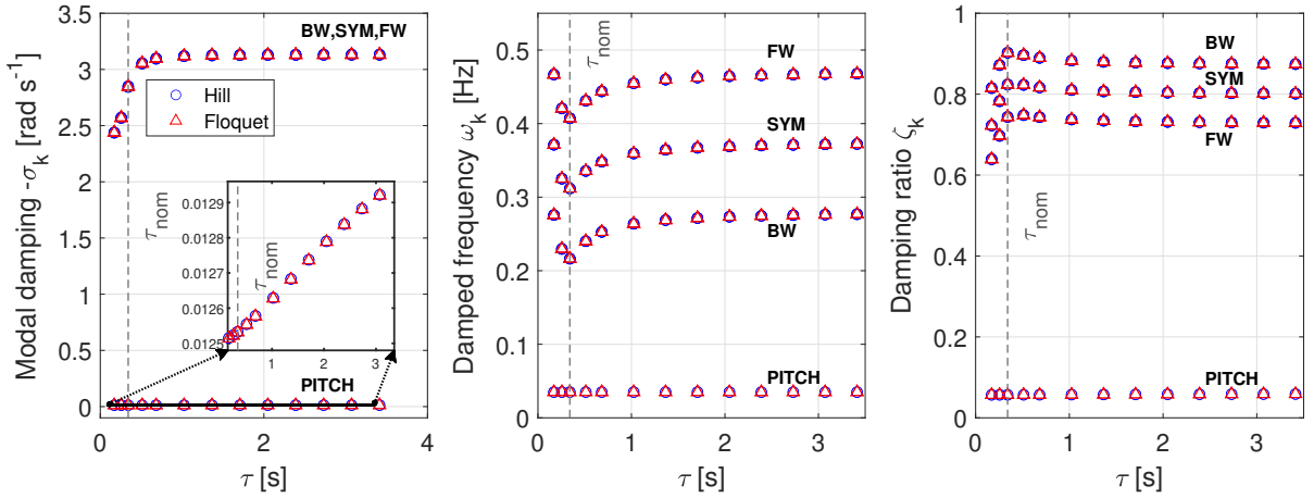
Figure 14. Modal damping, natural-damped frequency and damping ratio for an eigenvalue analysis in the NR frame with a time constant \tau variation.
