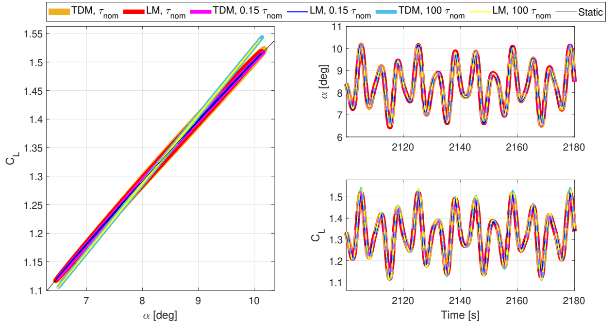
Figure 7. Hysteresis results for simulations with the operational point of V_0 = 8 ms -1 and \Omega = 0.6 rad s -1 in the inviscid region, with a forcing moment applied on the floater pitch DOF, and where time domain model (TDM) and linear model (LM) results are compared.
