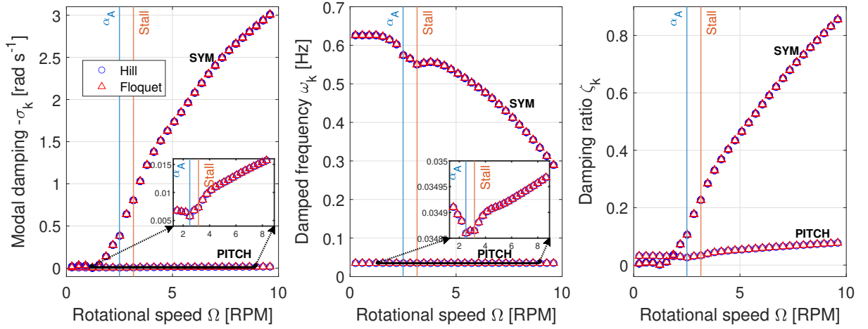
Figure 11. Modal damping, natural-damped frequency and damping ratio for a Campbell diagram eigenvalue analysis in the rotational frame with a rotational speed variation. The operational point is of V_0 = 8 \text{ ms}^{-1} .
