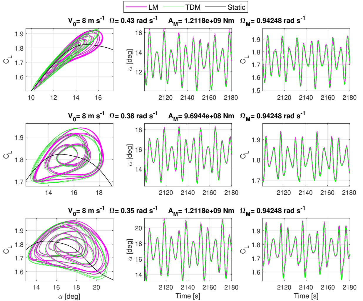
Figure 6. Dynamic lift and stall behaviour behavior at three different operational points surrounding the stall maximal static lift coefficient C_{L,static} region, with a varying forcing moment applied on the floater pitch DOF, and where the time domain model (TDM) and linear model (LM) results are compared.
