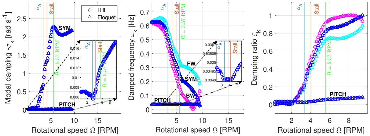
Figure 16. Modal damping, natural-damped frequency and damping ratio for a Campbell diagram eigenvalue analysis in the NR frame with a rotational speed variation. The operational point is of V_0 = 10 \text{ ms}^{-1} .
