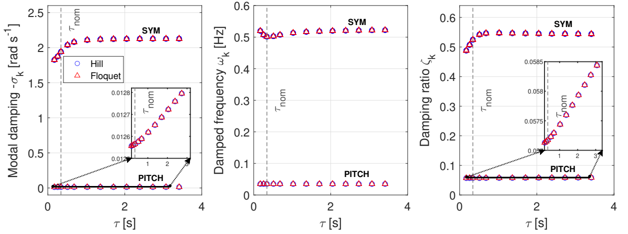
Figure 9. Modal damping, natural damped frequency and damping ratio for an eigenvalue analysis in the rotational frame with a time constant \tau variation.
