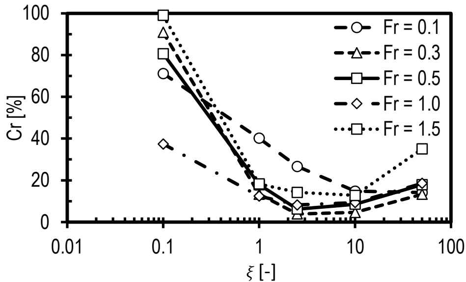
Figure 7. Reflection coefficient as a function of \xi for a range of Froude numbers.
