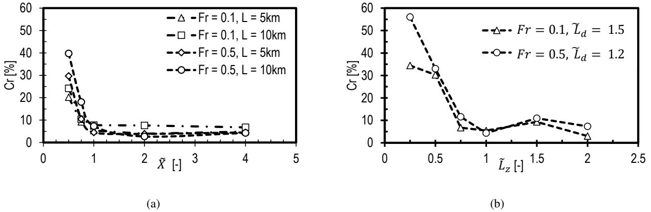
Figure 9. Reflection coefficient for the hill case as a function of: (a) domain length for Fr = 0.1 and Fr = 0.5 for L = 5 km and 10 km; and (b) domain height for Fr = 0.1, \tilde{L}_d = 1.5 and Fr = 0.5, \tilde{L}_d = 1.2 .
