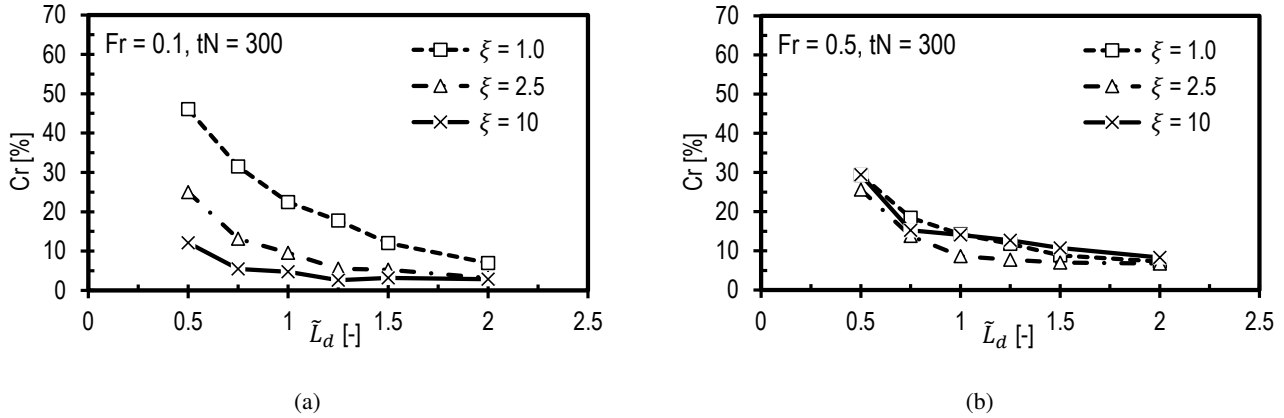
Figure 10. Reflection coefficient for the wind farm canopy case as a function of normalised damping layer thickness for different values of the damping coefficient when (a) Fr = 0.1 and (b) Fr = 0.5 .
