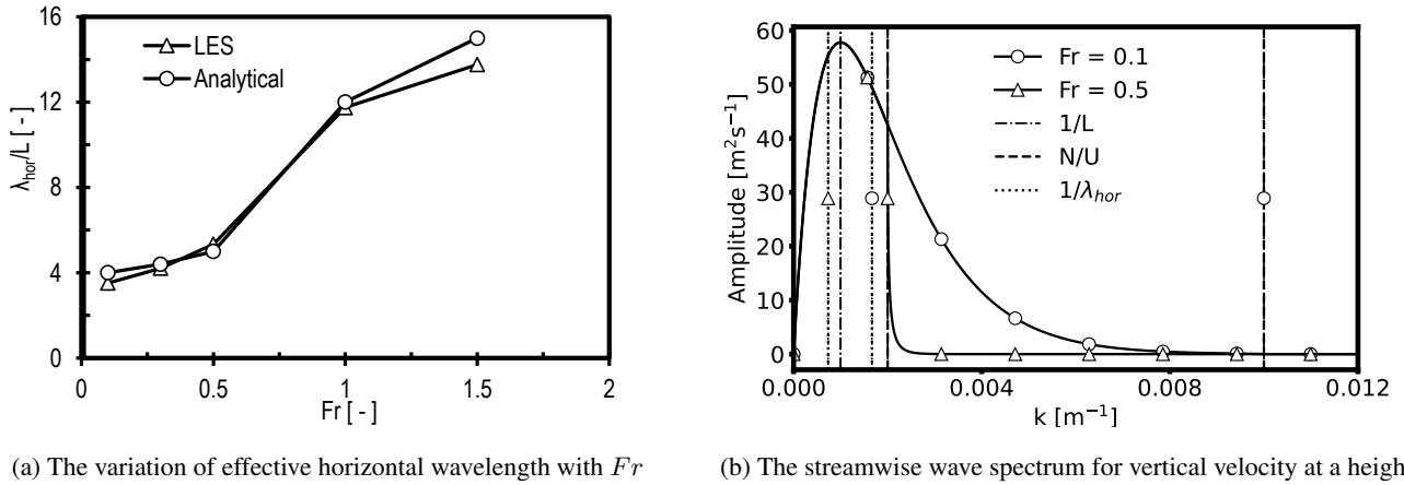
Figure 3. (a) Effective horizontal wavelength as a function of Fr , and (b) effective, dominant and buoyancy wavelengths identified for Fr = 0.1 and 0.5 .
