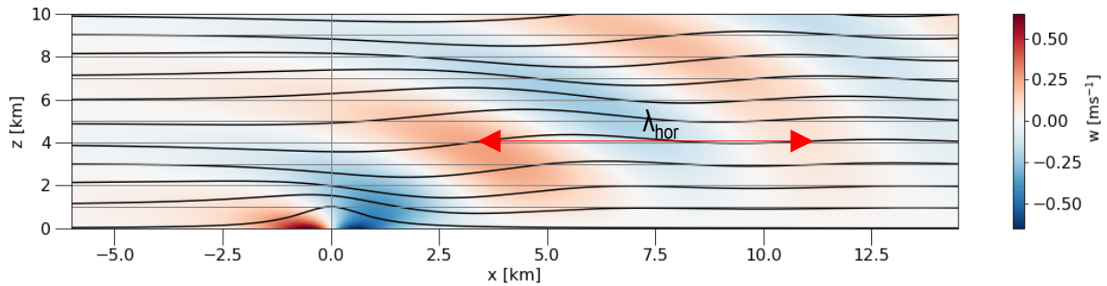
Figure 2. Steady-state analytical solution of flow over a WOA hill centered at x = 0\text{ km} . The color contours represent vertical velocity and the streamlines show the propagation of the waves. Allaerts (2022)
