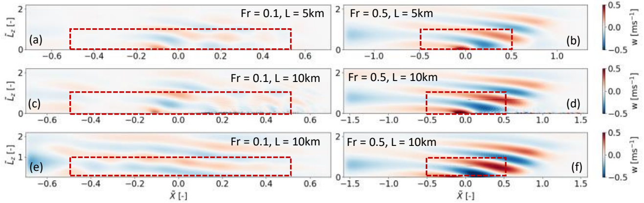
Figure 11. Plots (a-d) show vertical velocity of flow through and around the wind farm canopy with lengths L = 5 and 10 km for Fr = 0.1 and 0.5 , and \tilde{X} = 1.0 . For comparison, the plots (e-f) show the corresponding hill cases where L = 10 km for Fr = 0.1 and 0.5 , and \tilde{X} = 1.0 . The region inside the dashed red box is the non-damped domain.
