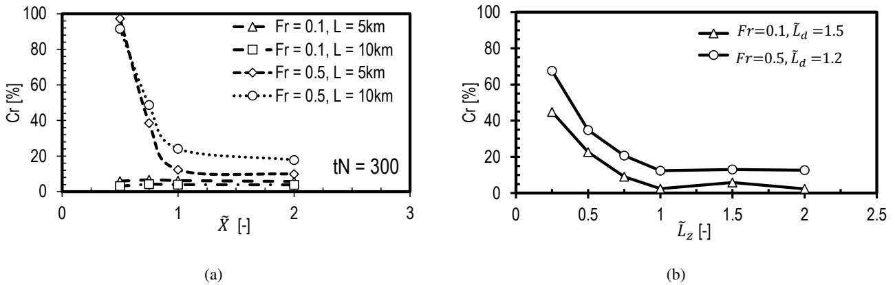
Figure 12. Reflection coefficient for the wind farm canopy case as a function of: (a) domain length for Fr = 0.1 and Fr = 0.5 for L = 5 km and 10 km; and (b) domain height for Fr = 0.1, \tilde{L}_d = 1.5 and Fr = 0.5, \tilde{L}_d = 1.2 .
