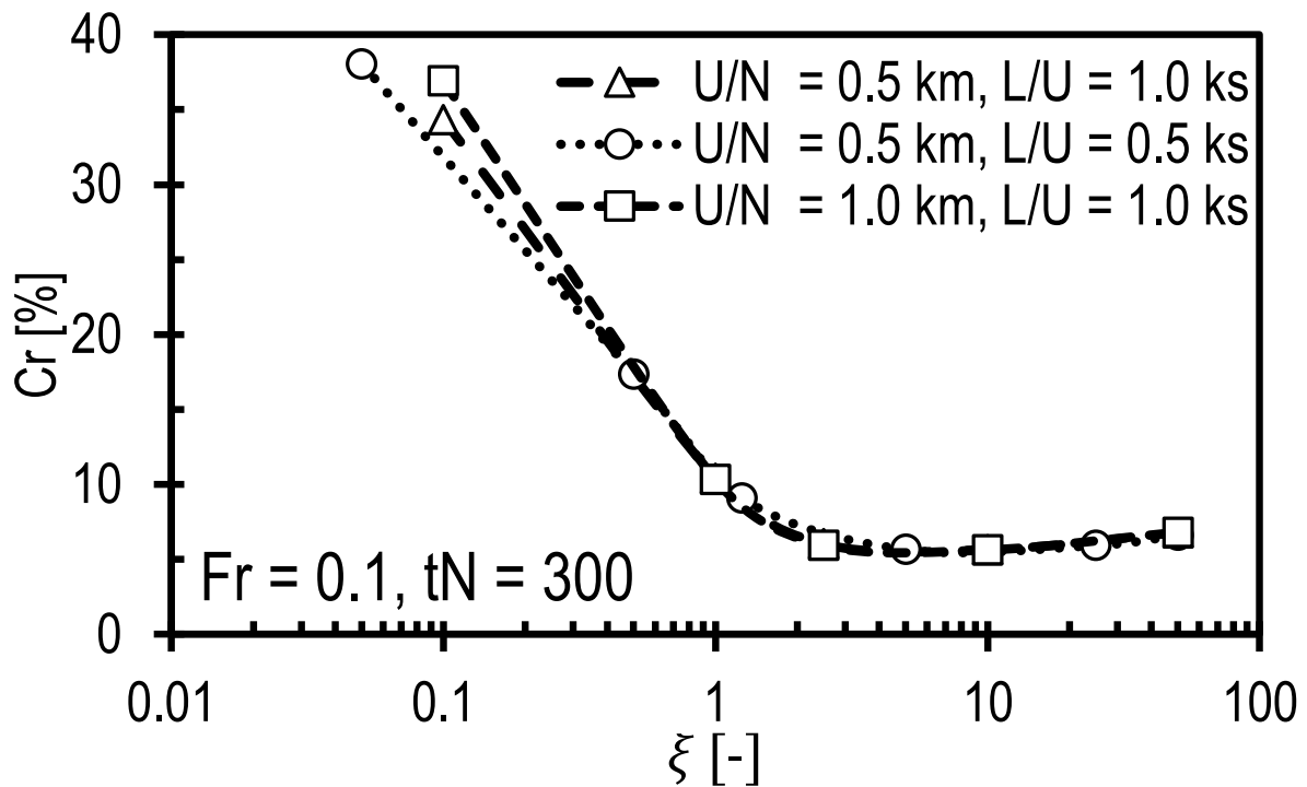
Figure 5. Reflection coefficient as a function of normalised damping coefficient \xi for varying length and time scales.
