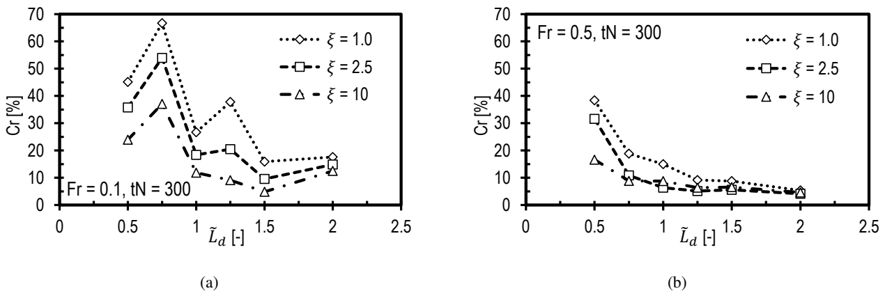
Figure 8. Reflection coefficient for the hill case as a function of normalised damping layer thickness for different values of the damping coefficient when (a) Fr = 0.1 and (b) Fr = 0.5 .
