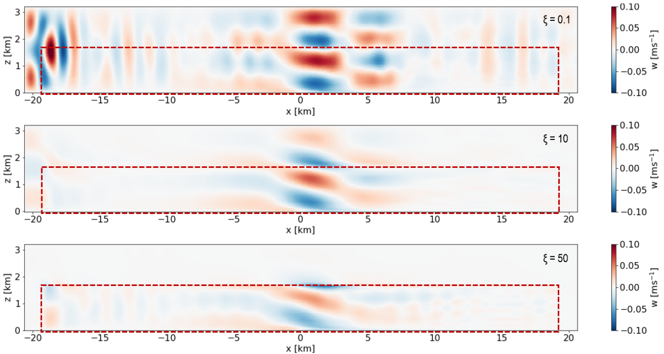
Figure 6. Contours of vertical velocity in a streamwise-oriented vertical plane at tN 300 for Fr = 0.1 with \xi = 0.1 (top), \xi = 10 (middle), and \xi = 50 (bottom). The red box shows the non-damped domain, and everything outside is the RDL.
