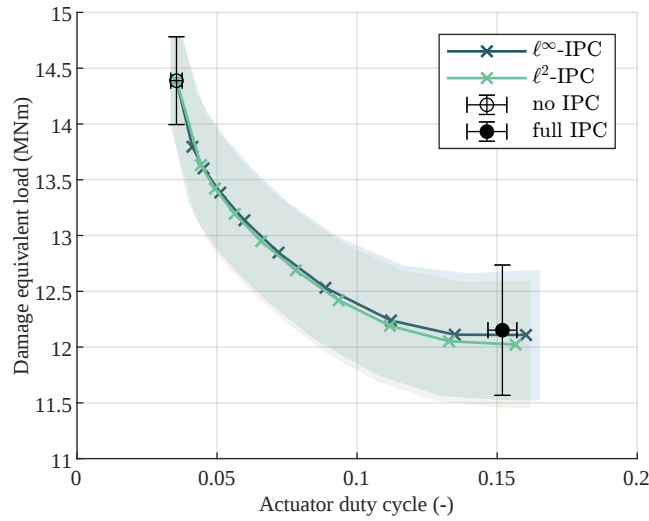
Figure 17. The trade-off between DEL and ADC when operating between no IPC and full IPC with 8.0 % turbulence. The \ell^\infty -IPC and \ell^2 -IPC control methods use a change in reference load while the full between 10 MNm (corresponding to no IPC uses a grid search of integrator gains) and 0 MNm (corresponding to achieve full IPC). The error bars (for no and full IPC) and the trade-off in DEL shaded region (for \ell^\infty -IPC and \ell^2 -IPC) represent the standard deviation (1-sigma) from the mean. The output-constrained IPC methods have a nonlinear trade-off and achieve an 87% of the reduction in DEL at just 50% of the increase in ADC compared to the full IPC controller with the same crossover frequency (0.2 rad/s).
