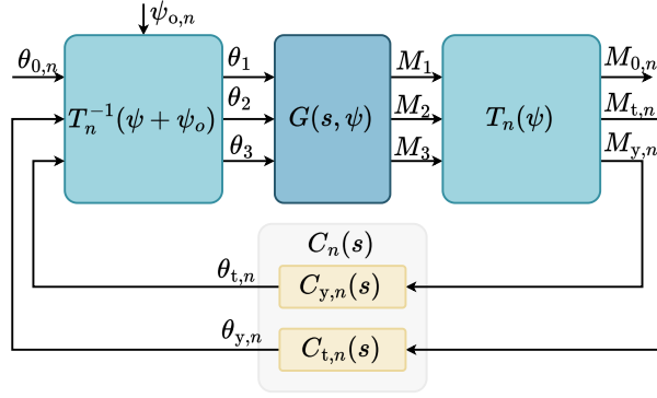
Figure 1. Block diagram of conventional -full IPC for the nP blade harmonic, fully attenuating the tilt and yaw moments. The forward MBC transformation \mathbf{T}_n transforms the rotating blade loads to the nonrotating frame, where the SISO controllers C_{t,n} and C_{y,n} fully attenuate the tilt and yaw moments. The inverse MBC transformation \mathbf{T}_n^{-1} converts the pitch signals back to the rotating frame and includes an azimuth offset \psi_{o,n} to decouple the tilt and yaw axes.
