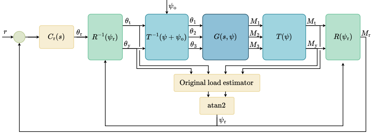
Figure 10. Block diagram of \ell^2 -IPC. The original-open-loop load estimator uses the nonrotating loads and nonrotating pitch angles to reconstruct the original-open-loop load. The angle of this load in the tilt-yaw plane is \psi_r , which is used to rotate the reference system to a radial and tangential axis where the magnitude of the nonrotating load vector is projected on the radial axis. A single SISO controller then regulates this load magnitude.
