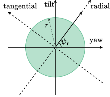
Figure 9. Using \ell^2 -IPC, the nonrotating load vector is projected on a new orthogonal reference system, consisting of a radial and tangential axis. In this new axes system, the magnitude of the load is projected on the radial axis. The load is thus constrained using the 2-norm, indicated by a circle.
