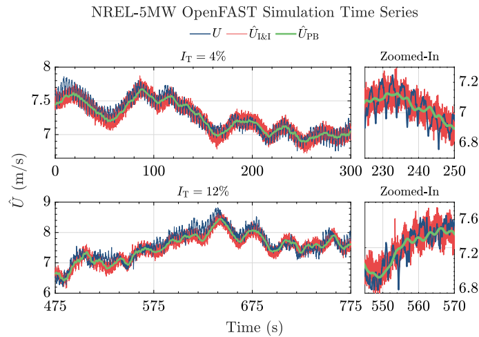
Figure 14. Wind speed estimation time series for the NREL-5MW wind turbine. The proposed method (blue-green line) gives a smooth, less noisy estimate compared to the I&I (green-red) for low (top plots) and high (bottom plots) turbulent cases. The low-frequency component of the wind speed is captured where biased estimation occasionally occurs, potentially due to an inaccurate C_p table utilized in both estimators and an absence of dynamic inflow modeling in the estimators. The actual REWS, as outputted by OpenFAST, is shown in-by the gray-blue line. Zoomed-in plots of 25-s time spans are provided on the right for clearer observation of the
