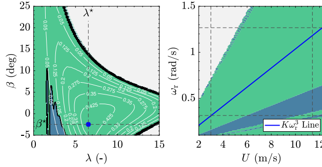
Figure 9. Stability region of the continuous wind speed estimate solver in the continuous time \mathcal{G}(s) , where the condition p < 0 in (29) is satisfied (indicated in green, otherwise in blue). The left subfigure shows the different C_p levels for the NREL-5MW turbine (white solid lines), with C_p^* indicated by the blue dot. The right subfigure shows the mapping of the stability region in terms of wind speed U and rotor speed \omega_r for the fine pitch angle \beta^* . The solid blue line is the partial-load regime, where the K\omega_r^3 controller is active. Also shown for completeness are the black dashed lines, indicating the lower and upper bounds for the rotor speed, as well as cut-in and rated wind speeds.
