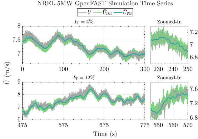
Figure 14. Wind speed estimation time series for the NREL-5MW wind turbine. The proposed method (blue line) gives a smooth, less noisy estimate compared to the I&I (green line) for low (top plots) and high (bottom plots) turbulent cases. The low-frequency component of the wind speed is captured where biased estimation occasionally occurs, potentially due to an inaccurate C_p table utilized in both estimators and an absence of dynamic inflow modeling in the estimators. The actual REWS, as outputted by OpenFAST, is shown in the gray line. Zoomed-in plots of 25-s time spans are provided on the right for clearer observation of the estimation performance.
