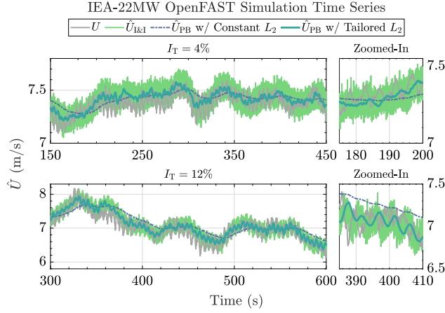
Figure 15. Wind speed estimation time series for the IEA-22MW wind turbine. The proposed method gives a smooth, less noisy estimate compared to the I&I (green line) for low (top plots) and high (bottom plots) turbulent cases. Constant L_2 (dashed dark blue line) results in lagged estimation compared to gain-tailored L_2 (solid blue line). The actual REWS, as outputted by OpenFAST, is shown in the gray line. Zoomed-in plots of 25-s time spans are provided on the right for clearer observation of the estimation performance.
