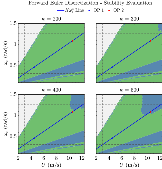
Figure 10. Unstable region (blue area) growth of \mathbf{H}_{FE}(z) with increasing \kappa = \{200, 300, 400, 500\} using h = 1/50 s of sampling time and the Forward Euler discretization method.
