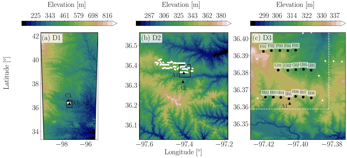
Figure 2. Horizontal extent and terrain elevation maps associated with the WRF simulations domains -mesoscale domain D1 (a) and LES domains D2 (b) and D3 (c). The King Plains wind farm consists of 88 turbines (white dots), from which a subset of 17 wind turbines was represented in the simulation (black dots). Within domain D3, some turbines near boundaries were removed (white dots). Inflow fetches of 2 and 1 km in the southerly and easterly boundaries, respectively, were removed from the analyses (white dashed lines). The observation sites A1, A2 and C1 (black triangles) are also shown.
