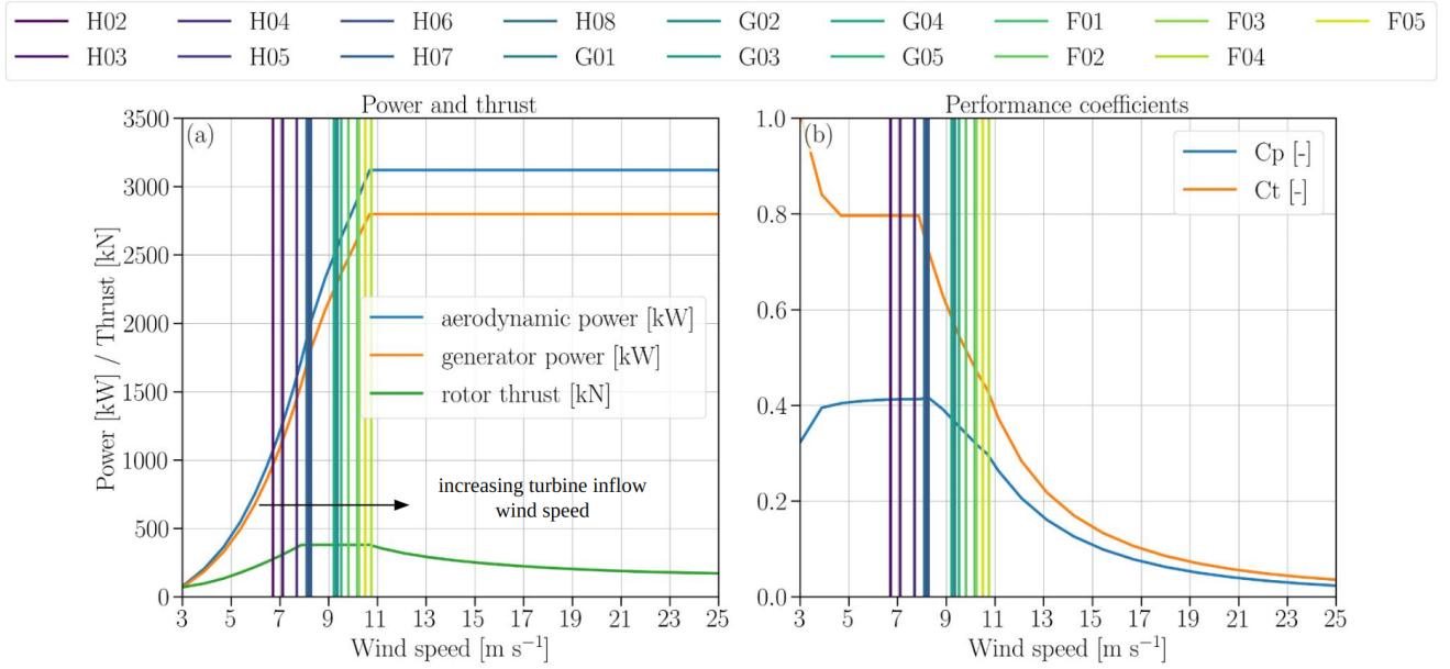
Figure C1. AerodynamicTheoretical aerodynamic, generator power, and rotor thrust curves for the NREL 2.82 MW turbine (Quon, 2022) used in the simulations (a). The power ( C_p ) and thrust ( C_t ) coefficient curves (b). The mean wind speed at hub height upstream of the turbines is calculated for the simulation with turbines and is shown as vertical lines.
