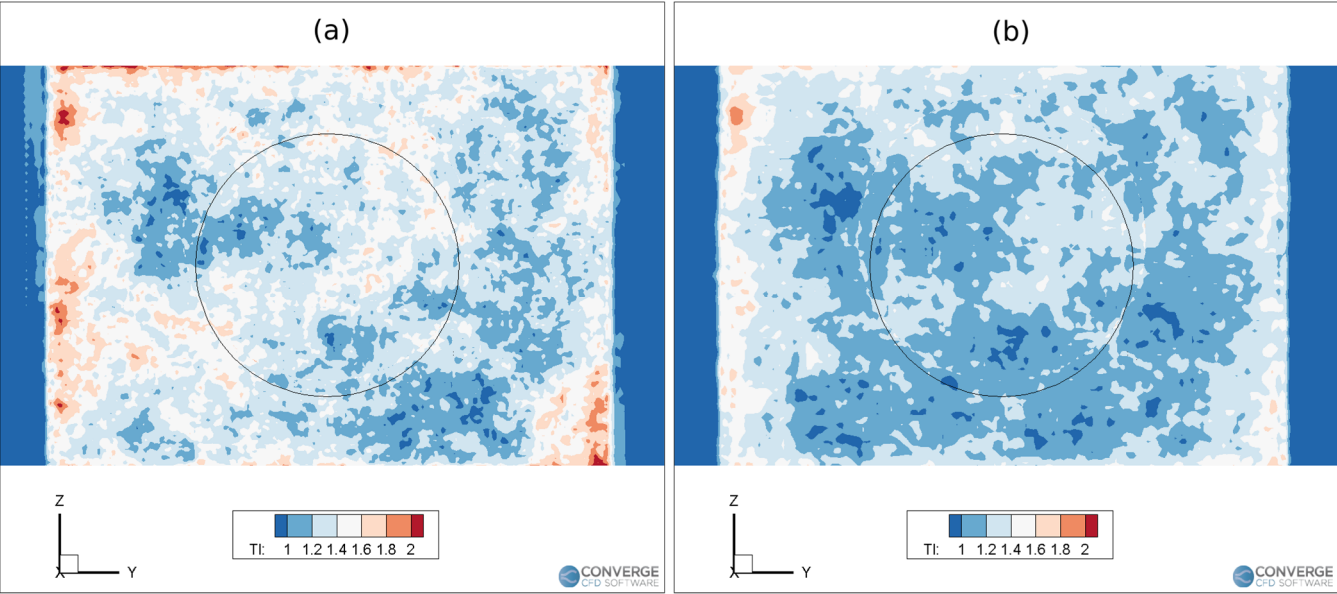
Figure A2: Turbulence intensity ( TI = stg(U - \bar{U})/\bar{U} ) at the rotor plane in preliminary empty-box simulations without the rotor. (a) LES simulations, (b) URANS-STG simulations. The average turbulence intensity on the rotor disk is 1.35% for the LES simulation and 1.2% for the URANS-STG approach.
