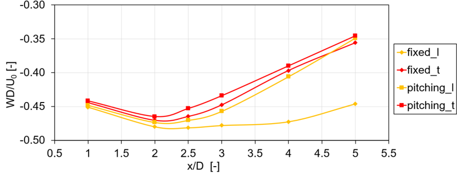
460 Figure 11: Along wake profile of normalized integral Wake Deficit, comparison between results with fixed platform and laminar (F-L) or turbulent inflow (F-T) and the ones with pitching platform and laminar (P-L) or turbulent inflow (P-T).
