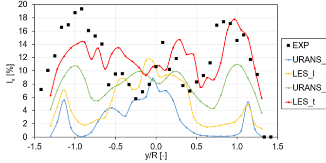
560 Figure 17: Fixed case, streamwise turbulence intensity of the wake at 3D from the rotor, horizontal traverse; comparisons with experiments (EXP).
