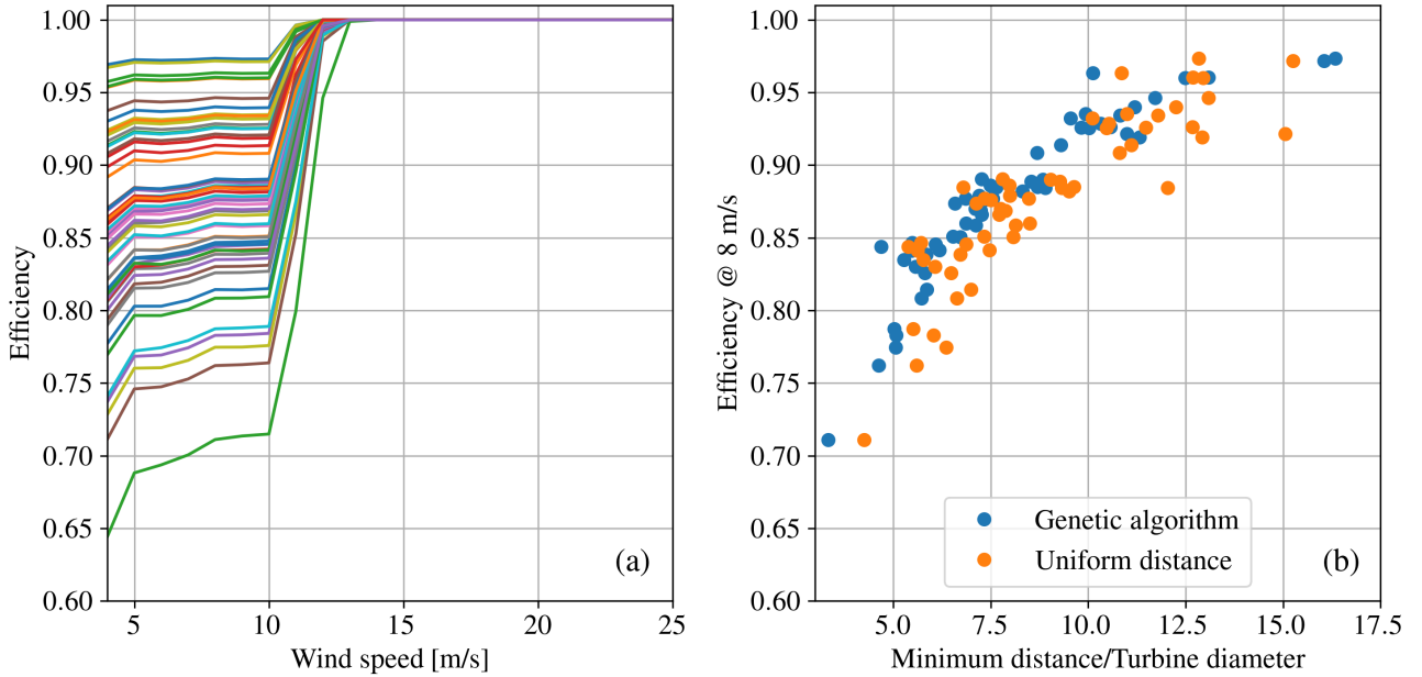
Figure 11. Array efficiency for all the considered wind farms. (a) Azimuthal-average of the array efficiency. (b) Efficiency at 8 m/s plotted against L_{\text{opt}} or L normalised by the turbine diameter.
