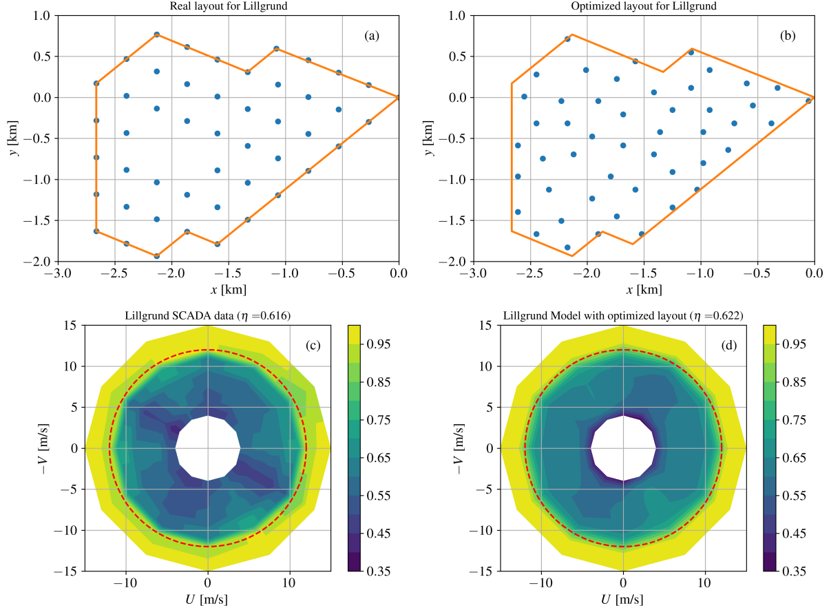
Figure 12. Validation of the optimization method for the Lillgrund wind farm. (a,b) layout of the farm, (c,d) array efficiency for different wind velocities and directions (the red dashed line indicates the rated speed of the installed Siemens wind turbine, 12 m/s). (a,c) real Lillgrund data (Sebastiani et al., 2021) (b,d) analysis of the optimized layout with the minimum distance fitness function. The title of the bottom row reports the average array efficiency of the farm for velocity below rated speed.
