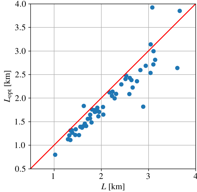
Figure 10. Minimum intra-turbine distance from the genetic algorithm, L_{\text{opt}} , plotted against the uniform distance estimate, L .
