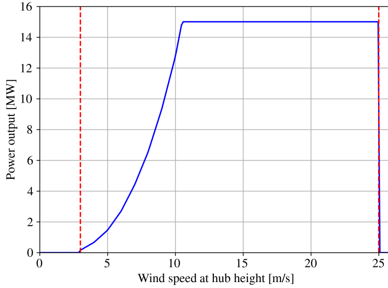
Figure 4. Power curve of the IEA 15 MW turbine. The characteristics wind speeds of cut-in and cut-out are marked with red dashes in the figure.
