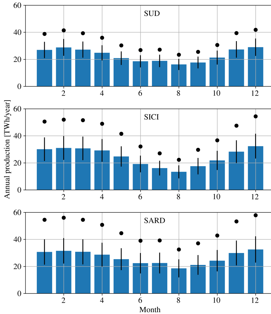
Figure 14. Annual power production in the three most producing Italian zones, i.e. SUD, SICI and SARD sorted for each month of the year. (Black circles) power production when all farms are approved. (Blue bars with error bars) expected value of the power production with the associated standard deviation.
