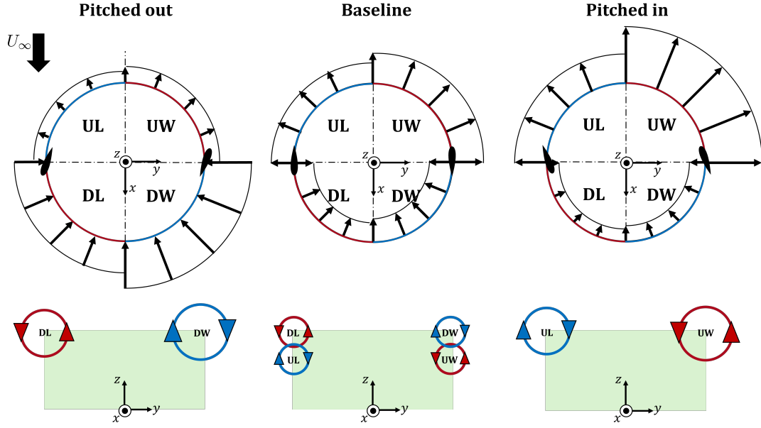
Figure 1. Top view schematic of the simplified AC force fields for the three "vortex generator" modes of operations adapted from Huang et al. (2023a); Bensason et al. (2024), namely the baseline case (where no pitch is applied), a pitched in case, and pitched out. Blades at a phase position of \theta = 0^\circ are shown at exaggerated sizes and pitch angles to demonstrate the pitching convention. The coordinate systems are shown at the center of the AC, and the rotation direction is anti-clockwise. The quadrants of the idealized AC are labeled as upwind windward UW 0^\circ < \theta < 90^\circ , upwind leeward UL 90^\circ < \theta < 180^\circ , downwind leeward DL 180^\circ < \theta < 270^\circ , and downwind windward DW 270^\circ < \theta < 360^\circ . The top edges of the rotor cylinder are color-coded based on the direction of rotation in the internal frame of reference of the trailing blade-tip vortices, with red and blue as counter-clockwise and clockwise, respectively. The top half of the rotor's projected frontal area (green) at a generic measurement plane downstream is shown below each mode. The projected dominant quadrant-labeled streamwise vortical structures stemming from the blade tips for each pitch case are shown via circular arrows.
