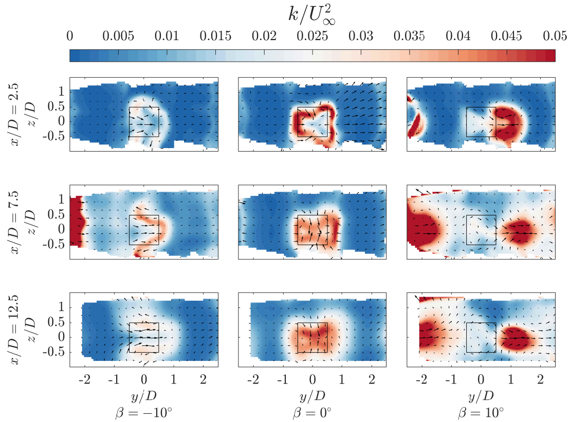
Figure C1. Normalized turbulent kinetic energy k = \frac{1}{2}((U'_x)^2 + (U'_y)^2 + (U'_z)^2) for the three pitch cases at stream-wise locations x/D = 2.5, 7.5, \text{ and } 12.5 . The black outlined square denotes the projected frontal area of the rotor, and the vectors show the in-plane velocity components.
