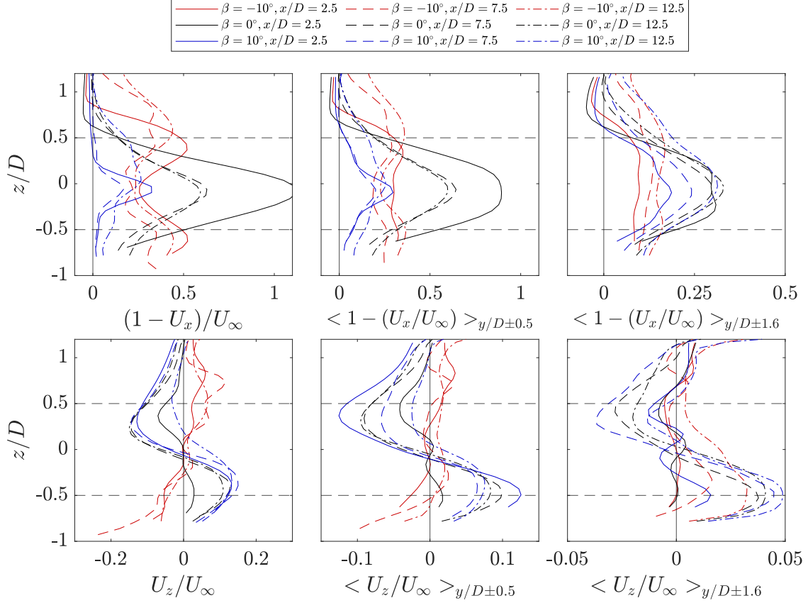
Figure 13. Normalized streamwise deficit 1 - (U_x/U_\infty) and axial U_z/U_\infty velocity profiles at discrete cross-stream measurement planes x/D = 2.5, 7.5, and 12.5 for the vortex generator and baseline modes of operations. (Left column) the normalized velocity profiles about the y/D = 0 symmetry plane. (Middle column) lateral-averaged streamwise velocity profiles within the projected frontal area of the rotor -0.5 \leq y/D \leq 0.5 . (Right column) lateral-averaged velocity profiles within lateral domain -1.6 \leq y/D \leq 1.6 . The horizontal dashed lines indicate the upper and lower bounds of the rotor projected frontal area.
