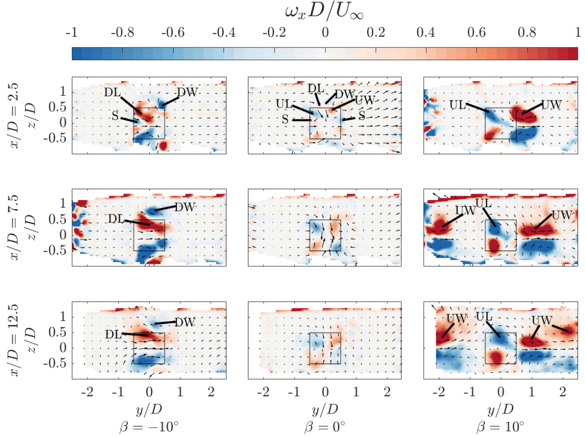
Figure 8. Normalized streamwise vorticity at \omega_x D / U_\infty for the three pitch cases at streamwise locations x/D = 2.5, 7.5 , and 12.5 . The black outlined square indicates the projected frontal area of the rotors, and the vectors show the in-plane velocity components. The streamwise vortical structures generated by each AC load quadrant are labeled, as described in Section 2. The label S corresponds to structures generated at the interface between the struts and blade.
