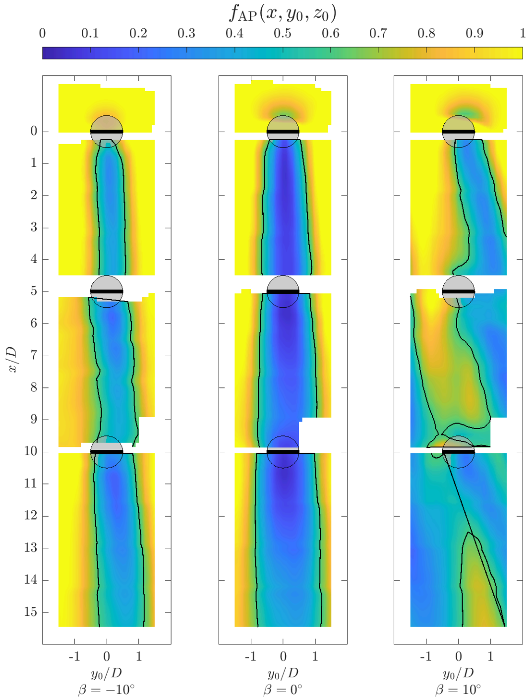
Figure 15. Available power as calculated using Equation 5 for the three pitch cases over all streamwise distances x/D and lateral offsets y_0/D ranging from -1.5 to 1.5. The gray areas indicate the top-view areas of the rotor and the idealized actuator surface. The black contour lines show where f_{AP} = 0.7 , i.e., 70% of the maximum available power provided by the streamwise flow.
