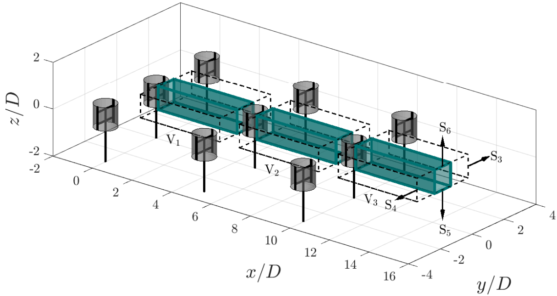
Figure 17. Schematic of the wind farm control volumes, denoted as V_1 , V_2 , and V_3 , corresponding to the flow behind the first, second, and third rotor of the central column, respectively. The shaded regions are the volumes within the projected areas of the rotors of the central column ( -0.5 \leq y/D \leq 0.5 ), while the dashed black lines indicate the edges of the central cells of the farm grid ( -1.6 \leq y/D \leq 1.6 ). The fluxes are evaluated through the lateral and axial surfaces S_3 , S_4 , S_5 , and S_6 , respectively. The gray shaded cylinder indicates the idealized AC surface of the rotors, which are shown at a phase-locked position of \theta = 0^\circ .
