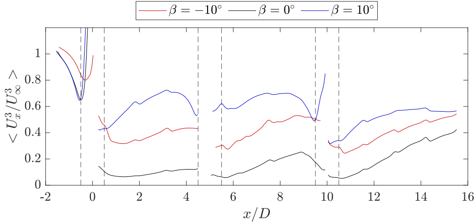
Figure 14. Mean available power \langle U_x^3/U_\infty^3 \rangle as calculated using Equation 5 for the three pitch cases over streamwise distance x/D within the projected frontal area of the central rotor column -0.5 < z/D, y/D < 0.5 . The vertical black dashed lines correspond to the boundaries of the swept volumes of the central column rotors.
