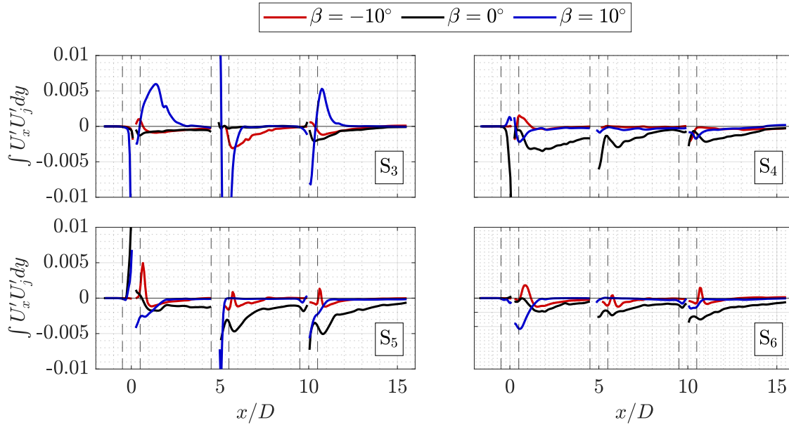
Figure 19. Line integrated Reynolds stress flux terms as a function of downstream position x/D through the surfaces j = S_{3,4,5,6} , as noted in Figure 17 for the three modes of operation. The flux terms are integrated within the lateral boundaries -0.5 \leq y/D \leq 0.5 . All values fluxes are normalized by the ratio of the turbine diameter to the product of the free stream wind speed and lateral integration length, 1/U_\infty^3 L , where L = D in this case. The vertical dashed line denotes the edges of the central rotor volumes.
