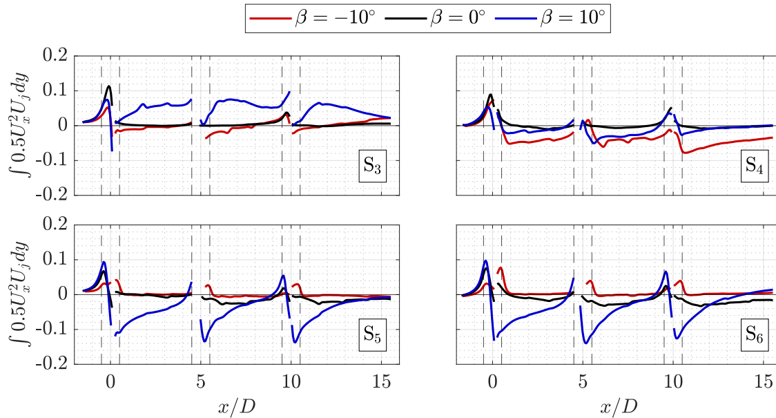
Figure 18. Line integrated advective flux terms as a function of downstream position x/D through the surfaces j = S_{3,4,5,6} , as noted in Figure 17 for the three modes of operation. The flux terms are integrated within the lateral boundaries -0.5 \leq y/D \leq 0.5 . All values fluxes are normalized by the ratio of the turbine diameter to the product of the free stream wind speed and lateral integration length, 1/U_\infty^3 L , where L = D in this case. The vertical dashed line denotes the edges of the central rotor volumes.
