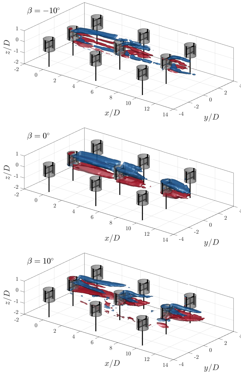
Figure A1. Iso-surfaces of the lateral vorticity contours at \omega_y D/U_\infty = \pm 1 for pitch cases \beta = \pm 10^\circ , and \beta = 0^\circ . The rotors are shown at a \theta = 0^\circ phase, with the gray-shaded cylinders representing the idealized actuator cylinder load.
