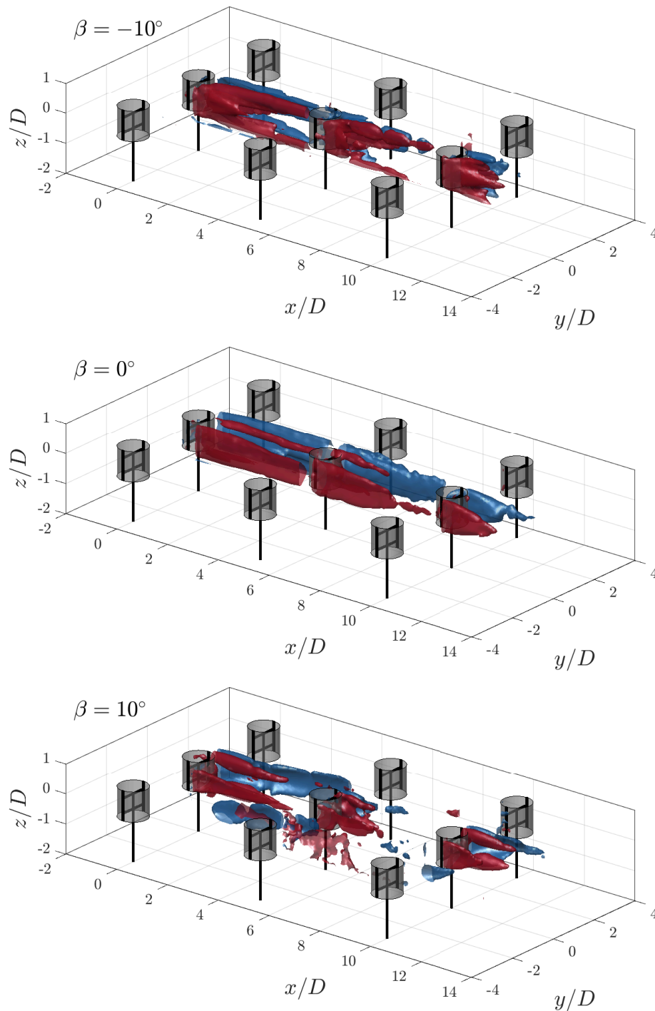
Figure A2. Iso-surfaces of the axial vorticity contours at \omega_z D/U_\infty = \pm 1 for pitch cases \beta = \pm 10^\circ , and \beta = 0^\circ . The rotors are shown at a \theta = 0^\circ phase, with the gray-shaded cylinders representing the idealized actuator cylinder load.
