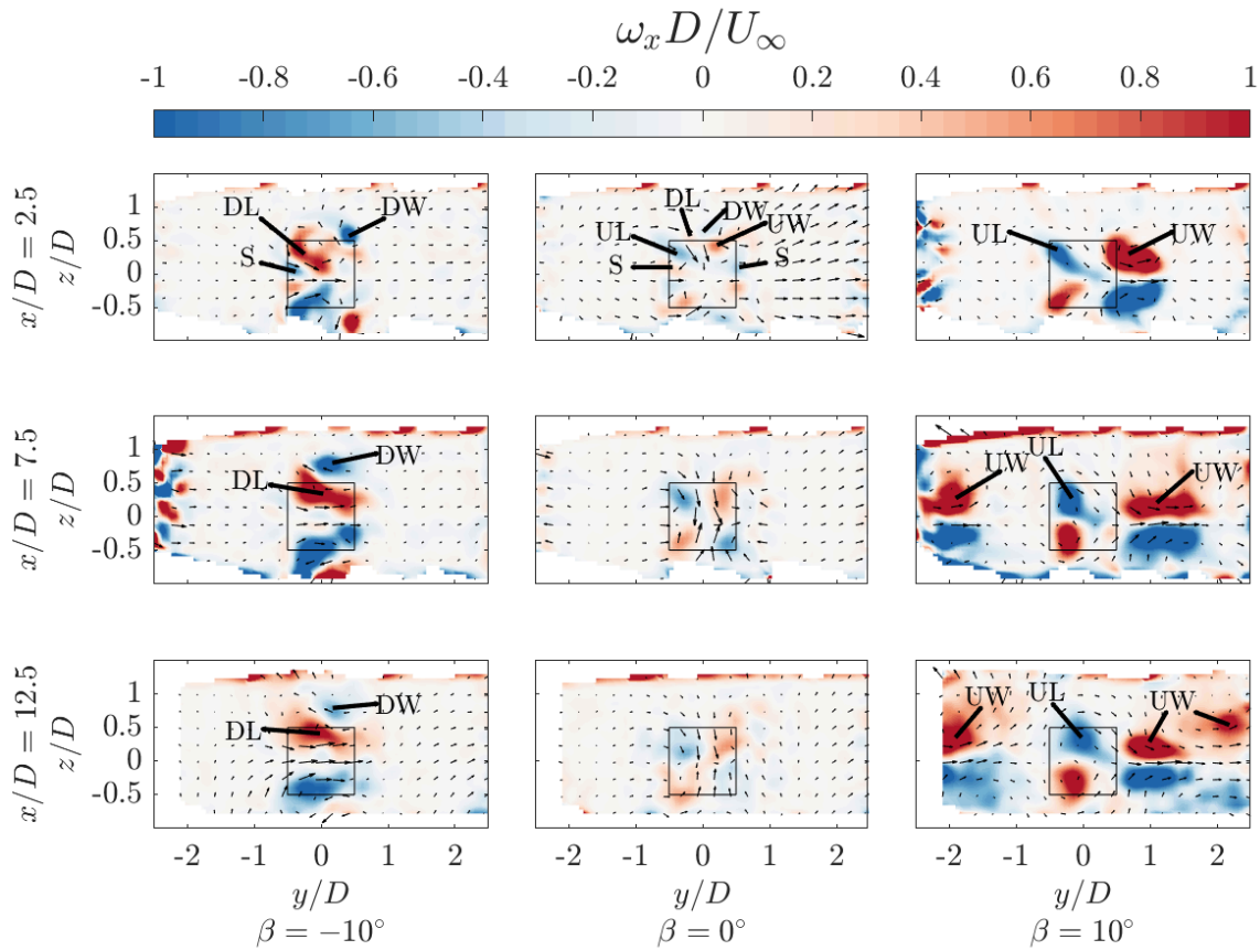
Figure 8. Normalized streamwise vorticity at \omega_x D / U_\infty for the three pitch cases at streamwise locations x/D = 2.5, 7.5, and 12.5 . The black outlined square indicates the projected frontal area of the rotors, and the vectors show the in-plane velocity components. The streamwise vortical structures generated by each AC load quadrant are labeled, as described in Section 2. The label S corresponds to structures generated at the interface between the struts and blade.
