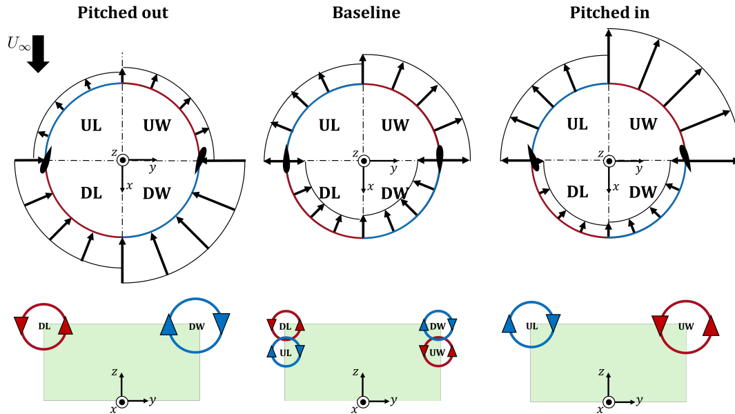
Figure 1. Top view schematic of the simplified AC force fields for the three "vortex generator" modes of operations adapted from Huang et al. (2023b); Bensason et al. (2024), namely the baseline case (where no pitch is applied), a pitched in case, and pitched out. Blades at a phase position of \theta = 0^\circ are shown at exaggerated sizes and pitch angles to demonstrate the pitching convention. The coordinate systems are shown at the center of the AC, and the rotation direction is anti-clockwise. The quadrants of the idealized AC are labeled as upwind windward UW 0^\circ < \theta < 90^\circ , upwind leeward UL 90^\circ < \theta < 180^\circ , downwind leeward DL 180^\circ < \theta < 270^\circ , and downwind windward DW 270^\circ < \theta < 360^\circ . The top edges of the rotor cylinder are color-coded based on the direction of rotation in the internal frame of reference of the trailing blade-tip vortices, with red and blue as counter-clockwise and clockwise, respectively. The top half of the rotor's projected frontal area (green) at a generic measurement plane downstream is shown below each mode. The projected dominant quadrant-labeled streamwise vortical structures stemming from the blade tips for each pitch case are shown via circular arrows.
