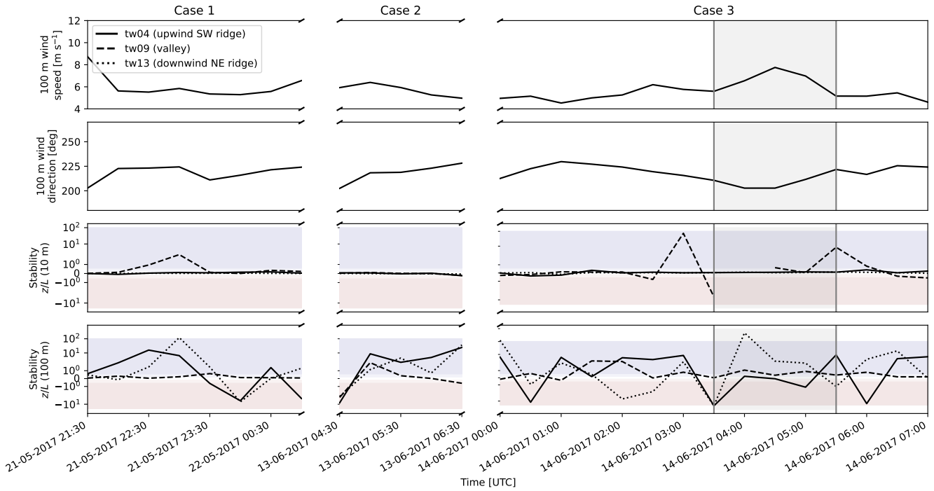
Figure 2. Thirty-minute averaged wind and stability metrics for the three selected case studies. Red and blue shading indicate areas in which the Obukhov stability parameter is unstable and stable, respectively. The gray shaded region within Case 3 indicates the simulation period.
