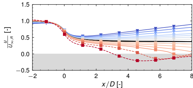
Figure B1. Normalized centerline velocity for C_T = \frac{8}{9} for different background velocity gradients. Grey area indicates negative velocities.
