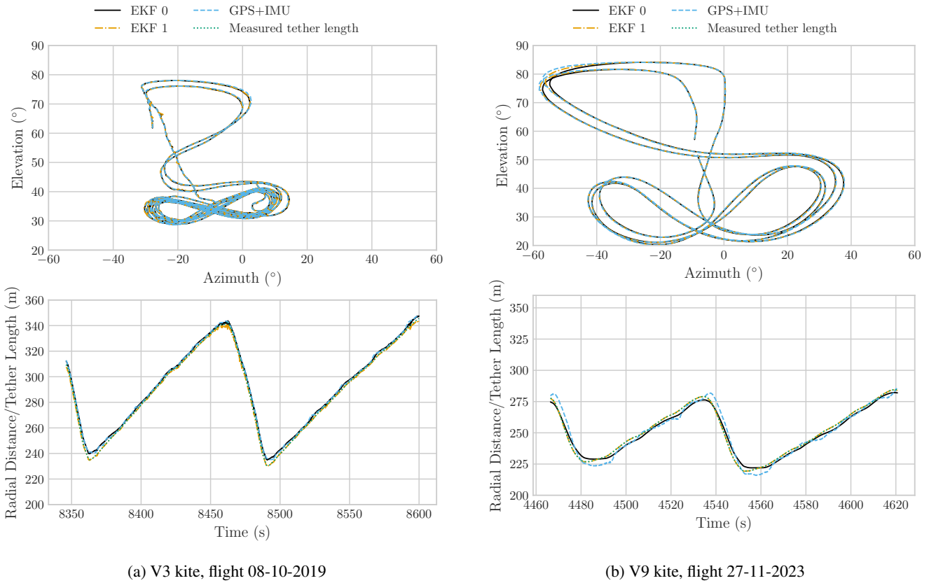
Figure 8. Comparison of estimated and measured kite trajectory, in terms of the azimuth and elevation angles and radial distance.
