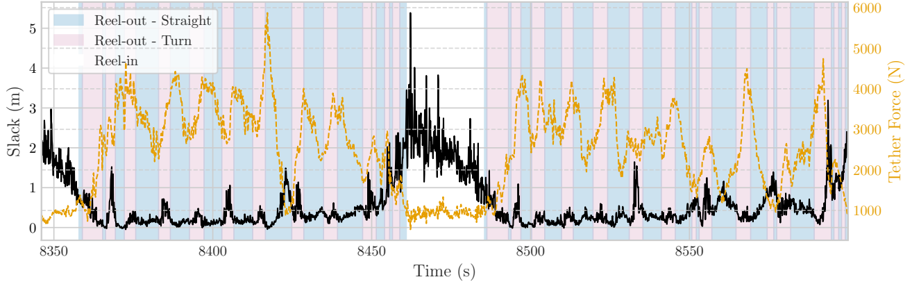
Figure 12. Variation of tether slack and force during two power generation cycles from the flight on 08-10-2019 using the V3 kite. The plot shows the slack in meters (left y-axis) and the tether force in Newtons (right y-axis).
