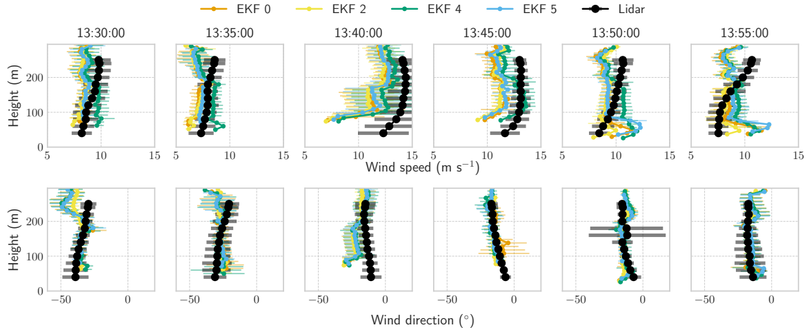
Figure 22. Test flight from 05-06-2024. Wind profile comparison of horizontal wind speed and direction estimated by the EKF using a minimal sensor configuration and three enhanced variants with additional inputs, compared to lidar observations. Wind profiles are averaged over 5-minute intervals.
