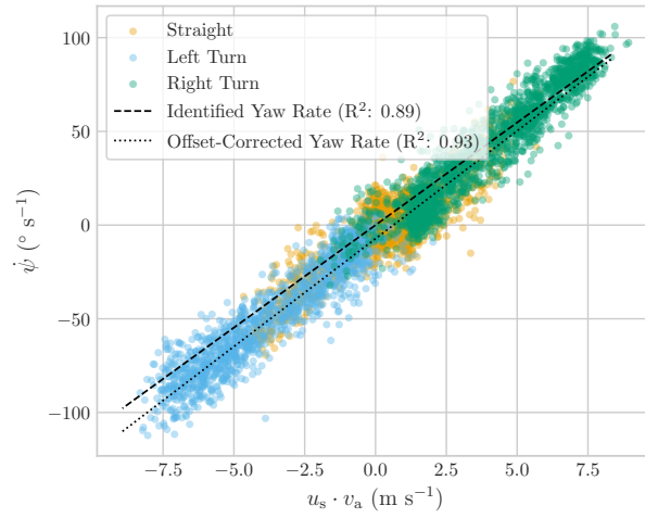
Figure 16. Measured yaw rate and identified turn rates of the V3 kite on 08-10-2019 during two power generation cycles. Identified turn rates are shown with and without offset correction.
