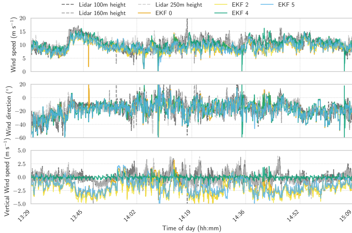
Figure 21. Test flight from 05-06-2024. Time series comparison of wind estimates from different EKF configurations, including a minimal sensor setup and three variants with additional inputs, against lidar observations. The plots show horizontal and vertical wind velocity components, as well as horizontal wind direction. Lidar data are available at 1-second resolution and are shown at three heights representative of the kite’s flight envelope.
