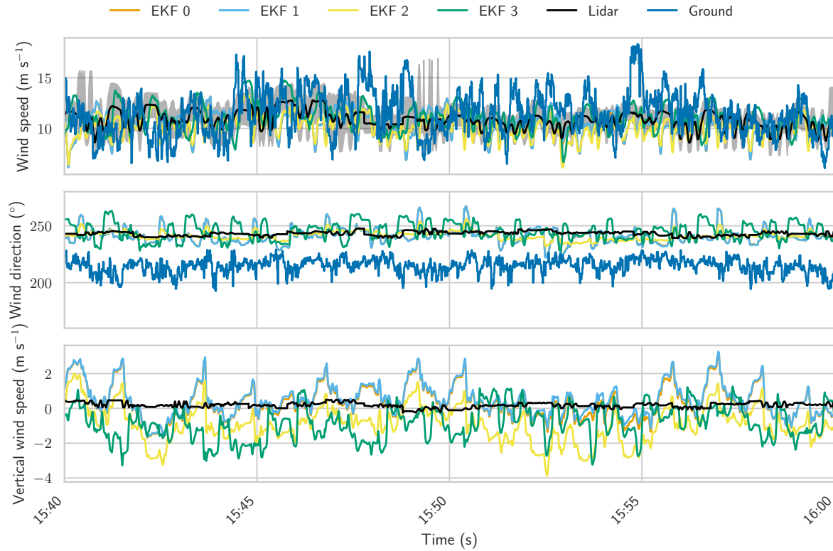
Figure 19. Test flight on 27-11-2023. Time series comparison of wind estimates from different EKF configurations, including a minimal sensor setup and three variants with additional inputs, against lidar observations and ground-based measurements. The plots show horizontal and vertical wind velocity components, as well as horizontal wind direction. Lidar data are available at 1-minute resolution, interpolated to kite altitude, with the mean and range (minimum–maximum) shown in grey. Ground-based wind speed measurements are extrapolated to kite height using a logarithmic wind profile.
