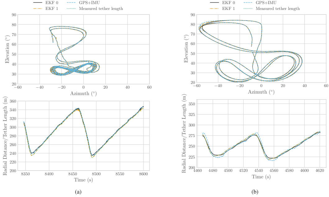
Figure 8. Comparison of estimated and measured kite trajectories. (a) V3 kite on 08-10-2019. (b) V9 kite on 27-11-2023. The trajectories are shown in terms of azimuth, elevation angle, and radial distance.
