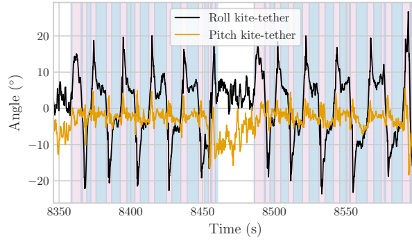
Figure 18. Estimated angle between tether and kite for the V3 kite during two power generation cycles. The background colors indicate the flight phase of the kite, legend can be found in Figure 12.
