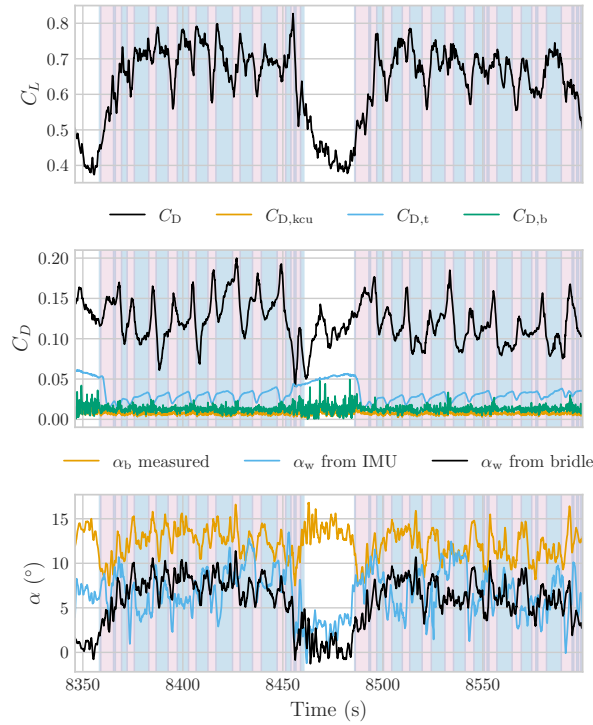
Figure 13. Aerodynamic coefficients and angle of attack of the V3 kite on 08-10-2019 during two power generation cycles. The background colours indicate the flight phase of the kite; the legend is provided in Figure 12.
