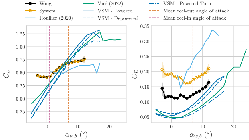
Figure 14. Estimated aerodynamic polars of the V3 kite from the flight on 08-10-2019 using the reconstructed wing angle of attack. The angle of attack is obtained by translating the measured angle at the bridle lines to the wing reference frame. Mean values are shown with shaded areas indicating the 99% confidence interval. Results are compared to previous studies.
