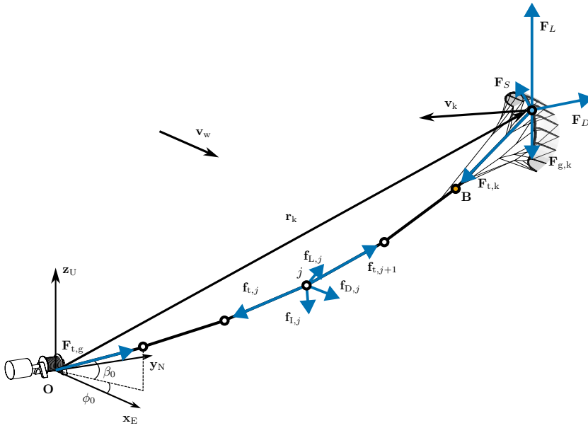
Figure 4. Schematic representation of the tether model and kite forces, as represented by the dynamic model used in the EKF. Adapted from Schelbergen and Schmehl (2024).
