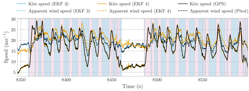
Figure 9. Comparison of the estimated and measured kite speed and apparent wind speed during the flight on 08-10-2019 using the V3 kite. The comparison is done for a configuration with (EKF 3) and without (EKF 4) apparent wind speed measurements.
