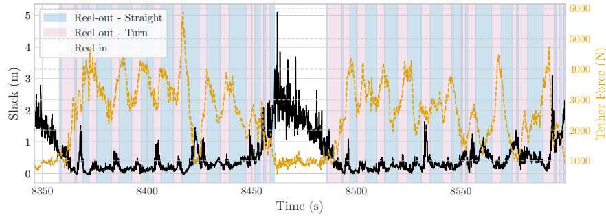
Figure 12. Variation of tether slack and force during two power generation cycles from the flight on 08-10-2019 using the V3 kite. The plot shows the slack in meters (left y-axis) and the tether force in Newtons (right y-axis).
