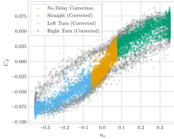
Figure 17. Side force coefficient estimated by the EKF for the V3 kite on 08-10-2019 during two power generation cycles, with and without time delay correction.
