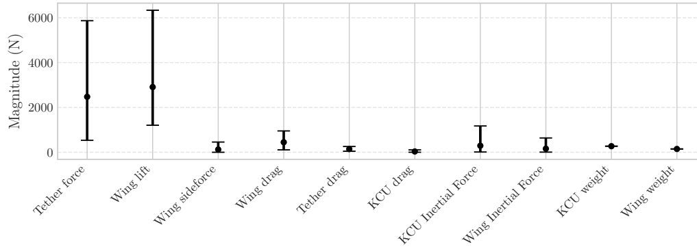
Figure 11. Mean, maximum, and minimum values of the different force contributions acting on the airborne subsystem during the flight on 08-10-2019 using the V3 kite. These forces were computed based on the estimated states obtained from the EKF described in section 4.
