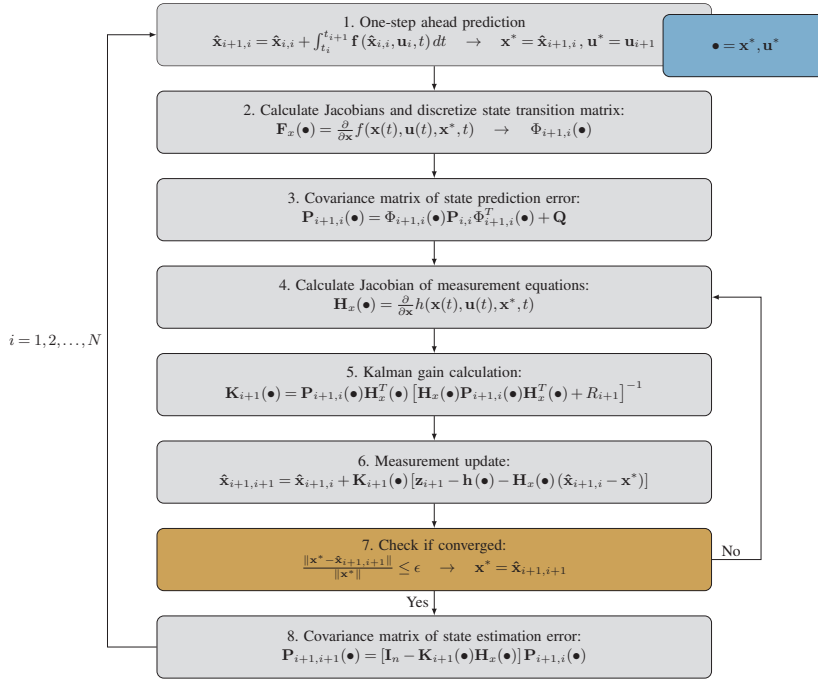
Figure 6. Iterated extended Kalman filter process flowchart. In the case of a non-iterated EKF, the process continues directly from step 7 to step 8, bypassing the iteration loop.
