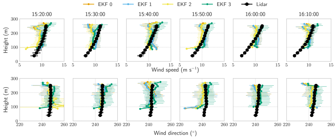
Figure 20. Test flight on 27-11-2023. Wind profile comparison of horizontal wind speed and direction estimated by the EKF using a minimal sensor configuration and three enhanced variants with additional inputs, compared to lidar observations. Wind profiles are averaged over 10-minute intervals.
