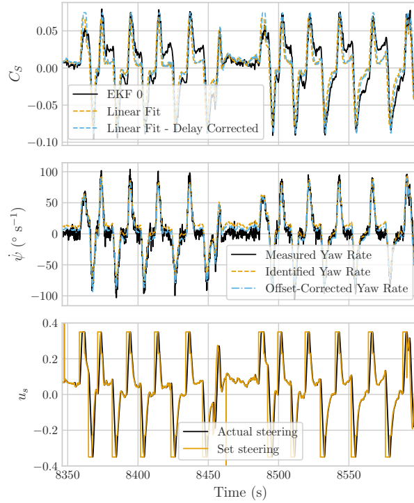
Figure 15. Side force coefficient, yaw rate, and steering input of the V3 kite on 08-10-2019 during two power generation cycles. Linear fits are shown for the side force coefficient and yaw rate to highlight their relation to the steering input.
