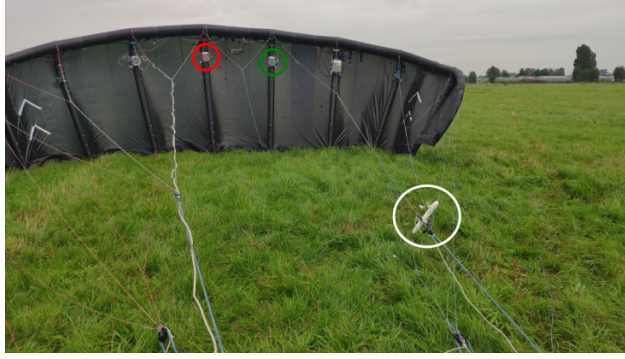
Figure 3. Fully instrumented V3.25 kite before launch. GPS+IMU units are mounted in the inflatable struts (highlighted by red and green circles). A Pitot tube and a wind vane are installed in the bridle lines (white circle). Photo courtesy of Kitepower B.V.
