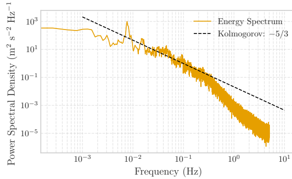
Figure 23. Power spectral density of the wind speed during the test flight on 08-10-2019. The reference -5/3 Kolmogorov slope is shown for comparison, indicating the expected inertial subrange behavior in atmospheric turbulence.
