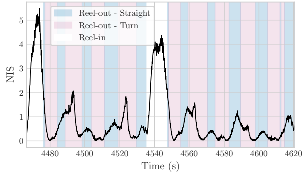
Figure 7. Normalized innovation squared (NIS) metric for two power generation cycles of the V9 kite, recorded on 27-11-2023.
