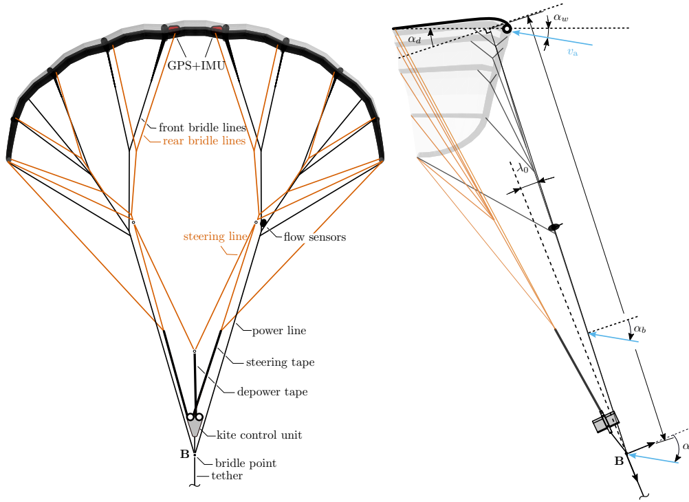
Figure 1. Illustration of system components and sensor setup. Adapted from Oehler and Schmehl (2019). The V3 kite geometry shows the bridle point B below the KCU, unlike the V9 geometry where the KCU is at the bridle point. All geometry data for the V3 kite are available in open-access from Poland and Schmehl (2024).
