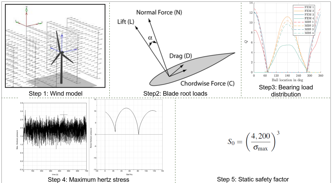
Figure 1. Illustration of the procedure used to calculate the static safety factor
