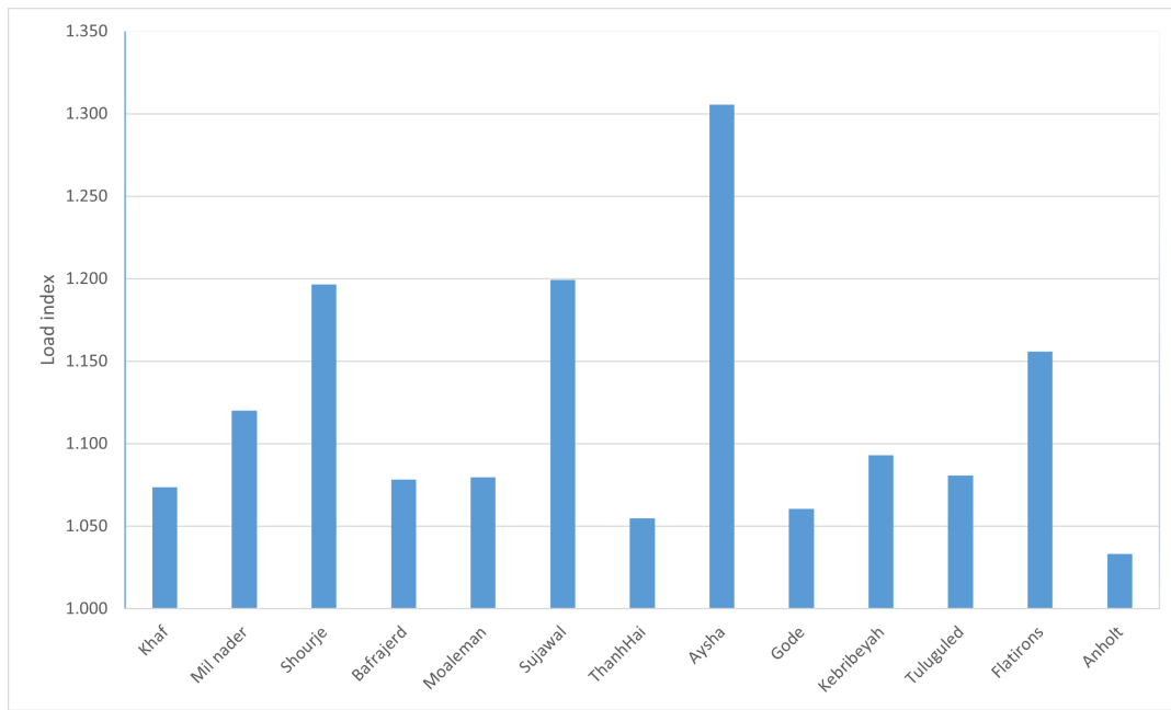
Figure 11. Load index of wind sites
