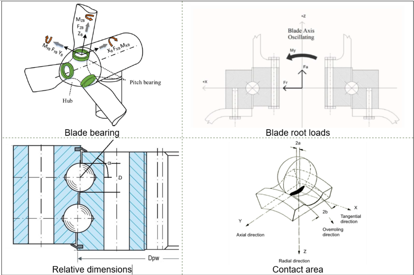
Figure 1. Illustration of the important processes used to calculate the static safety factor, images extracted from He et al. (2024); Harris et al. (2009); Rezaei et al. (2023); Solano-Alvarez (2015)
