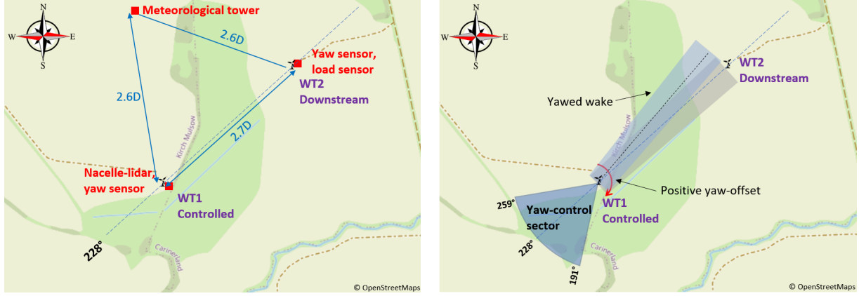
Figure 1. Wind farm layout at Kirch Mulsow test site; left: turbine spacing and distance to the met mast indicated; right: wind sectors for the control-experiment indicated ; adapted from Hulsman et al. (2022). © OpenStreetMap contributors 2024. Distributed under the Open Data Commons Open Database License (ODbL) v1.0.
