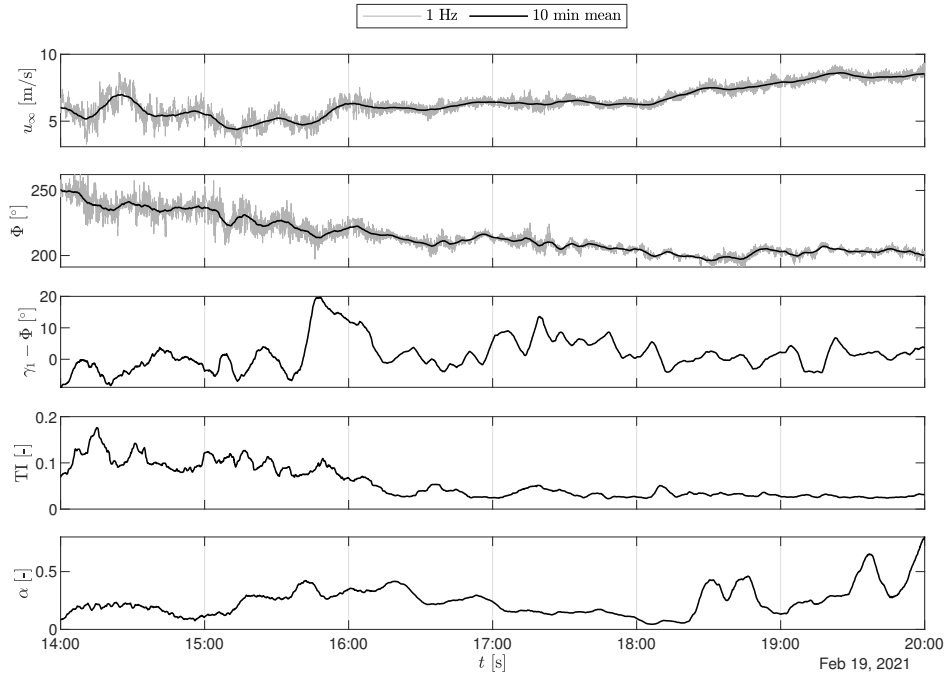
Figure 14. Ambient conditions on 19th of February, same time instance as shown in Figure 13; ambient wind speed u_\infty and wind direction \Phi are shown both as 1Hz and 10min average; the TI refers to 10min bins by definition and the same was applied to power law coefficient \alpha and WT1 yaw misalignment \gamma_1 - \Phi .
