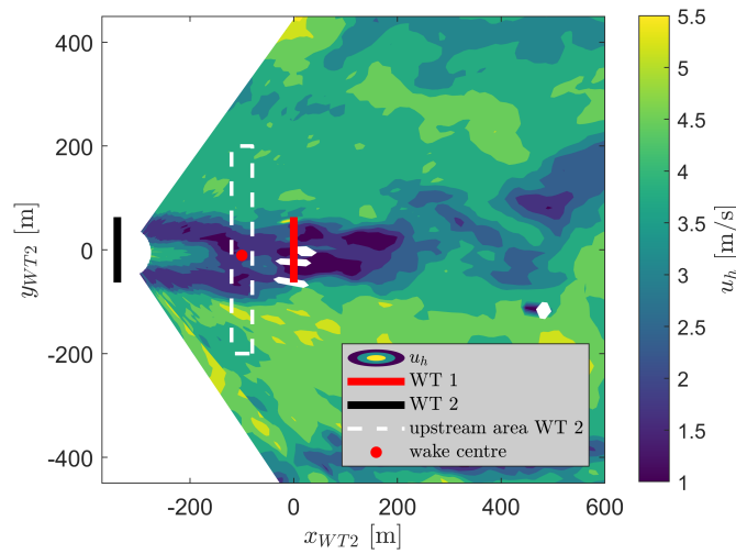
Figure 6. Wake centre identification from lidar measurements in WT2-based coordinate system. The wind direction here is 205°, resulting in a partial wake constellation.
