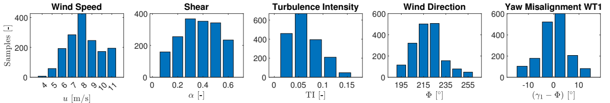
Figure 9. Histogram of ambient conditions contained in the investigated data set; all measurements refer the met mast (except for \gamma_1 , which is probed via GNSS on WT1)
