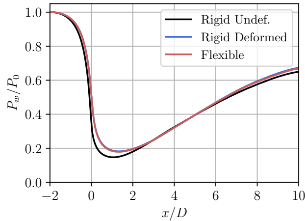
Figure 17. Available power in the wake (normalized by the power at the inflow), computed over the rotor swept area at various streamwise location.
