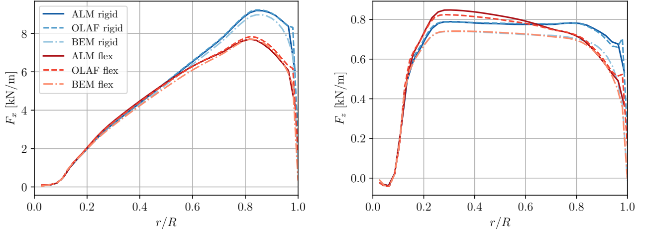
Figure 4. Steady state aerodynamic loads in the blade root frame for the rigid (blue) and flexible (red) cases: ALM (dark solid), free vortex wake model OLAF (dash) and the BEM (light dash-dot) from OpenFAST. Normal ( F_x , left) and lateral ( F_z , right) forces (relative to the blade root frame).
