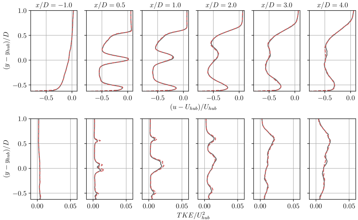
Figure 21. Profiles of mean velocity deficit (top) and turbulent kinetic energy (bottom) in the near wake of the turbine at various downstream locations. Comparison between the 64 pts/D (gray) and 128 pts/D (dashed red) resolutions.
