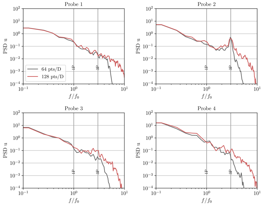
Figure 22. PSD of the streamwise velocity at various locations (as depicted in Figure 20). Comparison between the 64 pts/ D (gray) and 128 pts/ D (red) resolutions.
