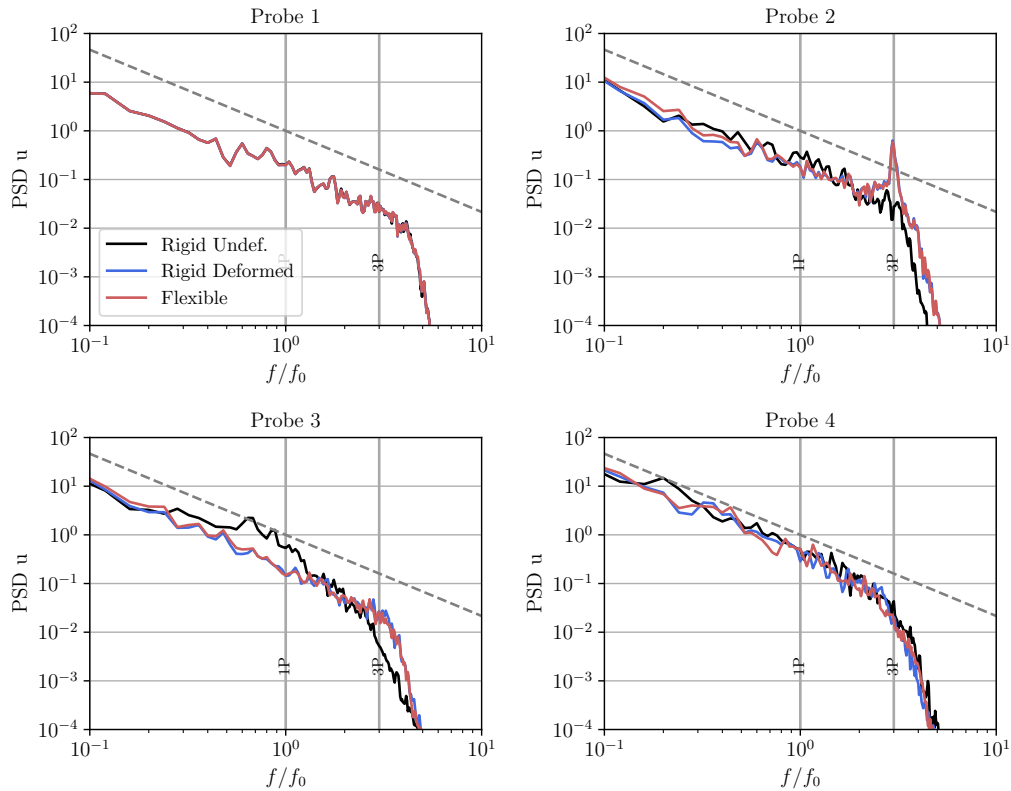
Figure 16. PSD of the streamwise velocity at various locations (as depicted in Figure 15). The dashed line indicates the (f/f_0)^{-5/3} function.
