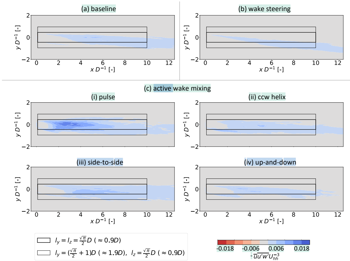
Figure 14. Contours of normalized -\overline{u'u'w'} along the xy plane at z = \frac{1}{4}\sqrt{\pi}D , or \approx 0.44D (i.e., the top surface of the control volume). Positive (blue) values indicate MKE flux into the control volume from aloft. The flow is viewed from above looking down.
