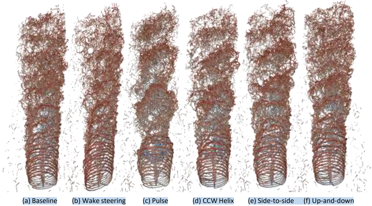
Figure 6. Renderings of instantaneous wake structures for each of the cases in Table 3 using Q isocontours at a level of 0.025. Coloring is according to streamwise velocity.
