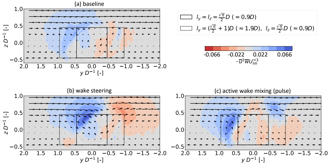
Figure 13. Contours of normalized -\overline{u^2 \overline{w}} along the yz plane at x = 3D . Positive (blue) values along the top face indicate MKE flux into the control volume. Vectors are composed of \overline{v} and \overline{w} and have the same scaling based on magnitude in all panels. The flow is viewed from upstream looking downstream.
