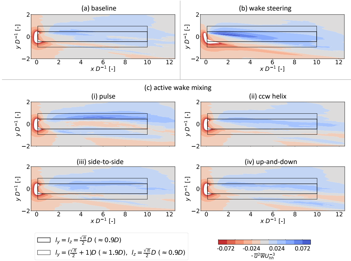
Figure 12. Contours of normalized -\overline{u}^2\overline{w} along the xy plane at z = \frac{1}{4}\sqrt{\pi}D , or \approx 0.44D (i.e., the top surface of the control volume). Positive (blue) values indicate MKE flux into the control volume from aloft. The flow is viewed from above looking down.
