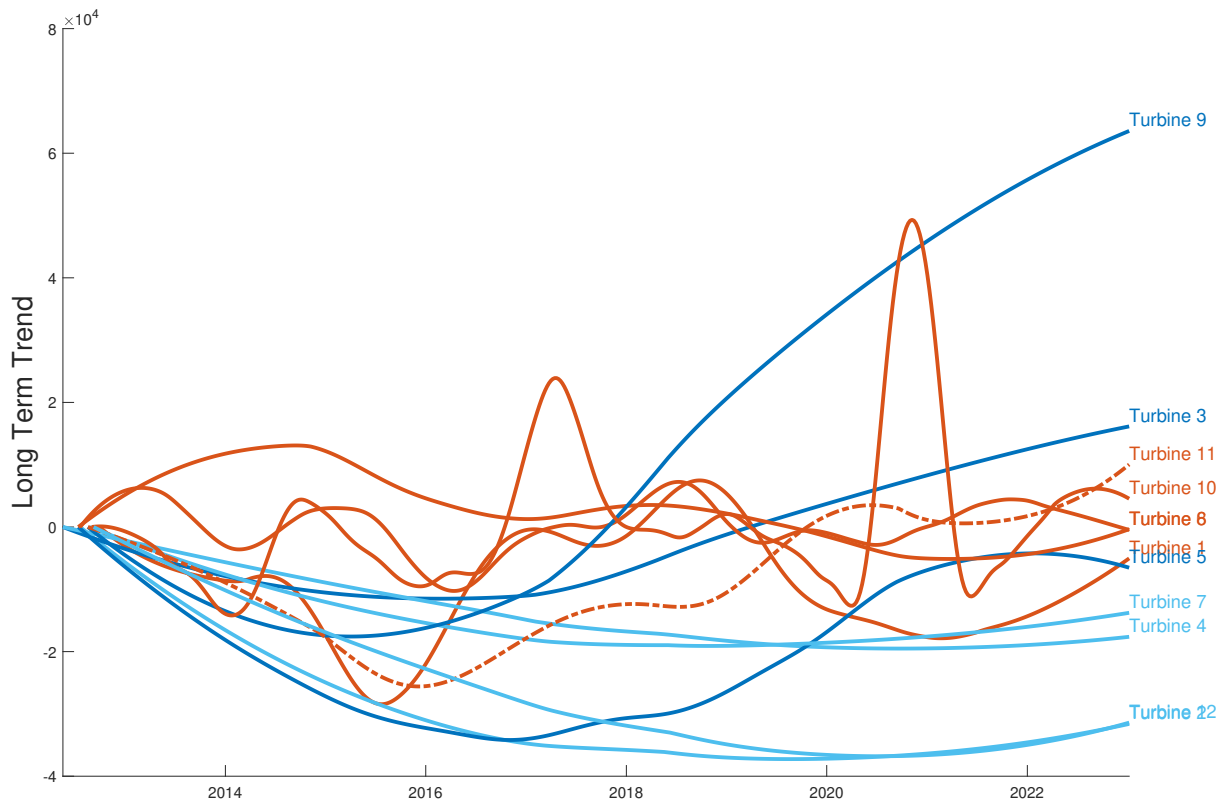
Figure 6. Grouped Long-Term Trends in Turbine Performance: Analysis of Shared Trajectories Among Twelve Turbines.
