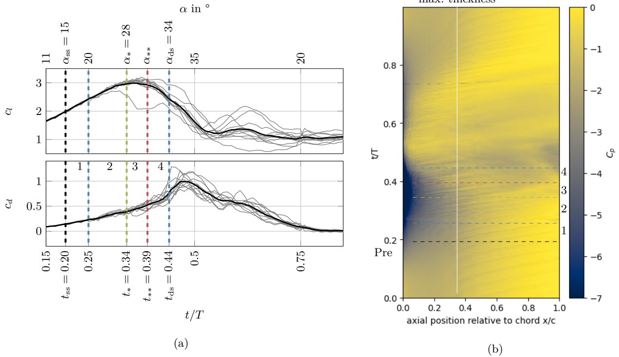
Figure 6. Evolution of dynamic stall in different phases for 20^\circ \pm 15^\circ , static stall at t_{ss} , localized stall at t_* , full stall at t_{**} , and deep stall at t_{ds} : (a) Phase-averaged (black) and individual (gray) lift and drag coefficients, (b) Spatiotemporal plot of phase-averaged pressure coefficient c_p on the suction side.
