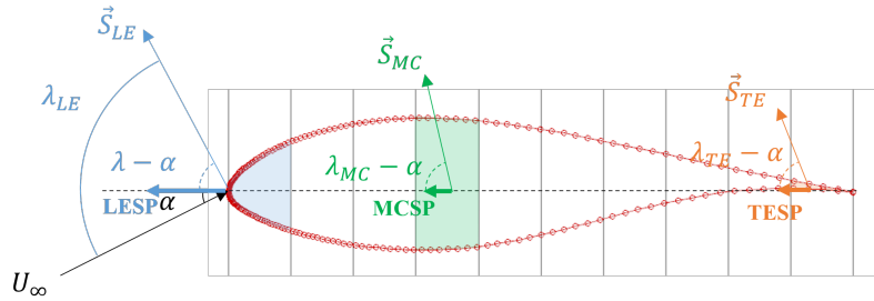
Figure 10. Positions of numerical probes and definitions of suction parameters
