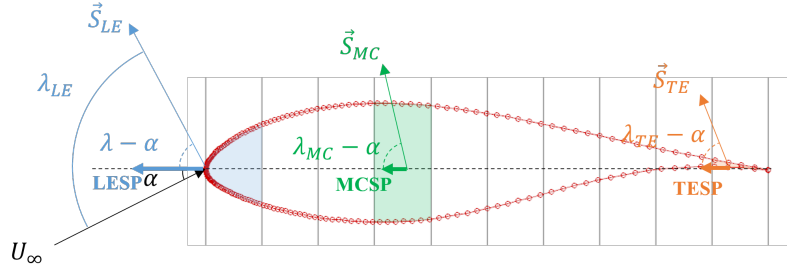
Figure 10. Positions of numerical probes and definitions of suction parameters
