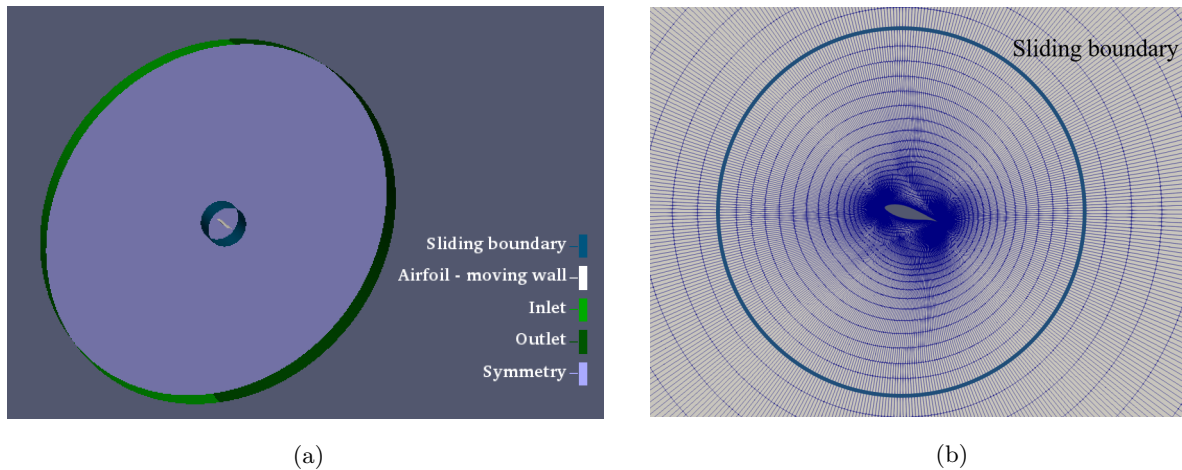
Figure 2. Numerical domain (a) boundary types (b) mesh around the airfoil, blue line indicating the interface between pitching and stationary domains
