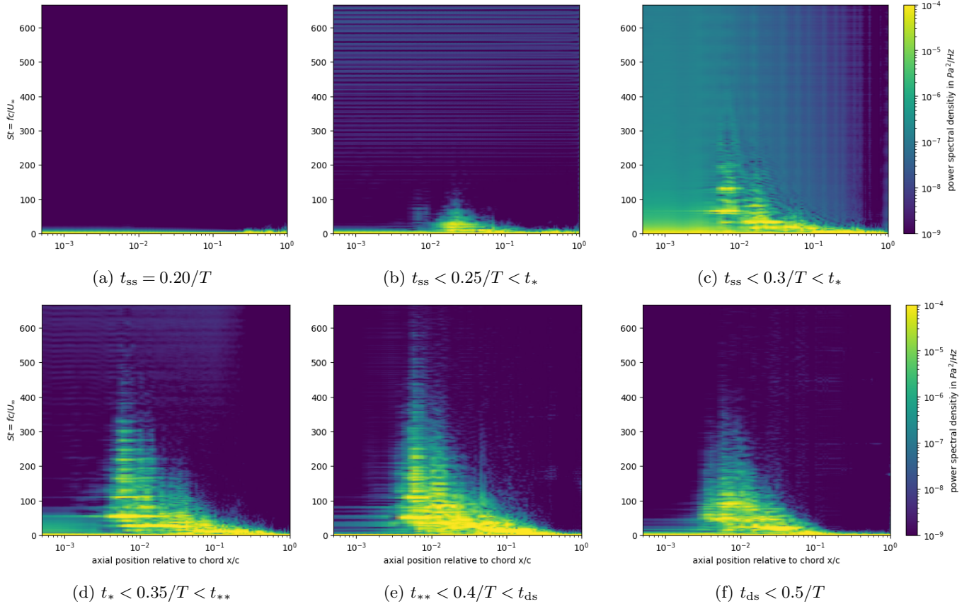
Figure 8. Power spectral density of phase-averaged pressure coefficient c_p on the suction side of the airfoil during dynamic stall, frequency non-dimensionalized as St = fc/U_\infty . (a) At static stall, (b) Initial instability (Stage1-2), (c) Attached vortex street (Stage2), (d) Peak lift (Stage3), (e) Full stall (Stage4), (f) Deep stall
