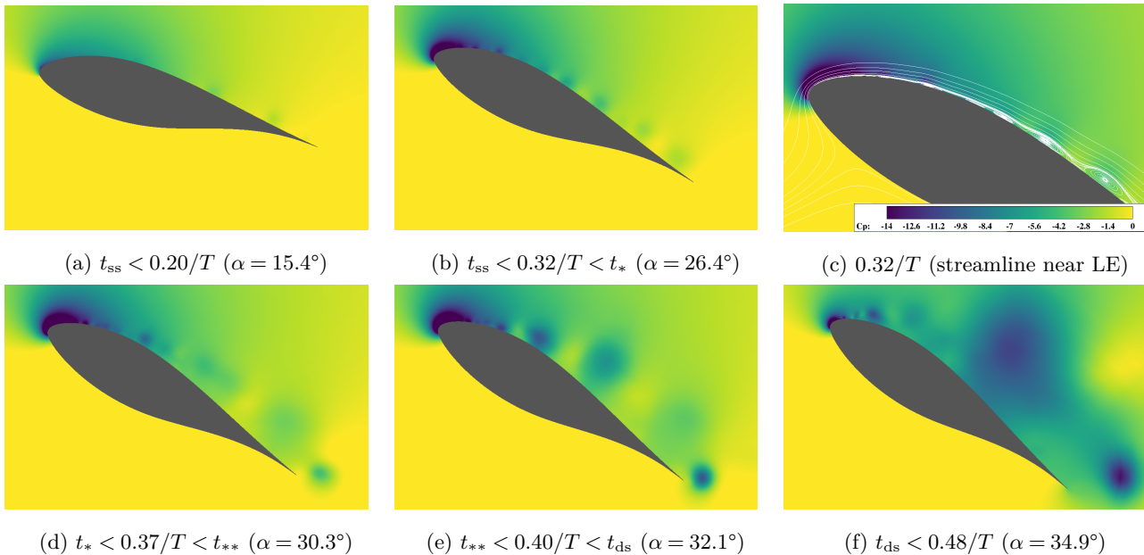
Figure 7. Instantaneous pressure coefficient C_p through during a dynamic stall (a) Initial instability (Stage1), (b)(c) Attached vortex street (Stage2), (d) Lift peak, localized stall (Stage3), (e) Full stall (Stage4), (f) Deep stall
