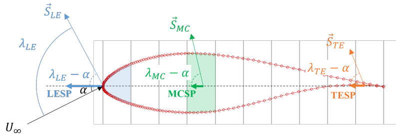
Figure 10. Positions of numerical probes (red dots) and definitions of suction parameters
