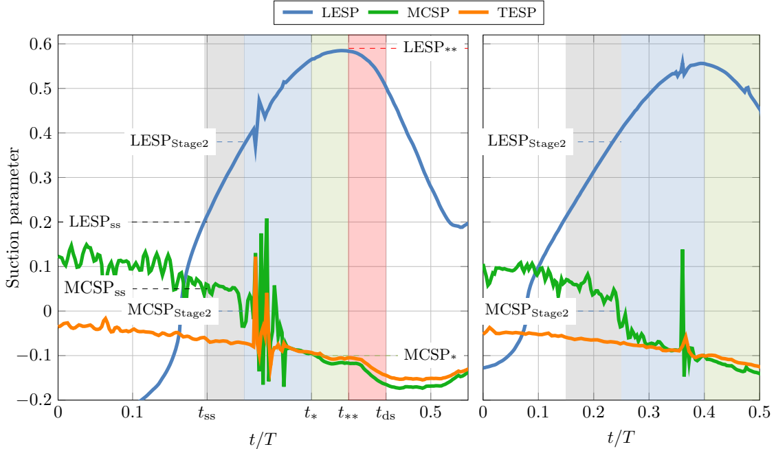
Figure 11. Leading-edge suction parameter (LESP), mid-chord suction parameter (MCSP), and trailing-edge suction parameter (TESP) from the pitching case of 20^\circ \pm 15^\circ (left) and 20^\circ \pm 10^\circ (right). The shaded regions refer to initial instability (gray), attached DSV (blue), lift peak (green), full stall (red)
