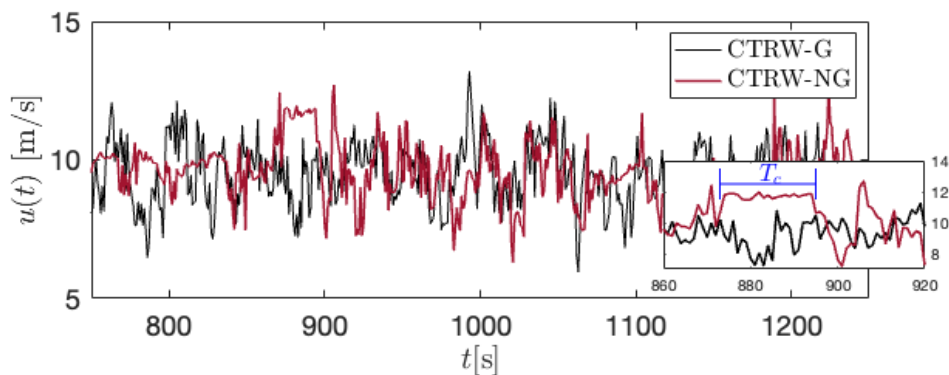
Figure 8. Excerpt of the wind speed time series u(t) for CTRW-G and CTRW-NG. A visible CWS period T_c is visible between 875 and 895s for the CTRW-NG. The exponent for the Lévy distribution of the CTRW-NG is \alpha_L = 0.9 .
