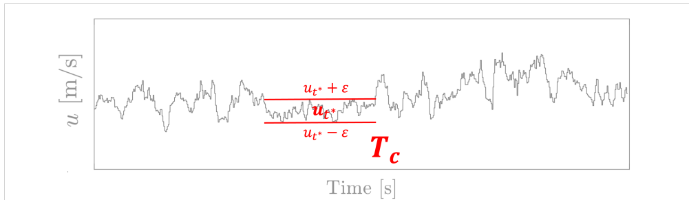
Figure 1. Schematic representation of a CWS period ( T_c ) measured from an exemplary wind speed time series u(t) . The constant speed interval range (CSR), u_{t^*} \pm \varepsilon specifies the limits for the accepted level of turbulence within a period T_c . The CSR is depicted by the horizontal red bars.
