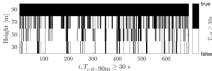
Figure G1. Events T_c > T_{min} at different heights, conditioned on \tilde{H} = 90 m. First, the reference height \tilde{H} is defined. Next, for each i event T_{c,i} > T_{min} at H = \tilde{H} , the occurrence of T_c at the remaining heights H = [70, 50, 30] m is evaluated. Black lines depict the occurrence of an event. The T_c at all heights H are conditioned so that T_c > T_{min} . For the example in this figure, T_{min} = 30 s and \tilde{H} = 90 m.
