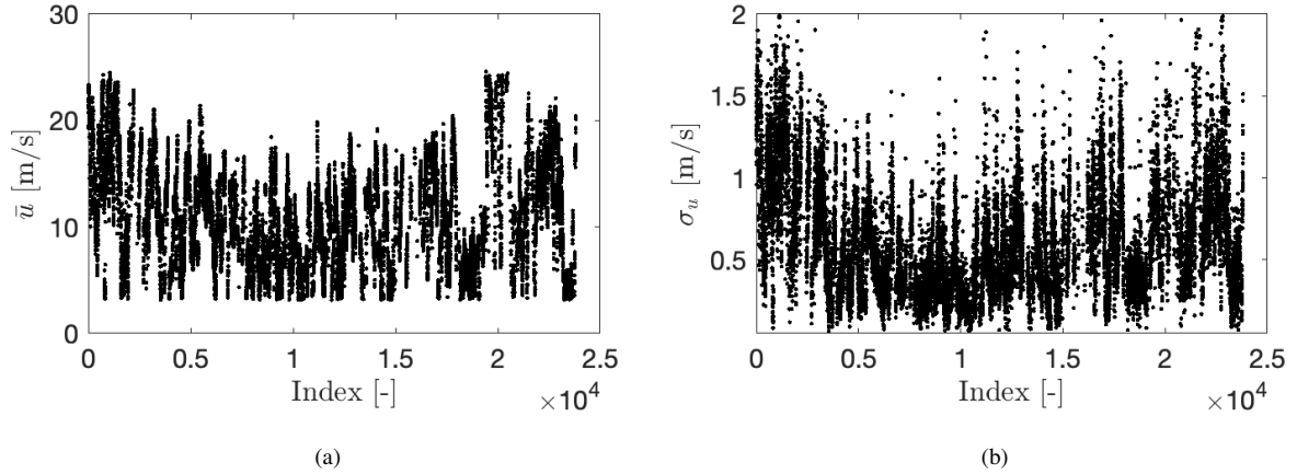
Figure 2. Wind velocity statistics of atmospheric FINO data at H = 90\text{ m} . (a) Mean wind speed \bar{u} . (b) Standard deviation \sigma_u . Each dot in the plots corresponds to a calculated value over a single 10-minute period. The dots are chronologically ordered.
