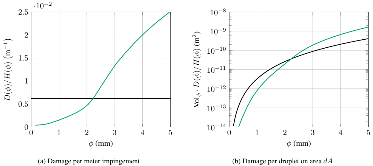
Figure 11. Normalized and absolute erosion damage for a single droplet at varying diameters; IEA 15MW turbine located at De Kooy; without drop-size effects: —; with drop-size effects: —.
