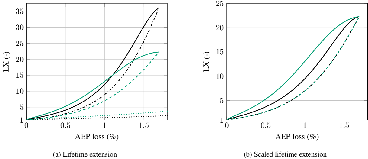
Figure 16. Pareto curves of lifetime extension as a function of the AEP loss; without drop-size effects, S-ESM: \cdots\cdots , V-ESM: -\cdot-\cdot- , VI-ESM: \text{—} ; with drop-size effects, S-ESM: \cdots\cdots , V-ESM: -\cdot-\cdot- , VI-ESM: \text{—} ; for more information on how to interpret this figure the reader should consult Fig. B1 and B5 and their corresponding explanation in the text; IEA 15MW turbine located at De Kooy.
