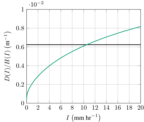
Figure 13. Normalized erosion damage per meter of impingement at various rain intensities; IEA 15MW turbine located at De Kooy; without drop-size effects: —; with drop-size effects: —.
