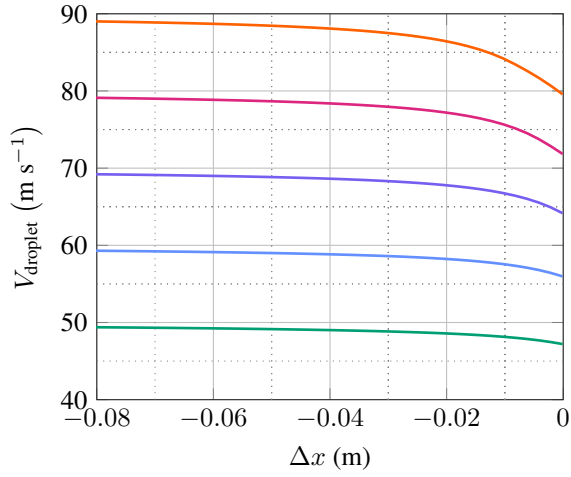
(a) Relative velocity of 0.49 mm diameter droplets versus distance to the leading edge \Delta x .
