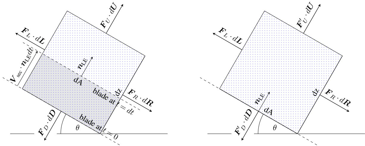
(a) Control volume fixed in the air; it is swept by a wind turbine (b) Control volume mapped to reference frame of the blade; the blade section dA ; the swept volume during dt is indicated in light gray. boundary D has become the leading-edge of the blade.
