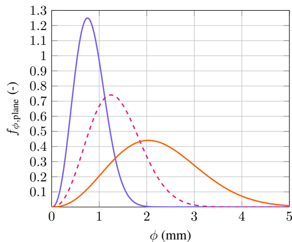
Figure 12. Best's distribution for a plane as a function of droplet diameter in millimeters for different rain intensities; rain intensities 0.1 mm hr -1 : —, 1 mm hr -1 : - - -, 10 mm hr -1 : —; the figure is partly reproduced from Barfknecht and von Terzi (2023).
