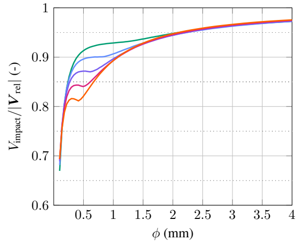
(b) Non-dimensional impact velocity as a function of droplet diameter.
