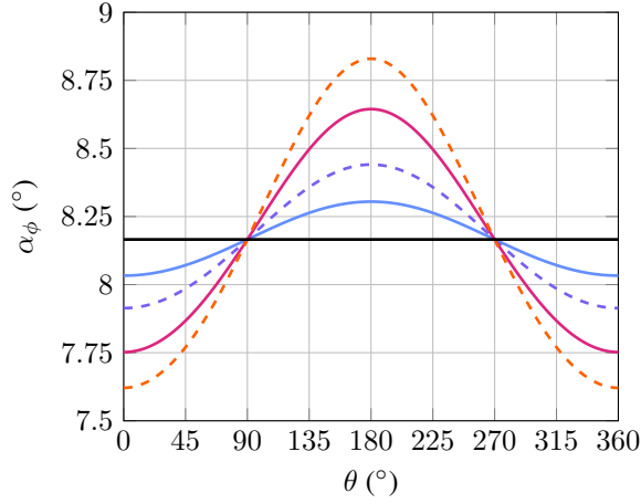
(a) Impact angle
