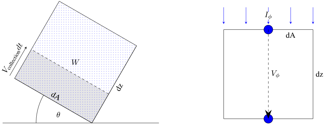
(a) Flow domain of air with rain (blue dots); it is oriented at an arbitrary blade angle \theta and is swept by a wind turbine blade section dA ; the swept volume during dt is indicated in light gray. (b) Control volume for the derivation of W ; rain enters at the top of the control volume; it subsequently falls through the volume until it reaches the lower boundary.
