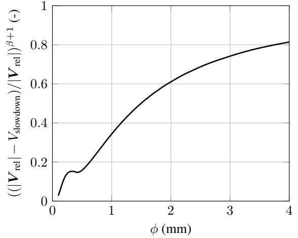
Figure 9. Non-dimensional damage due to the slowdown effect versus slowdown velocity and droplet diameter; \beta = 9.58 , |\mathbf{V}_{rel}| = 86.5 \text{ m s}^{-1} , R_c = 0.064 \text{ m} and n = 1.097 .
