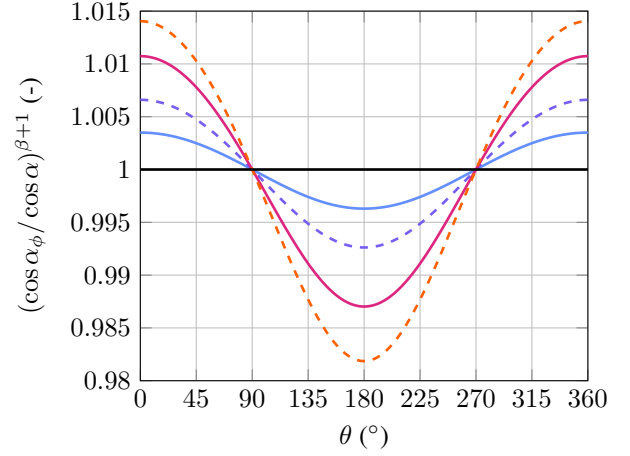
(b) Non-dimensional damage
