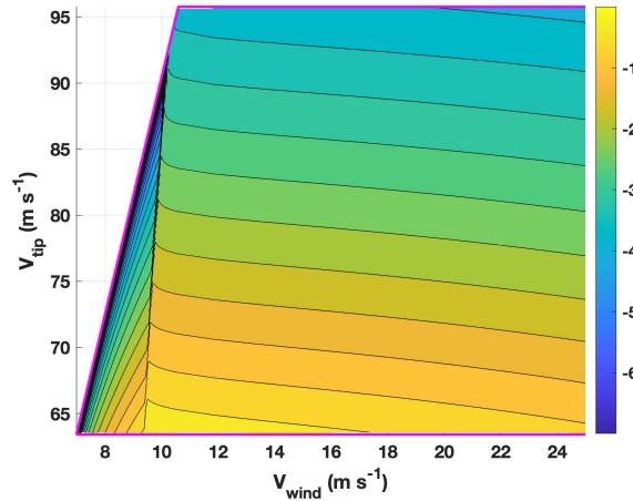
(c) \ln(\eta)
