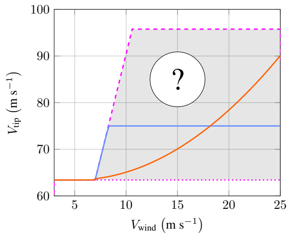
Figure B2. Operational tip-speed regime of the IEA 15MW turbine as a function of the instantaneous wind speed; g_{\min}(V_{\text{wind}}) : \cdots , g_{\text{normal}}(V_{\text{wind}}) : -\cdots- , ESM based on limit (C-ESM): — , ESM based on a parabolic equation: — .
