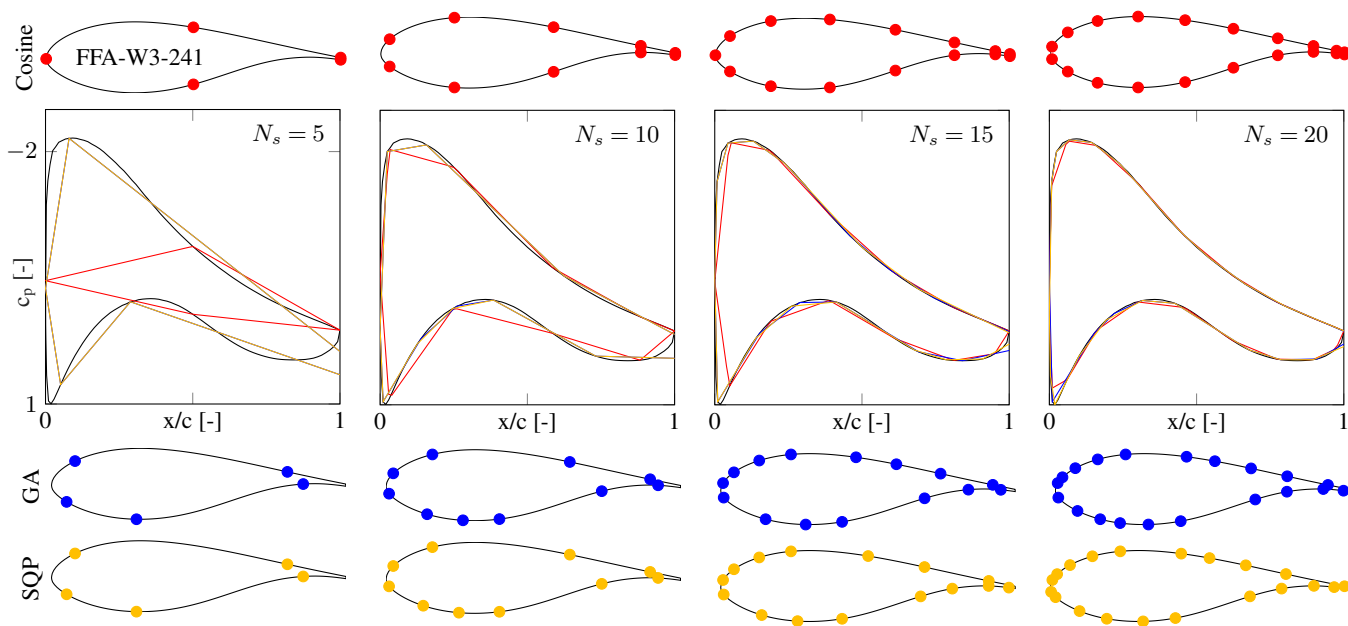
Figure 9. Accuracy in representing the expected (black) pressure distribution when using a cosine sensor spacing (red) and optimized layouts (blue and yellow) for a varying number of sensors, shown for the FFA-W3-241 airfoil and \alpha = 6.75^\circ
