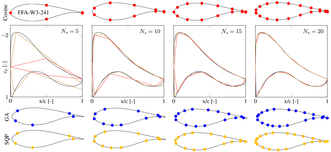
Figure 9. Accuracy in representing the expected (black) pressure distribution when using a cosine spacing (red) and optimized layouts (blue and yellow) for a varying number of sensors, shown for the FFA-W3-241 airfoil and \alpha = 6.75^\circ
