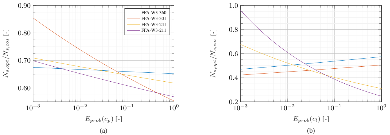
Figure 12. Ratio of required number of sensors between an optimized and cosine-spaced sensor layout to represent the pressure distribution (a) and the lift coefficient (b) with a specified accuracy
