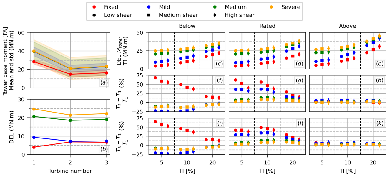
Figure 14. (a) Illustration of the mean (solid line) and standard deviation (shaded area) of the fore-aft tower-base moment along the array for a given wind condition (mean wind speed 8m/s, TI 5%, low shear). (b) similar illustration, but for the tower-base moment DEL. (c-e) DEL of the tower-base moment of the free-stream turbine (T1) across all the environmental conditions considered in this work. The relative difference between the tower-base moment DEL of (f-h) the first waked turbine (T2) and T1, and (i-k) the second waked turbine (T3) and T1.
