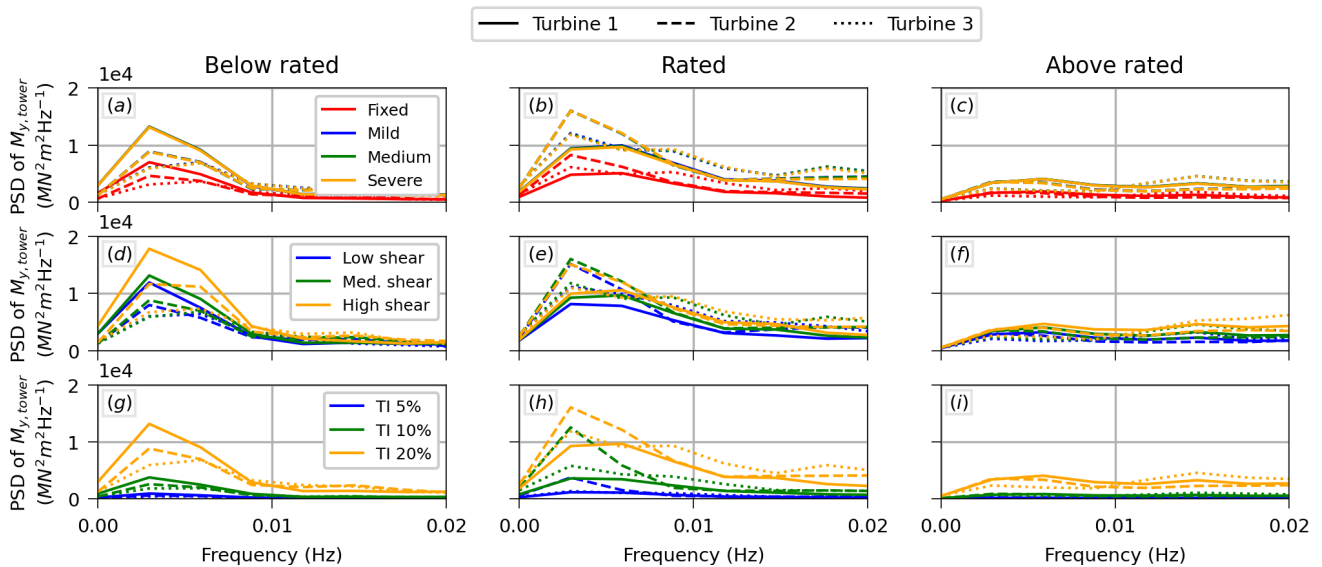
Figure 16. PSD of the fore-aft tower-base moment at the frequency range excited by the turbulent wind for the three different mean wind speeds. (a-ea-c) Different sea conditions for TI 20% and medium shear. (d-fd-f) Different shear conditions for the severe sea state and TI 20%. (g-ig-i) Different TI conditions for the severe sea state and medium shear.
