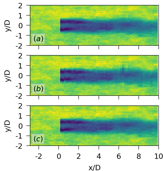
Figure 6. Top view of the wake obtained with FAST.Farm for (a) the fixed turbine with the recommended value of f_c = 0.083\text{Hz} for this case, (b) the floating turbine with the recommended value of f_c = 0.083\text{Hz} , and (c) the floating turbine with f_c = 0.010\text{Hz} , a value close to the resonance frequency of surge.
