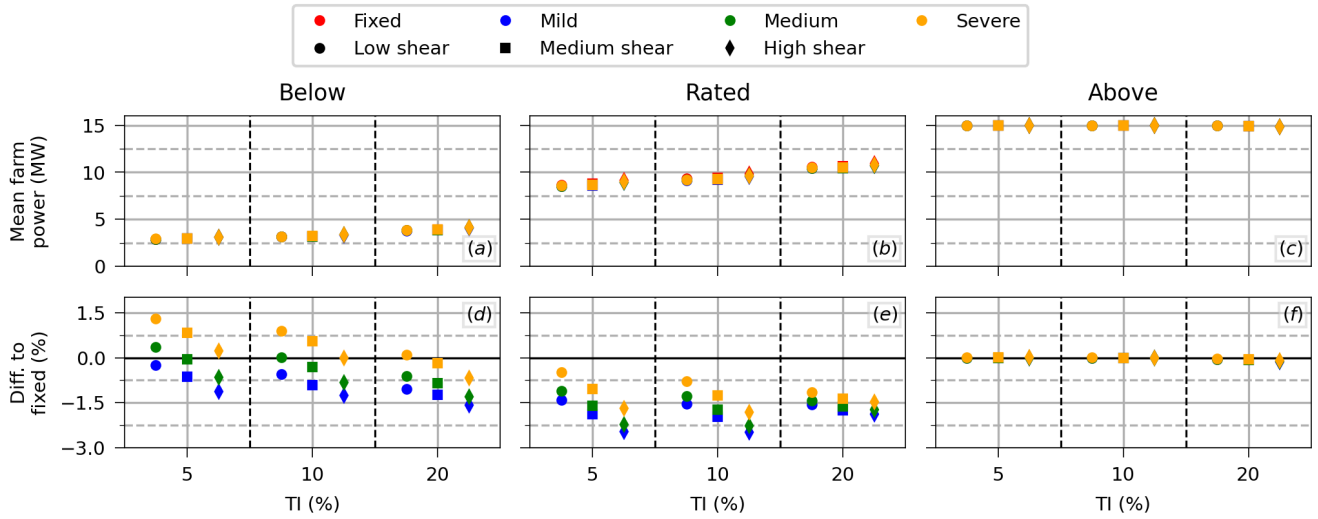
Figure 11. (aa-c) Mean generated power of the whole farm for all environmental conditions, and (bd-f) the relative difference between the floating farm and the fixed farm.
