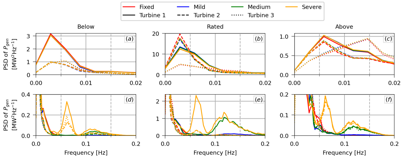
Figure 12. PSD of the generator power of each turbine in the array for low shear, TI = 5%, and for the three different mean wind speeds. The first row (a-ca-c) corresponds to the low frequencies that are excited by the turbulent wind, while the second row (d-fd-f) corresponds to the frequencies that are excited by the waves.
