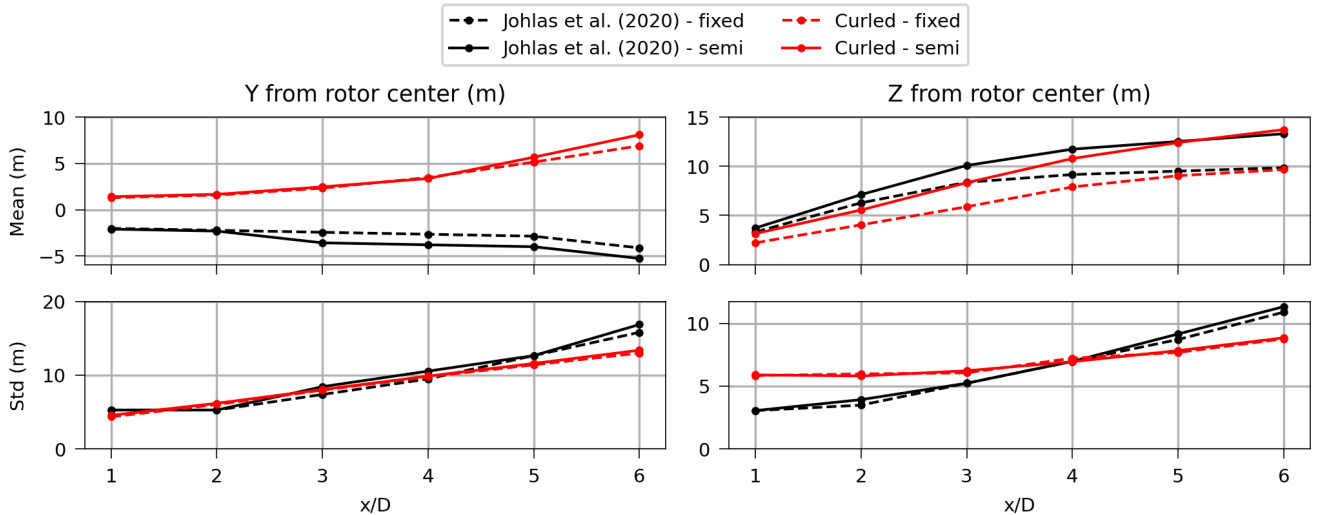
Figure 8. (a) Mean horizontal wake deflection, (b) mean vertical wake deflection, (c) horizontal wake meandering (expressed in terms of standard deviation of the wake center), and (d) vertical wake meandering as a function of downstream distance obtained with FAST.Farm (adopting the curled wake model) compared with LES results from Johlas et al. (2020) for the floating and fixed cases.
