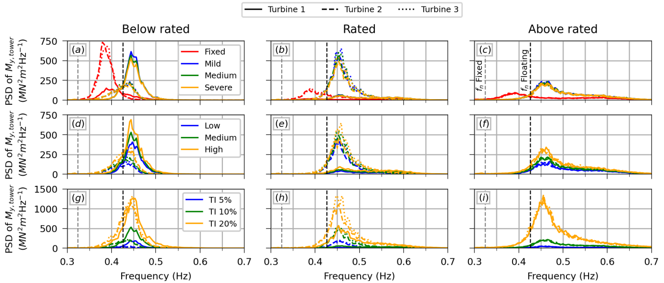
Figure 19. PSD of the fore-aft tower-base moment at the 3P frequency range for the three different mean wind speeds. (a–c) Different sea conditions for TI 10% and medium shear. (d–f) Different shear conditions for the severe sea state and TI 10%. (g–i) Different TI conditions for the severe sea state and medium shear.
