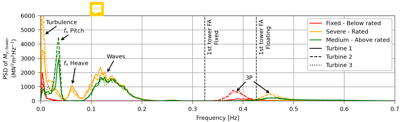
Figure 15. PSD of the fore-aft tower-base moment illustrating the distinct frequencies of interest. The examples in the figure consider TI 10% and medium shear
