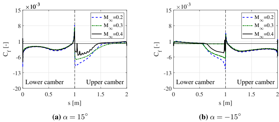
Figure 12. Instantaneous skin friction coefficient distribution at Re = 9 \times 10^6 , for the two different incidences, and varying inflow Mach number. The black dotted line corresponds to the leading edge
