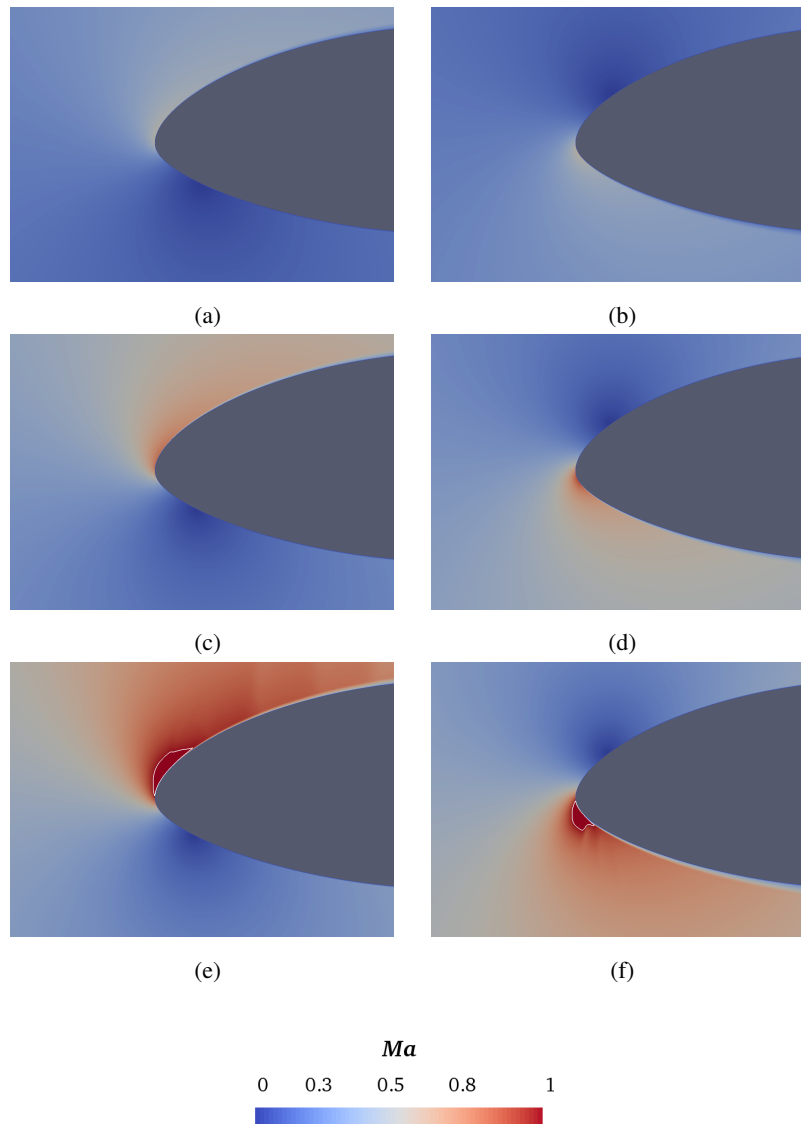
Figure 5. Instantaneous contour maps of local Mach number at Re = 1.8 \times 10^6 , for varying free-stream velocity: M_\infty = 0.2 (top), M_\infty = 0.3 (middle), and M_\infty = 0.4 (bottom). Two different incidences are considered: \alpha = 15^\circ (left column) and \alpha = -15^\circ (right column). The iso-line corresponding to Ma = 0.99 is depicted.
