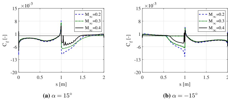
Figure 12. Instantaneous skin friction coefficient distribution at Re = 9 \times 10^6 , for the two different incidences, and varying inflow Mach number
