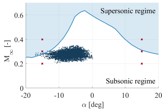
Figure 1. Operational conditions of the IEA-15MW RWT at 97% of the blade radius (De Tavernier and von Terzi , 2022). The red crosses represent some of the particular cases considered here
