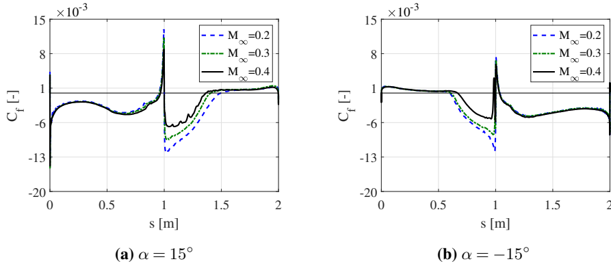
Figure 11. Instantaneous skin friction coefficient distribution at Re = 1.8 \times 10^6 , for the two different incidences, and varying inflow Mach number
