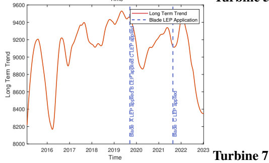
Figure A1. Overlay of blade maintenance activities on long-term Turbine Performance Integral (TPI) trends. Performance increases with higher TPI values. Vertical dashed lines indicate: Blade Leading Edge Protection (LEP) application. The solid line represents the long-term TPI trend.
