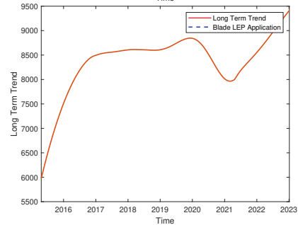
Figure A2. Overlay of blade maintenance activities on long-term Turbine Performance Integral (TPI) trends. Performance increases with higher TPI values. Vertical dashed lines indicate: Blade Leading Edge Protection (LEP) application. The solid line represents the long-term TPI trend.
