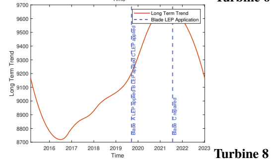
Figure A1. Overlay of blade maintenance activities on long-term Turbine Performance Integral (TPI) trends. Performance increases with higher TPI values. Vertical dashed lines indicate: Blade Leading Edge Protection (LEP) application. The solid line represents the long-term TPI trend.
