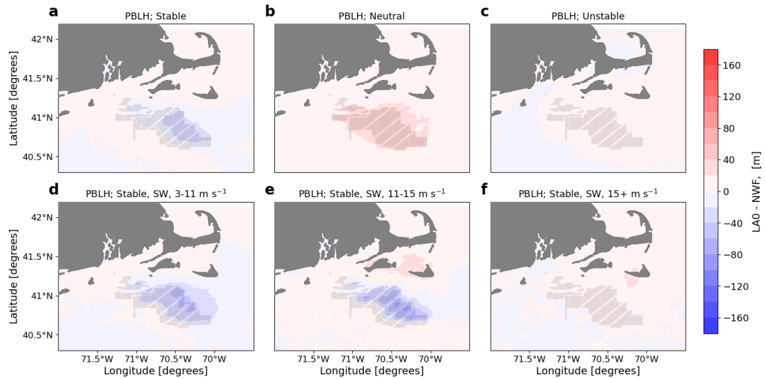
Figure 22. Mean PBLH difference between the LA0 and NWF simulations in (a) stable conditions, (b) neutral conditions, (c) unstable conditions, (d) 3-11 \text{ m s}^{-1} , (e) 11-15 \text{ m s}^{-1} , and (f) 15+ \text{ m s}^{-1} . Panels d, e, and f are only during times with stable conditions and southwest winds. Turbines are marked in gray.
