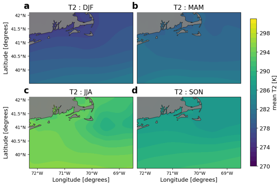
Figure A4. Same as in Fig. 5, but for SST2 m temperature .
