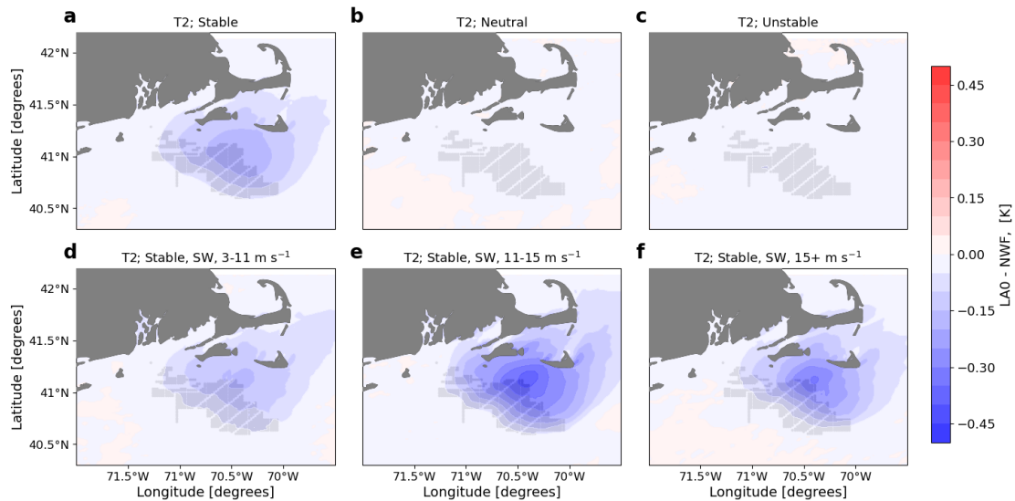
Figure 18. Mean 2 m temperature difference between the LA0 and NWF simulations in (a) stable conditions, (b) neutral conditions, (c) unstable conditions, (d) 3-11 \text{ m s}^{-1} , (e) 11-15 \text{ m s}^{-1} , and (f) 15+ \text{ m s}^{-1} . Panels d, e, and f are only during times with stable conditions and southwest winds. Turbines are marked in gray.
