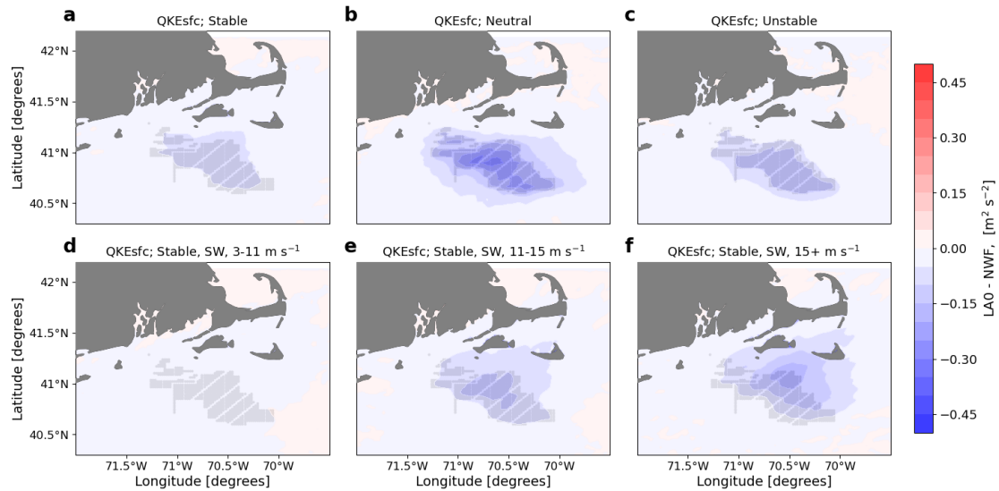
Figure 16. Mean surface TKE difference between the LA0 and NWF simulations in (a) stable conditions, (b) neutral conditions, (c) unstable conditions, (d) 3-11 m s -1 , (e) 11-15 m s -1 , and (f) 15+ m s -1 . Panels d, e, and f are only during times with stable conditions and southwest winds. Turbines are marked in gray.
