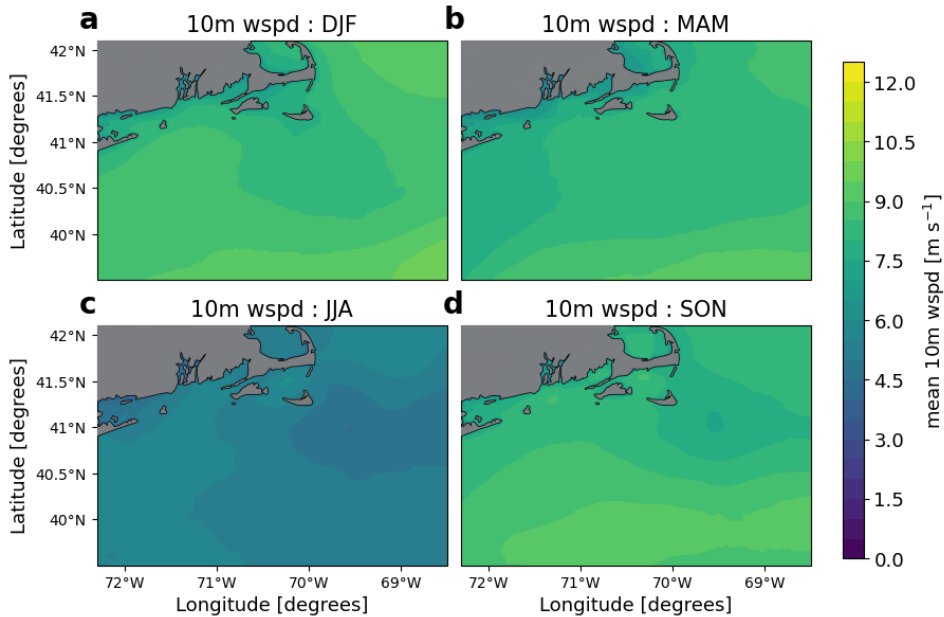
Figure A2. Same as in Fig. 5, but for 10 m wind speed
