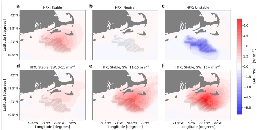
Figure 20. Mean heat flux difference between the LA0 and NWF simulations in (a) stable conditions, (b) neutral conditions, (c) unstable conditions, (d) 3-11 \text{m s}^{-1} , (e) 11-15 \text{m s}^{-1} , and (f) 15+ \text{m s}^{-1} . Panels d, e, and f are only during times with stable conditions and southwest winds. Turbines are marked in gray.
