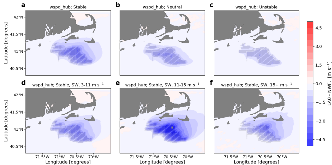
Figure 10. Mean hub-height wind speed difference between the LA0 and NWF simulations in (a) stable conditions, (b) neutral conditions, (c) unstable conditions, (d) 3-11 m s -1 , (e) 11-15 m s -1 , and (f) 15+ m s -1 . Panels d, e, and f are only during times with stable conditions and southwest winds. Turbines are marked in gray.
