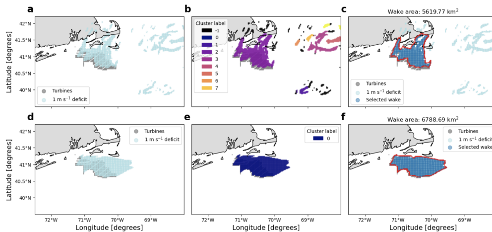
Figure 7. Example of the three steps taken to identify the wind plant wake on 14 December 2019 at 22:00 UTC (a, b, and c) and on 04 February 2020 at 07:00 UTC (d, e, and f) in the LA100 simulations . Turbines are marked in gray. (a and d) All points identified with a 1 \text{ m s}^{-1} deficit are marked in light blue. (b and e) The points with a wind speed deficit are clustered, and a label is assigned to each cluster by the DBSCAN algorithm. The -1 label indicates points classified as noise. (c and f) The selected wind plant wake is in darker blue, with its wake boundary in red.
