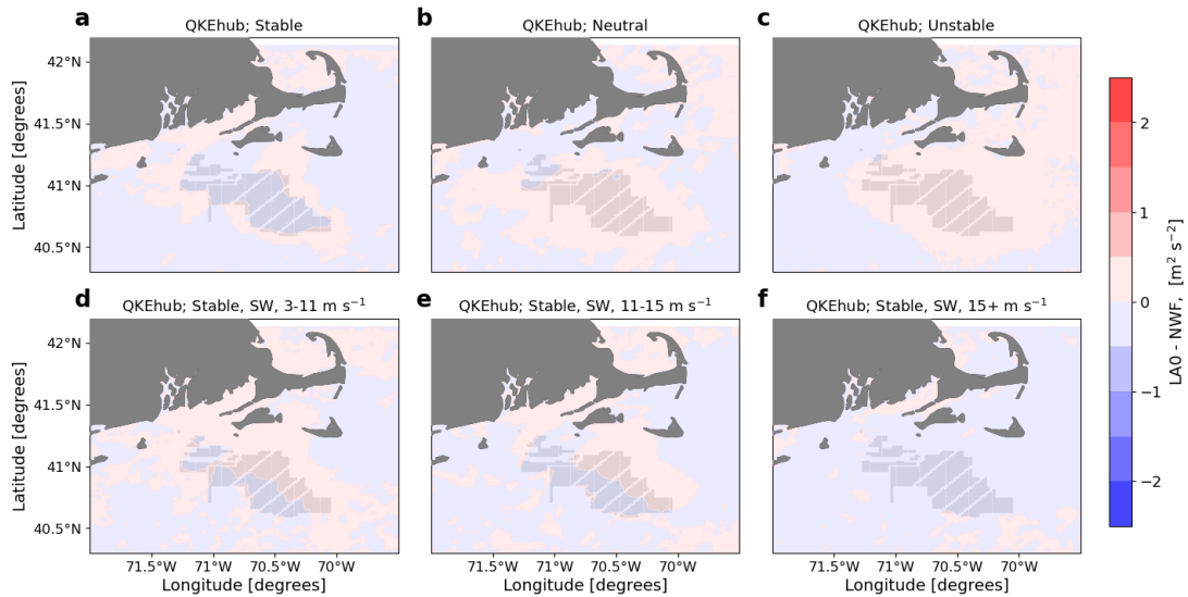
Figure 14. Mean hub-height TKE difference between the LA0 and NWF simulations in (a) stable conditions, (b) neutral conditions, (c) unstable conditions, (d) 3-11 m s -1 , (e) 11-15 m s -1 , and (f) 15+ m s -1 . Panels d, e, and f are only during times with stable conditions and southwest winds. Turbines are marked in gray.
