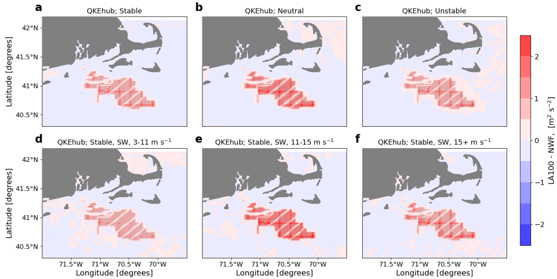
Figure 13. Mean hub-height TKE difference between the LA100 and NWF simulations in (a) stable conditions, (b) neutral conditions, (c) unstable conditions, (d) 3-11 m s -1 , (e) 11-15 m s -1 , and (f) 15+ m s -1 . Panels d, e, and f are only during times with stable conditions and southwest winds. Turbines are marked in gray.
