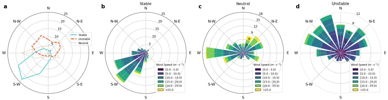
Figure 6. (a) The frequency of each 22.5-degree wind direction bin for each stability classification. Wind roses for stable, neutral, and unstable conditions are shown in Panels panels b, c, and d, respectively. In all panels, radial distance from the center refers to the percentage of values in each 22.5 degree bin.
