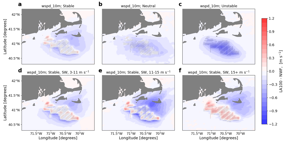
Figure 11. Mean 10 m wind speed difference between the LA100 and NWF simulations in (a) stable conditions, (b) neutral conditions, (c) unstable conditions, (d) 3-11 m s -1 , (e) 11-15 m s -1 , and (f) 15+ m s -1 . Panels d, e, and f are only during times with stable conditions and southwest winds. Turbines are marked in gray.
