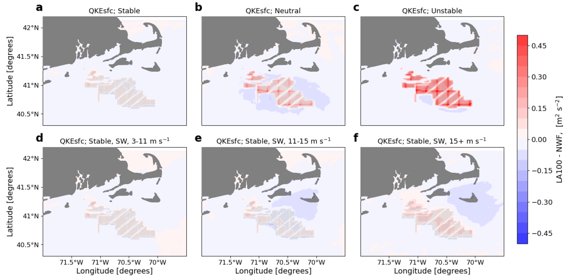
Figure 15. Mean surface TKE difference between the LA100 and NWF simulations in (a) stable conditions, (b) neutral conditions, (c) unstable conditions, (d) 3-11 m s -1 , (e) 11-15 m s -1 , and (f) 15+ m s -1 . Panels d, e, and f are only during times with stable conditions and southwest winds. Turbines are marked in gray.
