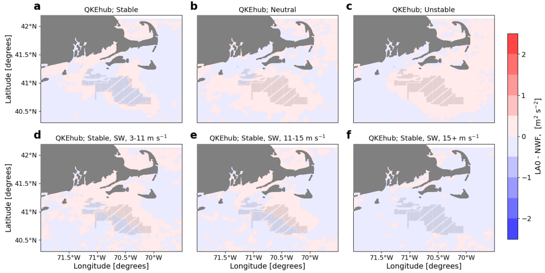
Figure 14. Mean hub-height QKE difference between the LA0 and NWF simulations in (a) stable conditions, (b) neutral conditions, (c) unstable conditions, (d) 3-11 \text{m s}^{-1} , (e) 11-15 \text{m s}^{-1} , and (f) 15+ \text{m s}^{-1} . Panels d, e, and f are only during times with stable conditions and southwest winds. Turbines are marked in gray.
