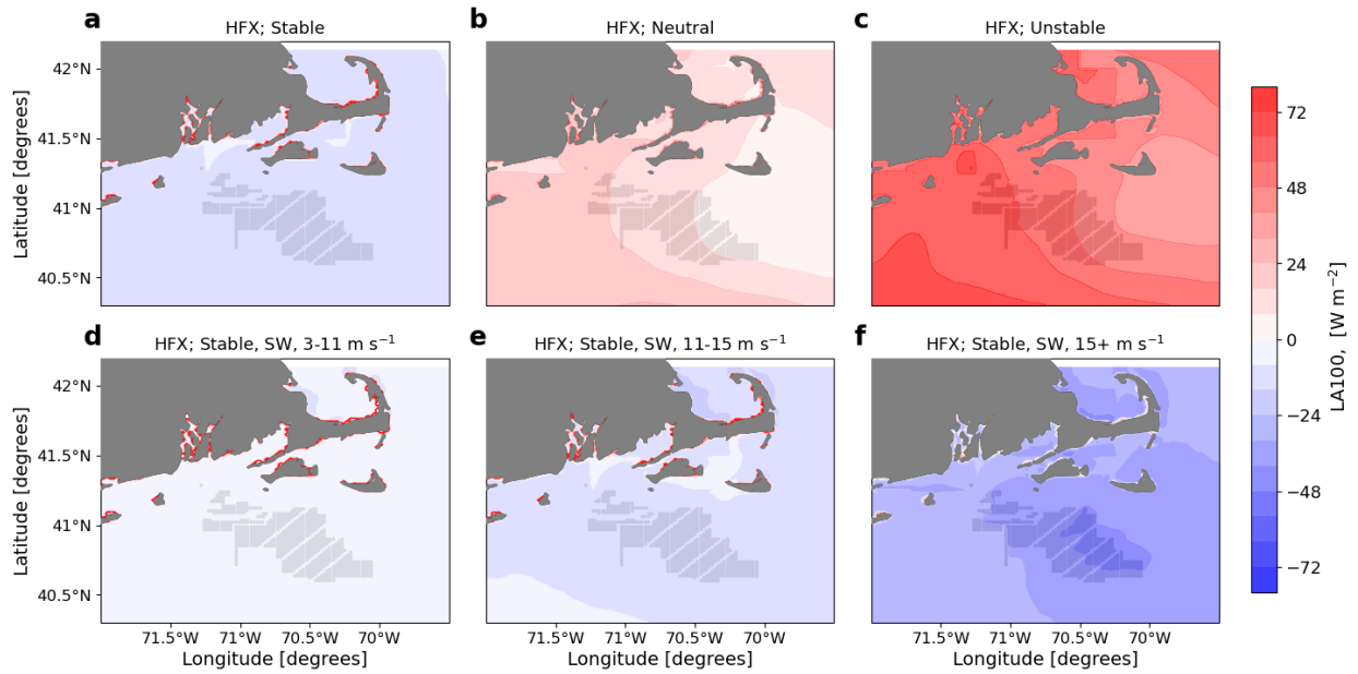
Figure C2. Mean surface heat flux for the LA100 simulation in (a) stable conditions, (b) neutral conditions, (c) unstable conditions, (d) 3-11 m s -1 , (e) 11-15 m s -1 , and (f) 15+ m s -1 . Panels d, e, and f are only during times with stable conditions and southwest winds. Turbines are marked in gray..
