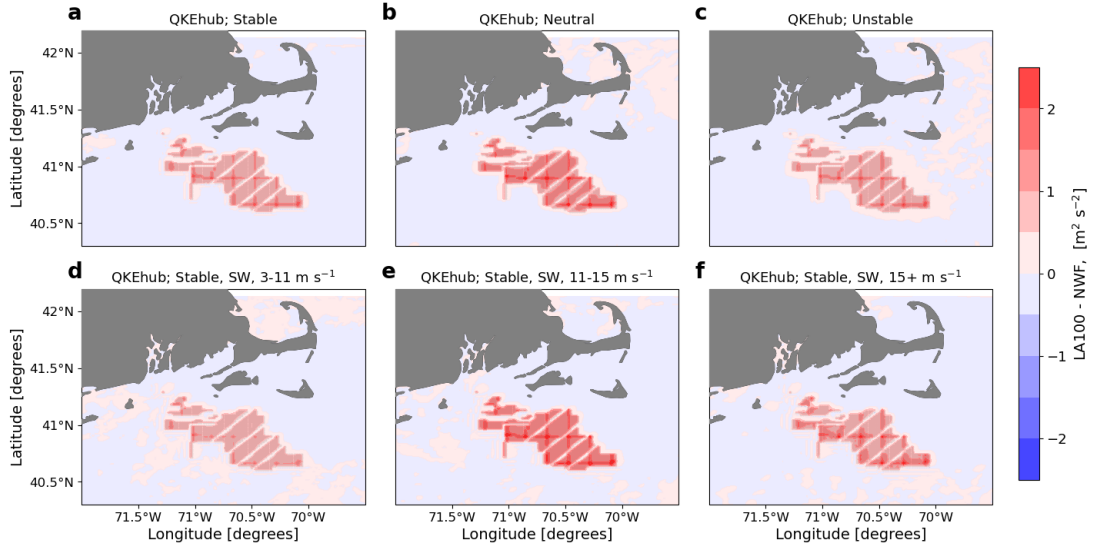
Figure 13. Mean hub-height QKE difference between the LA100 and NWF simulations in (a) stable conditions, (b) neutral conditions, (c) unstable conditions, (d) 3-11 \text{m s}^{-1} , (e) 11-15 \text{m s}^{-1} , and (f) 15+ \text{m s}^{-1} . Panels d, e, and f are only during times with stable conditions and southwest winds. Turbines are marked in gray.
