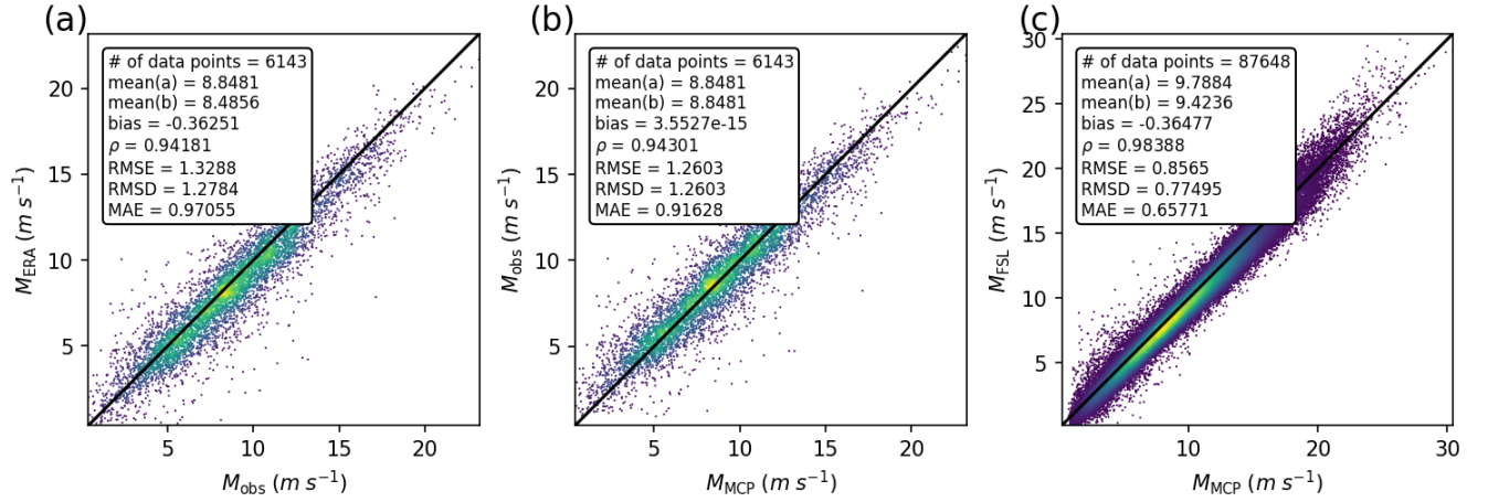
Figure 8. Illustration of MCP. a) 100 m ERA wind against 75.3 m observed wind during 2010, b) 75.3 m observed wind against MCP-corrected wind during 2010, and c) free stream LES wind against MCP-corrected wind during 2010-2019.
