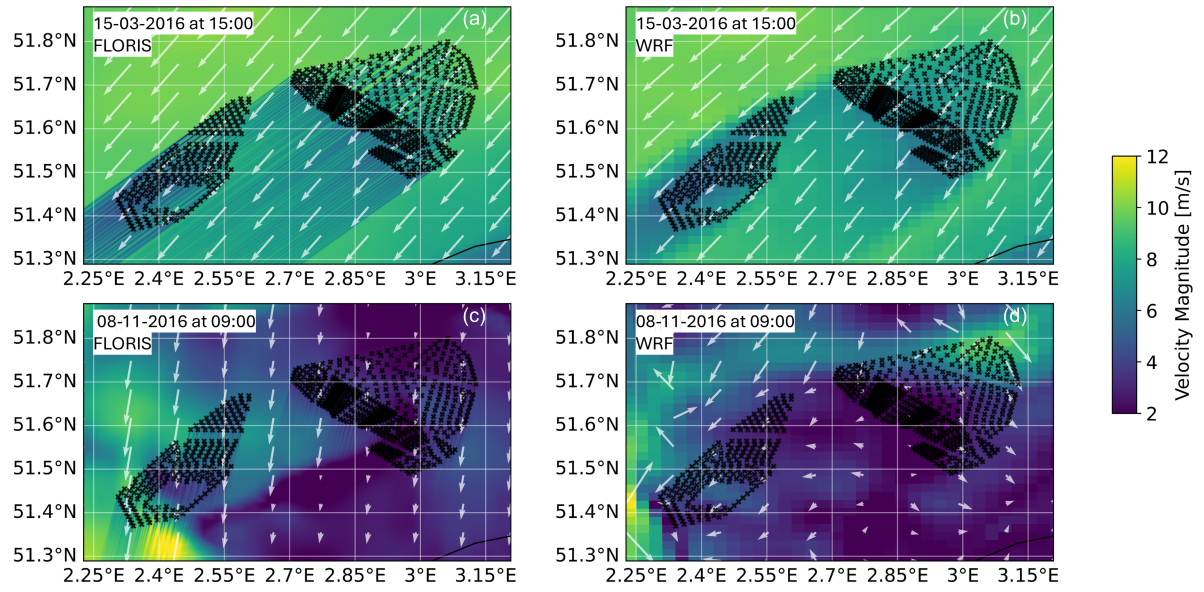
Figure 8. The velocity field for the TurboPark A=0.04 model with varying TI (a,c), and corresponding WRF velocity field (b,d) for a steady case (15-03-2016 at 15:00) (a,b), and a transient case (08-11-2016 at 09:00) (c,d).
