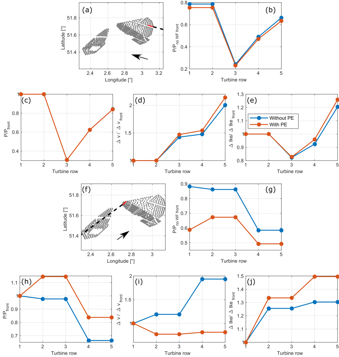
Figure 12. (a) & (f) In red are the wind turbine locations considered for a specific wind direction (depicted by the black arrow (a) 105° (f) 234°), for (a) the BE-NL wind farm cluster is not waked by the PE wind farm cluster while for (f) the BE-NL cluster is waked by the PE wind farm cluster. (b) & (g) The wind turbine power per turbine row normalized by the no WF front row turbine for unwaked (blue) and waked (orange) conditions. (c) & (h) The wind turbine power per turbine row normalized by the front row turbine for unwaked (blue) and waked (orange) conditions. (d) & (i) The wind speed deficit (compared to the noWT case) per turbine row normalized by the front row turbine for unwaked (blue) and waked (orange) conditions. (e) & (f) The added TKE (compared to the no WT case) per turbine row normalized by the front row turbine for unwaked (blue) and waked (orange) conditions.
