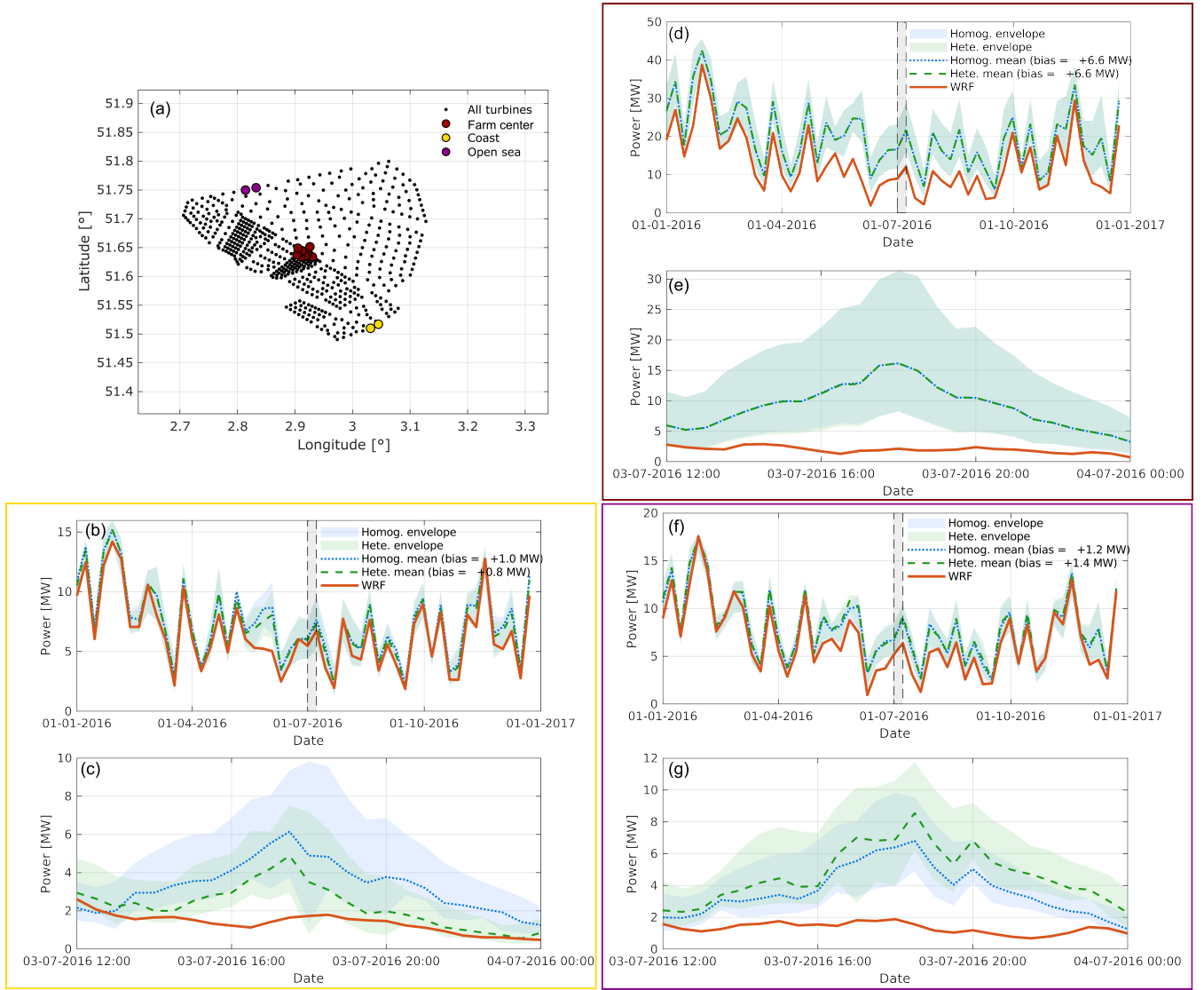
Figure C2. Grid cell power output (MW) at three representative locations within the BE-NL wind farm cluster for simulations with PE. Panel (a) shows the locations of the selected grid cells, representing the farm center, coastal, and open-sea regions. Panels (d,b,f) show weekly averages computed from 30-min data, while panels (e,c,g) show a twelve-hour zoom on 3 July 2016 at 30-min resolution. Shown are WRF (without PE) and the mean and envelope of all engineering wake models grouped by homogeneous and heterogeneous setups. The dashed box indicates the zoomed period within the full time series. Bias is defined as the engineering wake model power minus WRF power.
