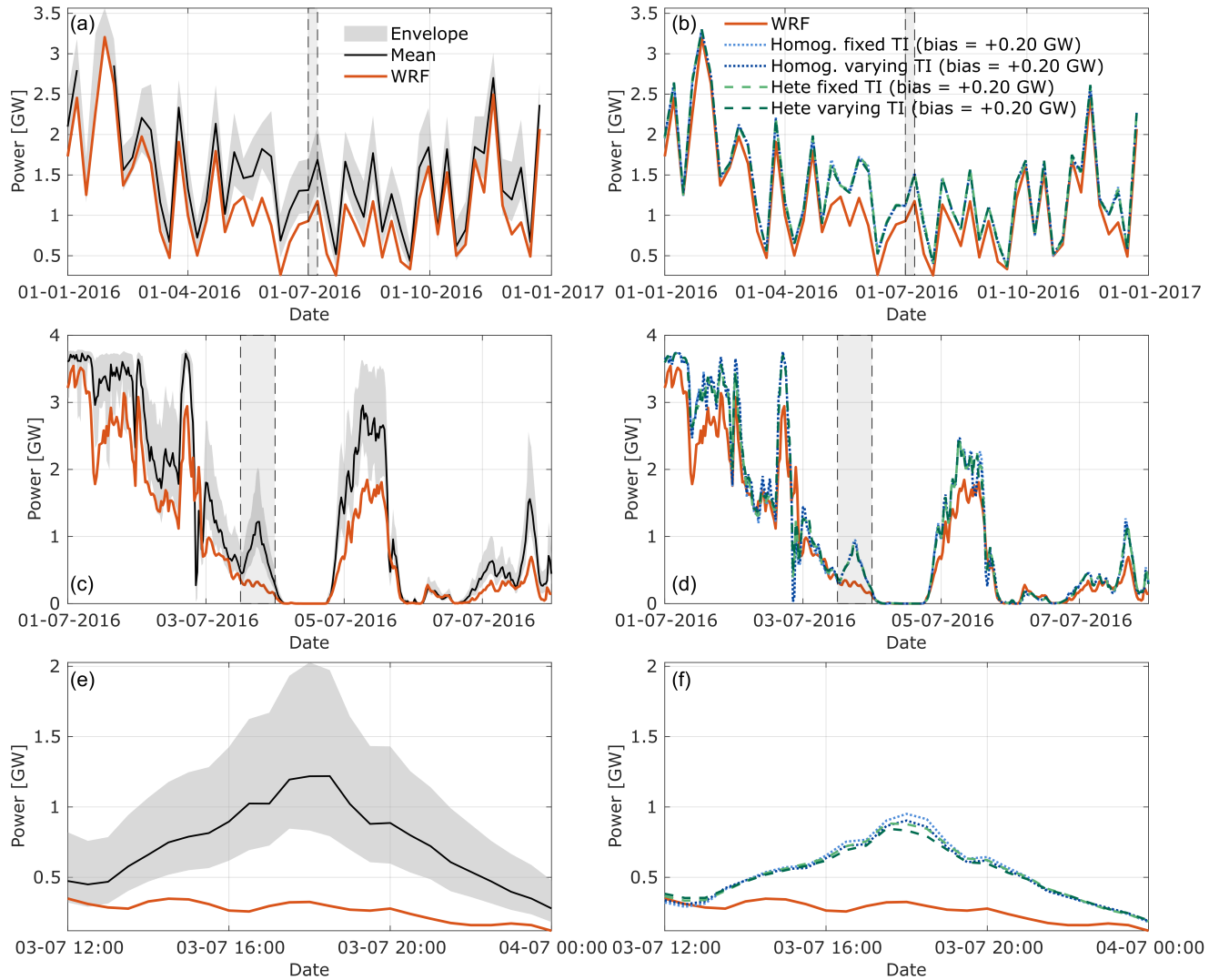
Figure C1. Total wind farm power (GW) for the BE–NL offshore wind farm cluster for simulations with PE. Shown are WRF (without PE), and the mean and envelope of all engineering models (a,c,e), and the different configurations of Turbopark with induction factor A=0.04 (b,d,f). The top row (a,b) shows weekly averages computed from 30-min data, the middle row (c,d) shows a one-week zoom (1–7 July 2016) at 30 min resolution, and the bottom row (e,f) shows a twelve-hour zoom (3 July 2016) also at 30 min resolution. The dashed box shows the time period zoom within the longer time series.
