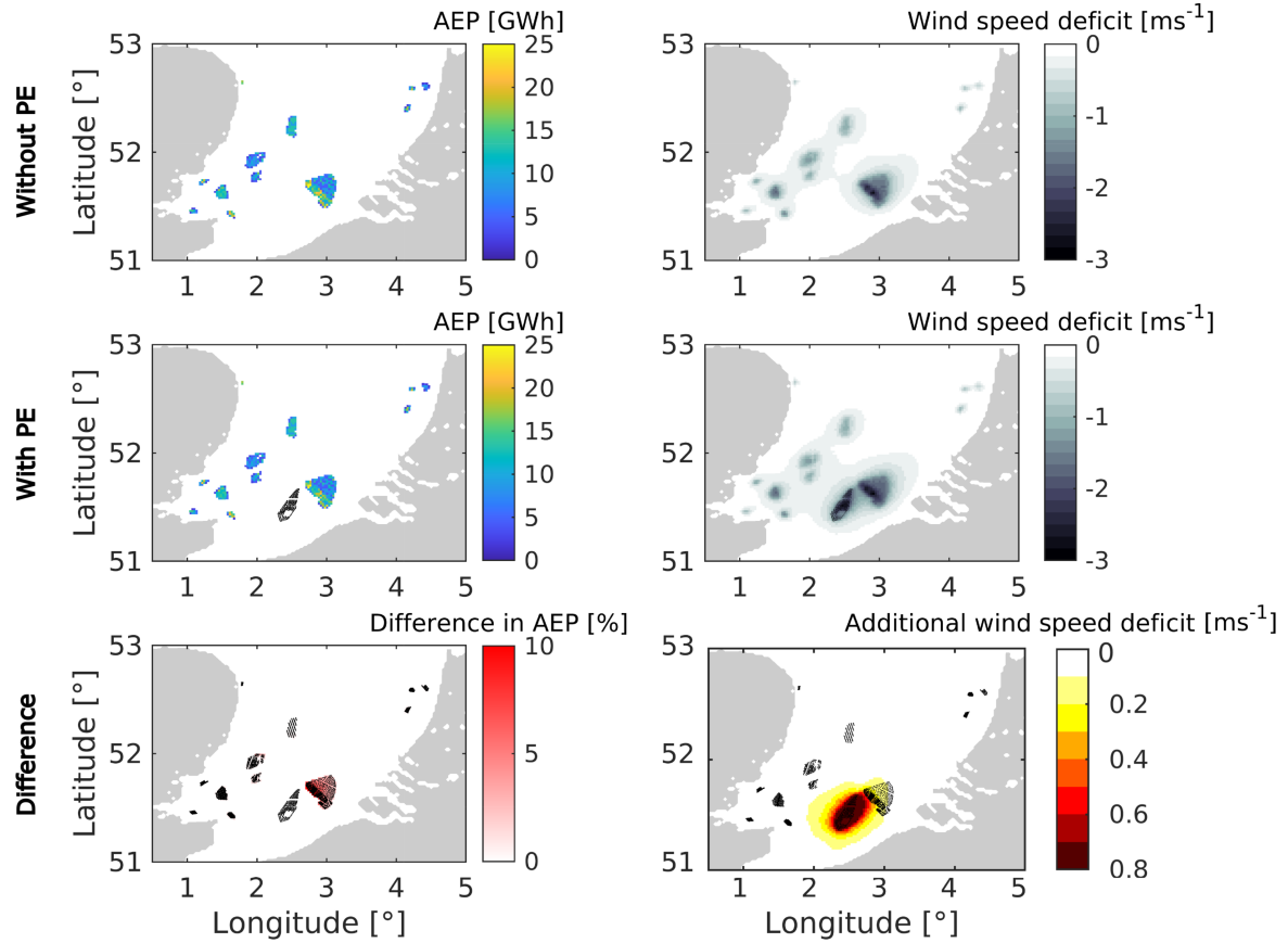
Figure 3. Annual energy production (left column) and temporally averaged wind speed deficit (right column) before (top row) and after (middle row) the construction of the PE wind farm cluster. The bottom row shows the difference between the two.
