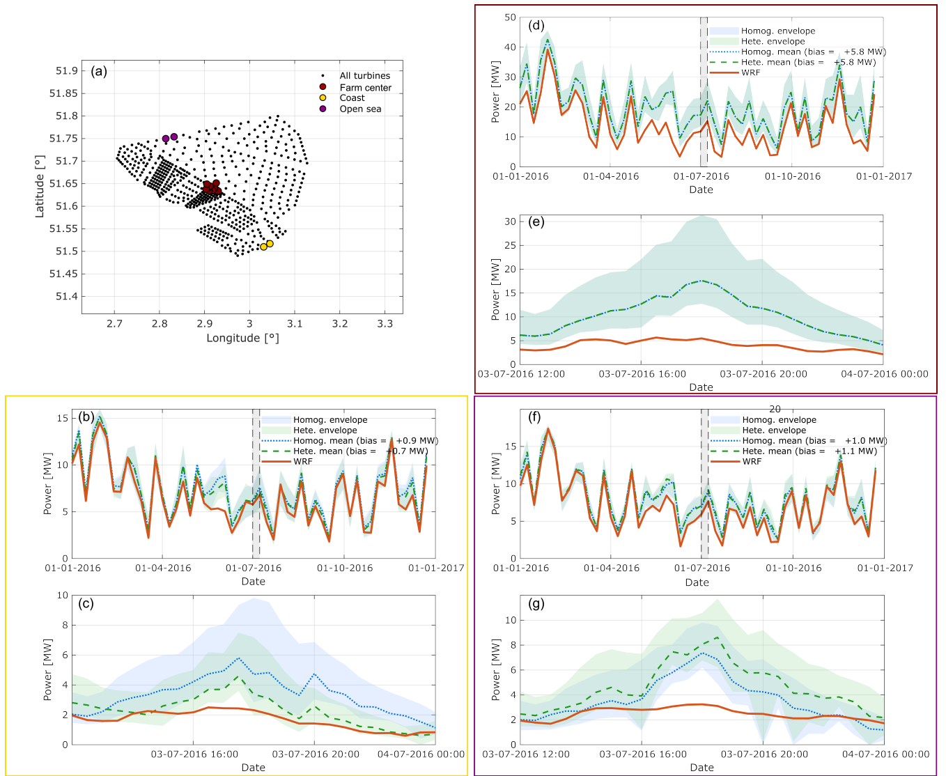
Figure 3. Grid cell power output (MW) at three representative locations within the BE-NL wind farm cluster for simulations without PE. Panel (a) shows the locations of the selected grid cells, representing the farm center, coastal, and open-sea regions. Panels (d,b,f) show weekly averages computed from 30-min data, while panels (e,c,g) show a twelve-hour zoom on 3 July 2016 at 30-min resolution. Shown are WRF (without PE) and the mean and envelope of all engineering wake models grouped by homogeneous and heterogeneous setups. The dashed box indicates the zoomed period within the full time series. Bias is defined as the engineering wake model power minus WRF power.
