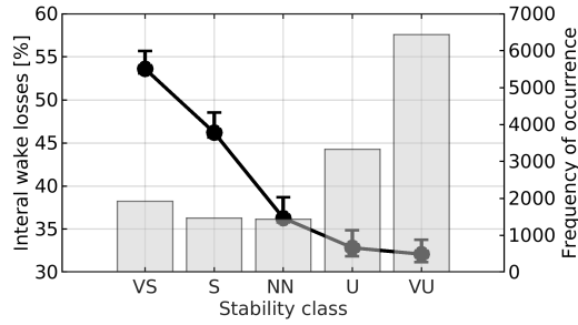
Figure 10. (Line) Spatiotemporal conditional average of internal wake energy losses as a function of atmospheric stability classes (VS: Very Stable, S: Stable, NN: Near Neutral, U: Unstable, VU: Very Unstable) only including wind speeds between 10 and 15 ms^{-1} , (bars) frequency of occurrence for the different atmospheric stability classes. The error bars represent a 95% confidence interval obtained via bootstrapping with 1000 resamples.
