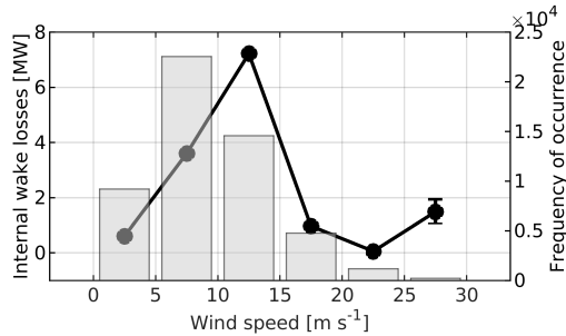
Figure 11. (Line) Spatiotemporal conditional average of absolute internal wake energy losses as a function of wind speed, (bars) frequency of occurrence for the different wind speed bins. The error bars represent a 95% confidence interval obtained via bootstrapping with 1000 resamples.
