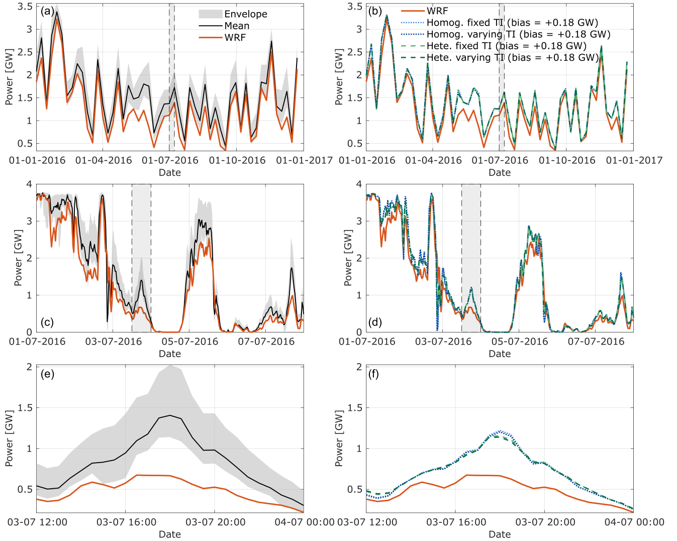
Figure 2. Total power (GW) for the BE–NL offshore wind farm cluster for simulations without PE. Shown are WRF (without PE), and the mean and envelope of all engineering models (a,c,e), and the different configurations of Turbopark with induction factor A=0.04 (b,d,f). The top row (a,b) shows weekly averages computed from 30-min data, the middle row (c,d) shows a one-week zoom (1–7 July 2016) at 30 min resolution, and the bottom row (e,f) shows a twelve-hour zoom (3 July 2016) also at 30 min resolution. The dashed box shows the time period zoom within the longer time series. The bias is calculated as the engineering wake model minus WRF.
