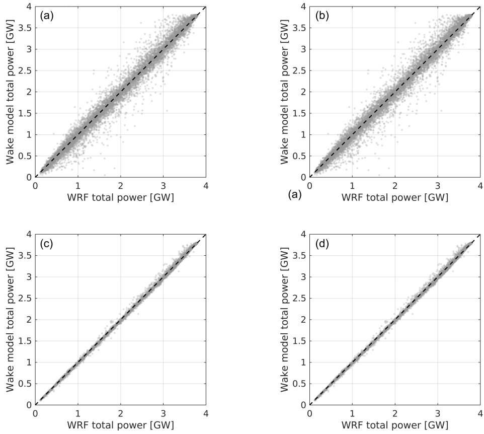
Figure A1. Total BE–NL wind farm cluster power for the no WF simulation compared between WRF and the four engineering wake model setups (a) homogeneous with fixed TI (slope=1.001, R^2 = 0.990 ), (b) homogeneous with varying TI (slope=1.001, R^2 = 0.990 ), (c) heterogeneous with fixed TI (slope=1.000, R^2 = 0.998 ), and (d) heterogeneous with varying TI (slope=1.000, R^2 = 0.998 ). The dashed line represents the 1:1 line.
