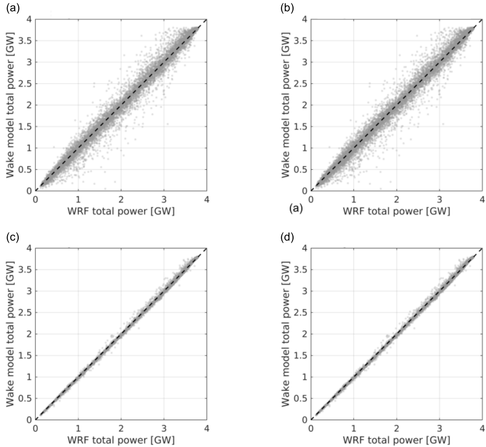
Figure B1. Total BE–NL wind farm cluster power for the no WF simulation compared between WRF and the four engineering wake model setups (a) homogeneous with fixed TI (slope=1.001, R^2 = 0.990 ), (b) homogeneous with varying TI (slope=1.001, R^2 = 0.990 ), (c) heterogeneous with fixed TI (slope=1.000, R^2 = 0.998 ), and (d) heterogeneous with varying TI (slope=1.000, R^2 = 0.998 ). The dashed line represents the 1:1 line.
