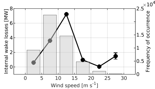
Figure 11. (Line) Spatiotemporal conditional average of absolute internal wake energy losses as a function of wind speed, (bars) frequency of occurrence for the different wind speed bins. The error bars represent a 95% confidence interval obtained via bootstrapping with 1000 resamples.
