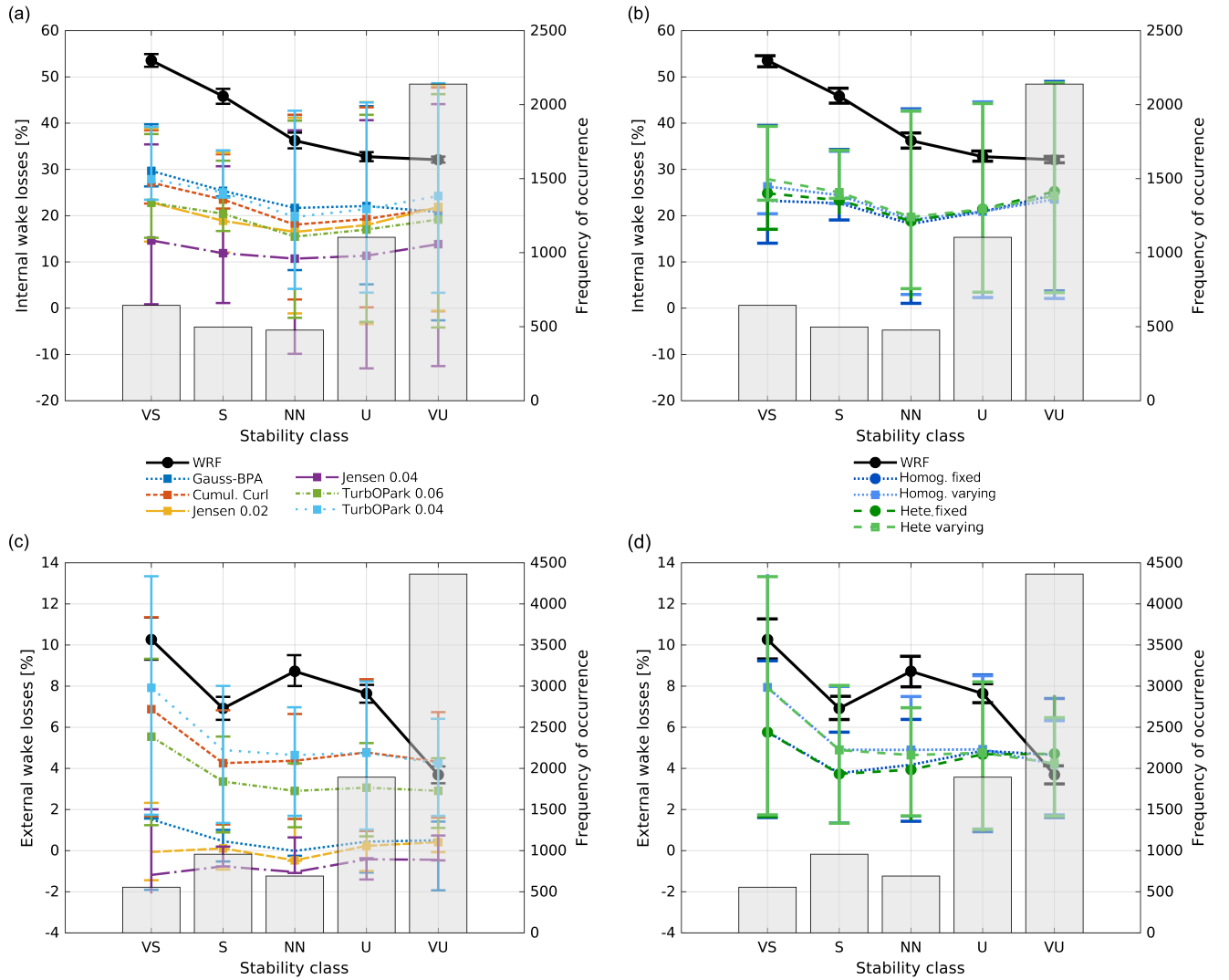
Figure 7. Spatiotemporal conditional averages of wake energy losses by atmospheric stability class (VS: very stable, S: stable, NN: near-neutral, U: unstable, VU: very unstable). (a,b) Internal wake energy losses for wind speeds between 10 and 15 ms^{-1} . (c,d) External wake energy losses for wind directions from 193° - 317°. Lines show engineering wake models for heterogeneous inflow and varying TI and WRF; (a,c) all models, (b,d) TurbOPark ( A = 0.04 ) for all inflow setups and WRF. Bars indicate the frequency of occurrence of each stability class. The error bars represent a 95% confidence interval obtained via bootstrapping with 1000 resamples.
