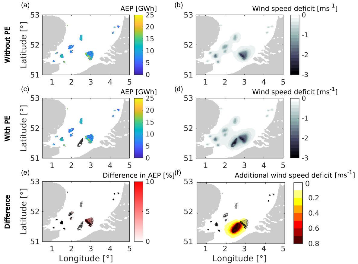
Figure 3. Annual energy production (a,c,e) and temporally averaged wind speed deficit (b,d,f) before (a,b) and after (c,d) the construction of the PE wind farm cluster. The bottom row shows the difference between the two (e,f).
