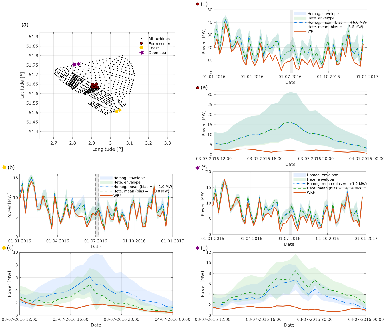
Figure D2. Grid cell power output (MW) at three representative locations within the BE-NL wind farm cluster for simulations with PE . Panel (a) shows the locations of the selected grid cells, representing the farm center, coastal, and open-sea regions. Panels (d,b,f) show weekly averages computed from 30-min data, while panels (e,c,g) show a twelve-hour zoom on 3 July 2016 at 30-min resolution. Shown are WRF ( without PE ) and the mean and envelope of all engineering wake models grouped by homogeneous and heterogeneous setups. The dashed box indicates the zoomed period within the full time series. Bias is defined as the engineering wake model power minus WRF power.
