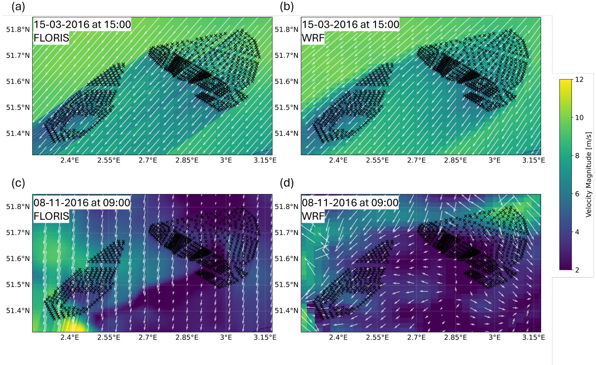
Figure 8. The velocity field for the TurbOPark A=0.04 model with varying TI (a,c), and corresponding WRF velocity field (b,d) for a steady case (15-03-2016 at 15:00) (a,b), and a transient case (08-11-2016 at 09:00) (c,d). Arrows indicate wind vectors and are shown using the same scale in all panels.
