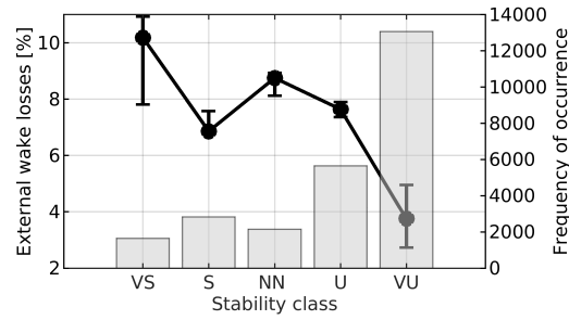
Figure 6. (Line) Spatiotemporal conditional average of external wake energy losses as a function of atmospheric stability classes (VS: Very Stable, S: Stable, NN: Near Neutral, U: Unstable, VU: Very Unstable) only including wind directions from 193^\circ - 317^\circ , (bars) frequency of occurrence for the different atmospheric stability classes. The error bars represent a 95% confidence interval obtained via bootstrapping with 1000 resamples.
