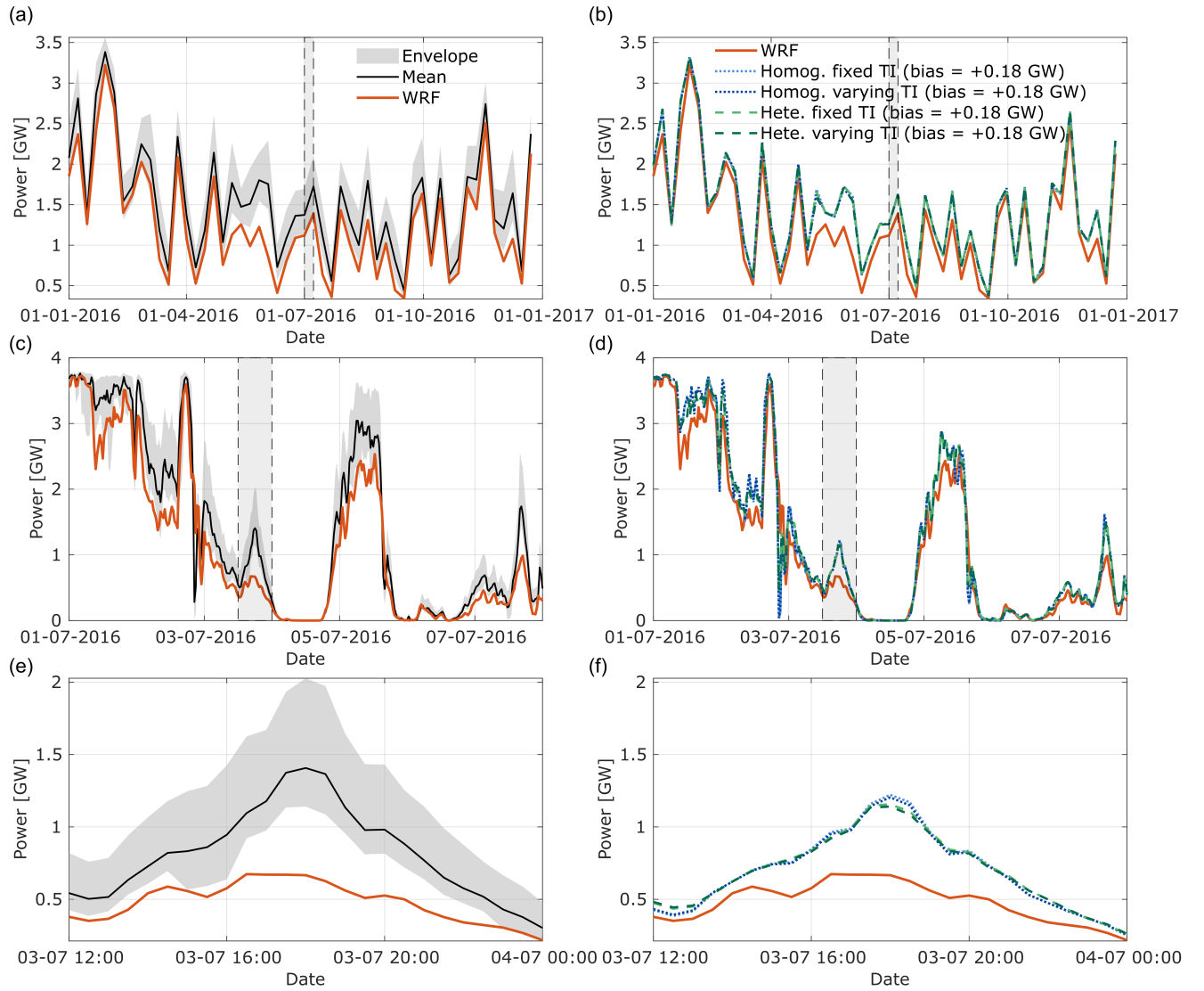
Figure 2. Total power (GW) for the BE–NL offshore wind farm cluster for simulations without PE . Shown are WRF, and the mean and envelope of all engineering models (a,c,e), and the different configurations of TurbOPark with induction factor A=0.04 (b,d,f). The top row (a,b) shows weekly averages computed from 30-min data, the middle row (c,d) shows a one-week zoom (1–7 July 2016) at 30 min resolution, and the bottom row (e,f) shows a twelve-hour zoom (3 July 2016) also at 30 min resolution. The zoom periods were selected to show periods with the largest differences between WRF and the engineering wake models. The zoom periods were selected to show periods with the largest differences between WRF and the engineering wake models. The dashed box shows the time period zoom within the longer time series. The bias is calculated as the engineering wake model minus WRF.
