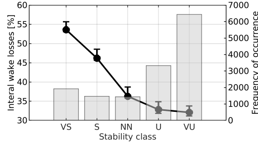
Figure 10. (Line) Spatiotemporal conditional average of internal wake energy losses as a function of atmospheric stability classes (VS: Very Stable, S: Stable, NN: Near Neutral, U: Unstable, VU: Very Unstable) only including wind speeds between 10 and 15 \text{ms}^{-1} , (bars) frequency of occurrence for the different atmospheric stability classes. The error bars represent a 95% confidence interval obtained via bootstrapping with 1000 resamples.
