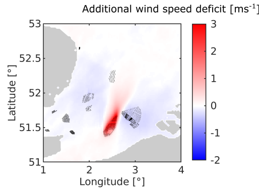
Figure 8. External BE–NL wind farm wake deficit for wind directions between 180^\circ and 210^\circ , the sector showing negative external wake losses. This map shows the additional wind speed deficit after the construction of the PE wind farm for timesteps with negative external wake energy losses over the farm.
