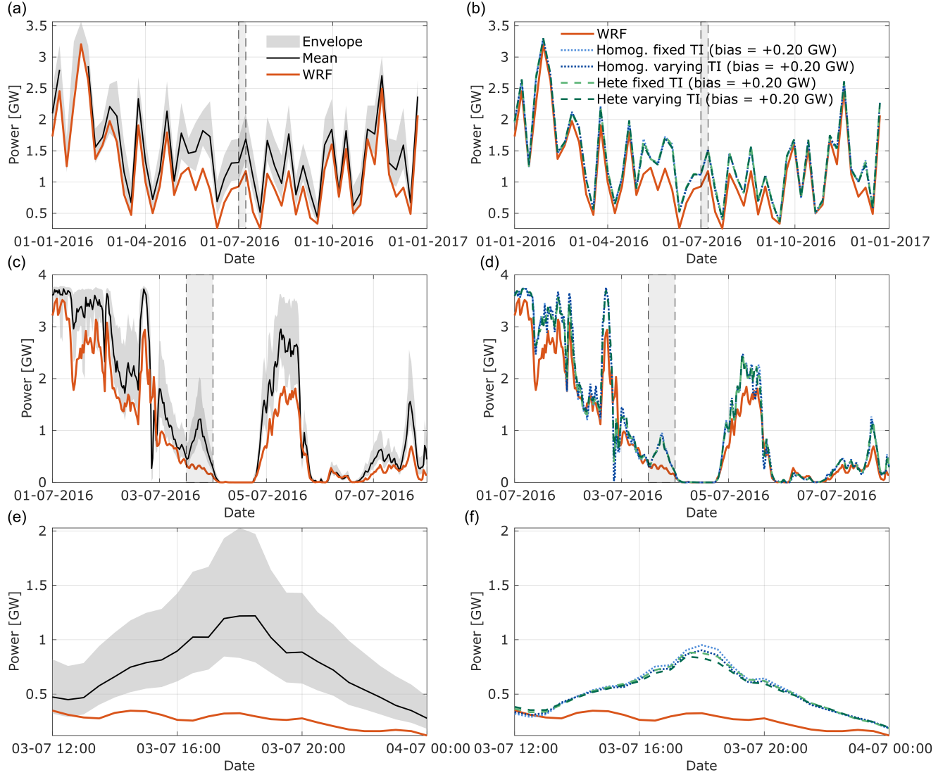
Figure D1. Total wind farm power (GW) for the BE–NL offshore wind farm cluster for simulations with PE . Shown are WRF ( without PE ), and the mean and envelope of all engineering models (a,c,e), and the different configurations of TurbOPark with induction factor A=0.04 (b,d,f). The top row (a,b) shows weekly averages computed from 30-min data, the middle row (c,d) shows a one-week zoom (1–7 July 2016) at 30 min resolution, and the bottom row (e,f) shows a twelve-hour zoom (3 July 2016) also at 30 min resolution. The dashed box shows the time period zoom within the longer time series.
