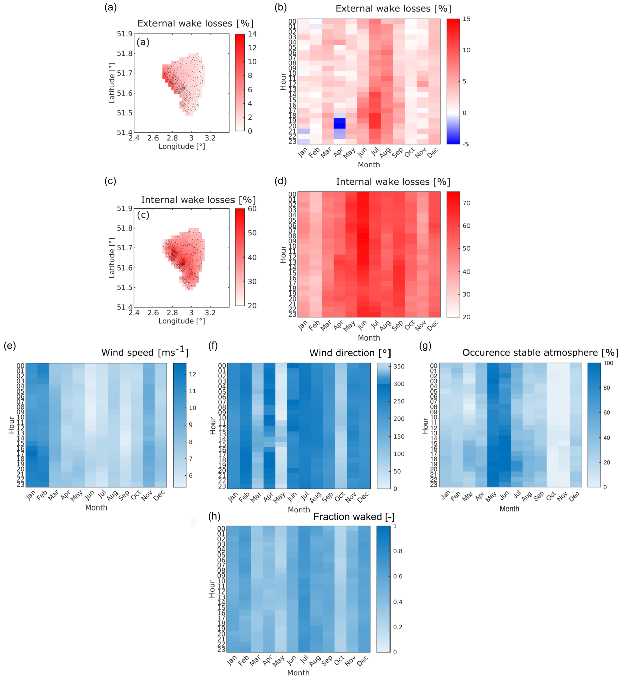
Figure 13. Results are shown for the BE-NL wind farm cluster. (a) Temporal average external wake energy losses. (b) Hourly and monthly variations of the spatiotemporally averaged external wake energy losses. (c) Yearly averaged internal wake energy losses. (d) Hourly and monthly variations of the spatiotemporally averaged internal wake energy losses. Hourly and monthly variations of (e) wind speed, (f) wind direction, (g) occurrence of stable atmospheric conditions (h) fraction of wind directions within the PE wind farm cluster wake ( 193^\circ - 317^\circ ), with 1 corresponding to waked and 0 to non waked conditions. Hourly variations are given in UTC.
