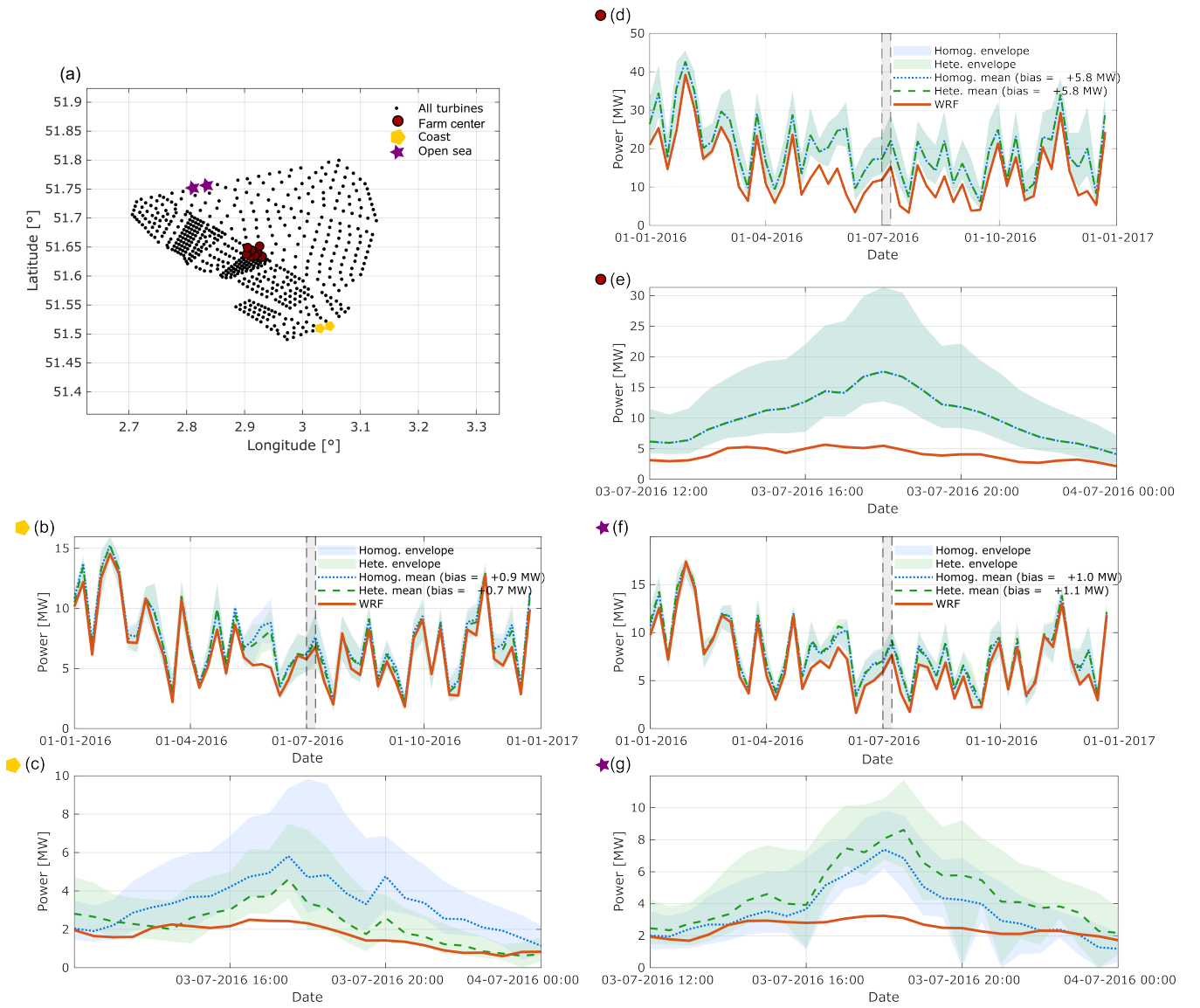
Figure 3. Grid cell power output (MW) at three representative locations within the BE-NL wind farm cluster for simulations without PE . Panel (a) shows the locations of the selected grid cells, representing the farm center (circle), coastal (pentagon), and open-sea (star) regions. Panels (d,b,f) show weekly averages computed from 30-min data, while panels (e,c,g) show a twelve-hour zoom on 3 July 2016 at 30-min resolution. Shown are WRF ( without PE ) and the mean and envelope of all engineering wake models grouped by homogeneous and heterogeneous setups. The dashed box indicates the zoomed period within the full time series. Bias is defined as the engineering wake model power minus WRF power.
